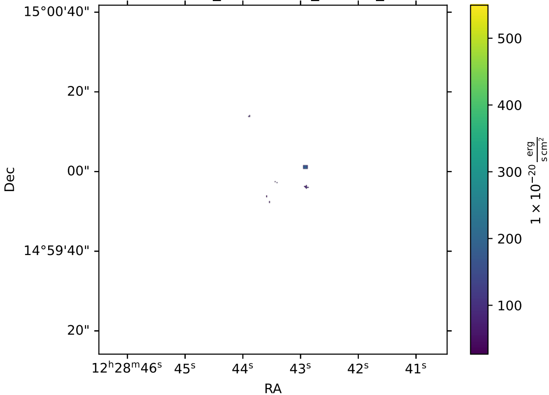
IC3392_multithresh_OI6300_I
