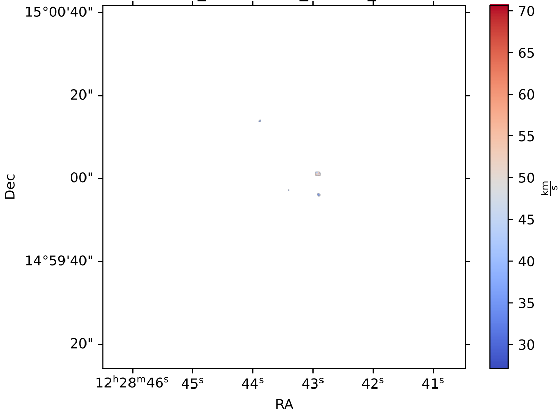
IC3392_multithresh_OI6300_SIGMA
