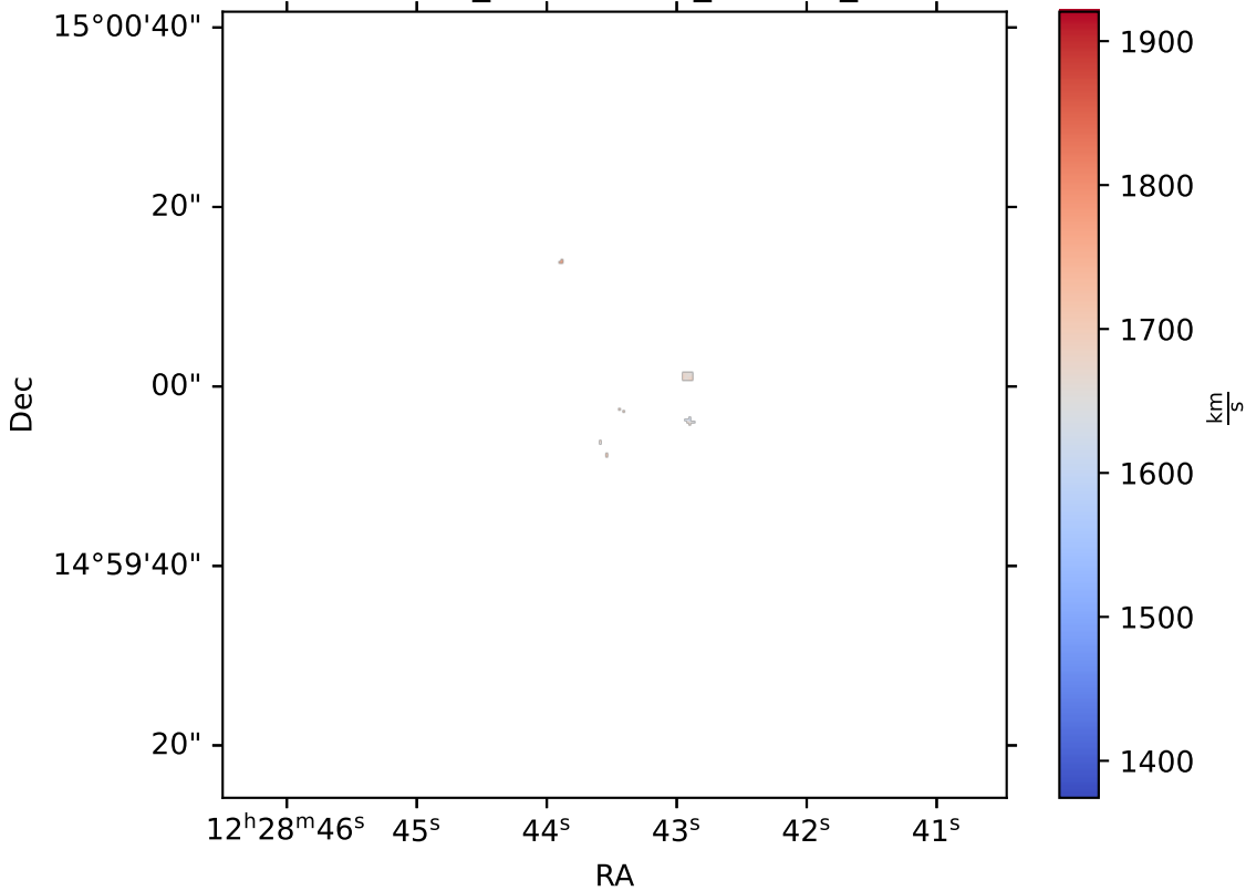
IC3392_multithresh_OI6300_V
