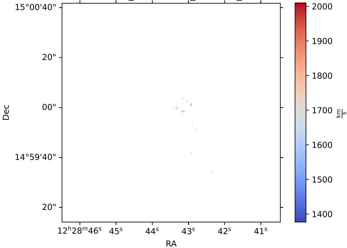
IC3392_multithresh_OIII4958_V
