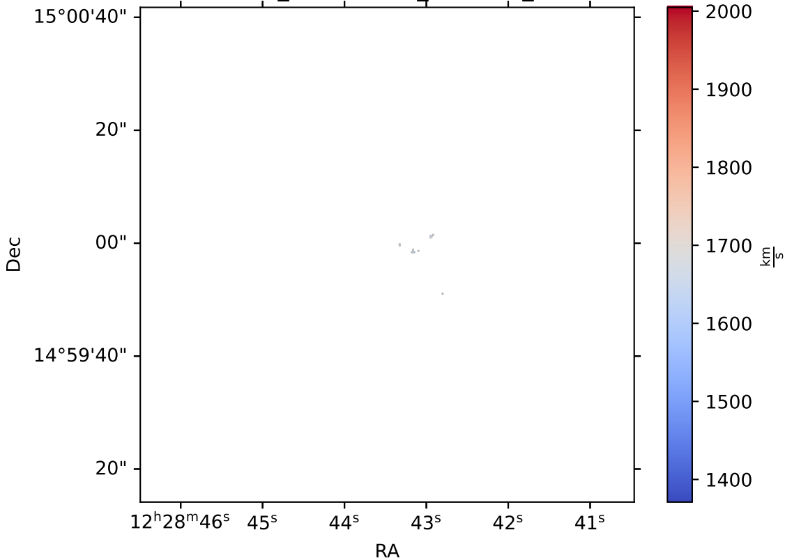
IC3392_multithresh_OIII4958_VEL
