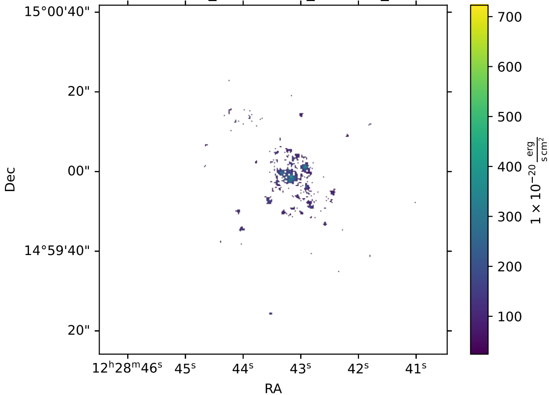
IC3392_multithresh_OIII5006_I
