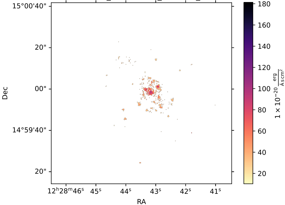
IC3392_multithresh_OIII5006_P
