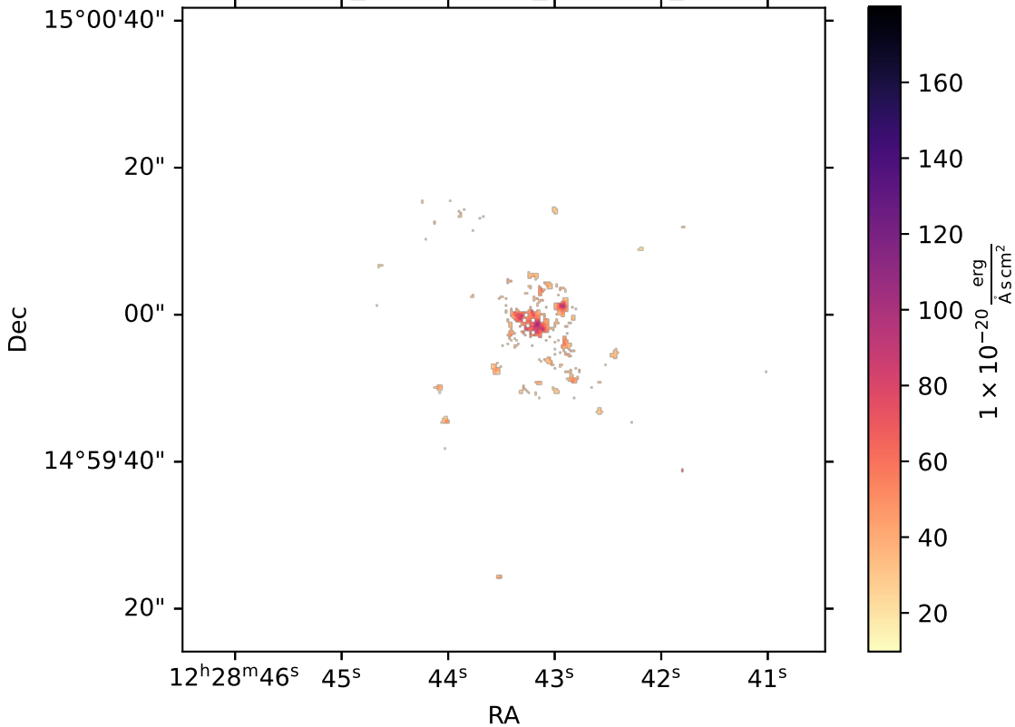
IC3392_multithresh_OIII5006_PEAK
