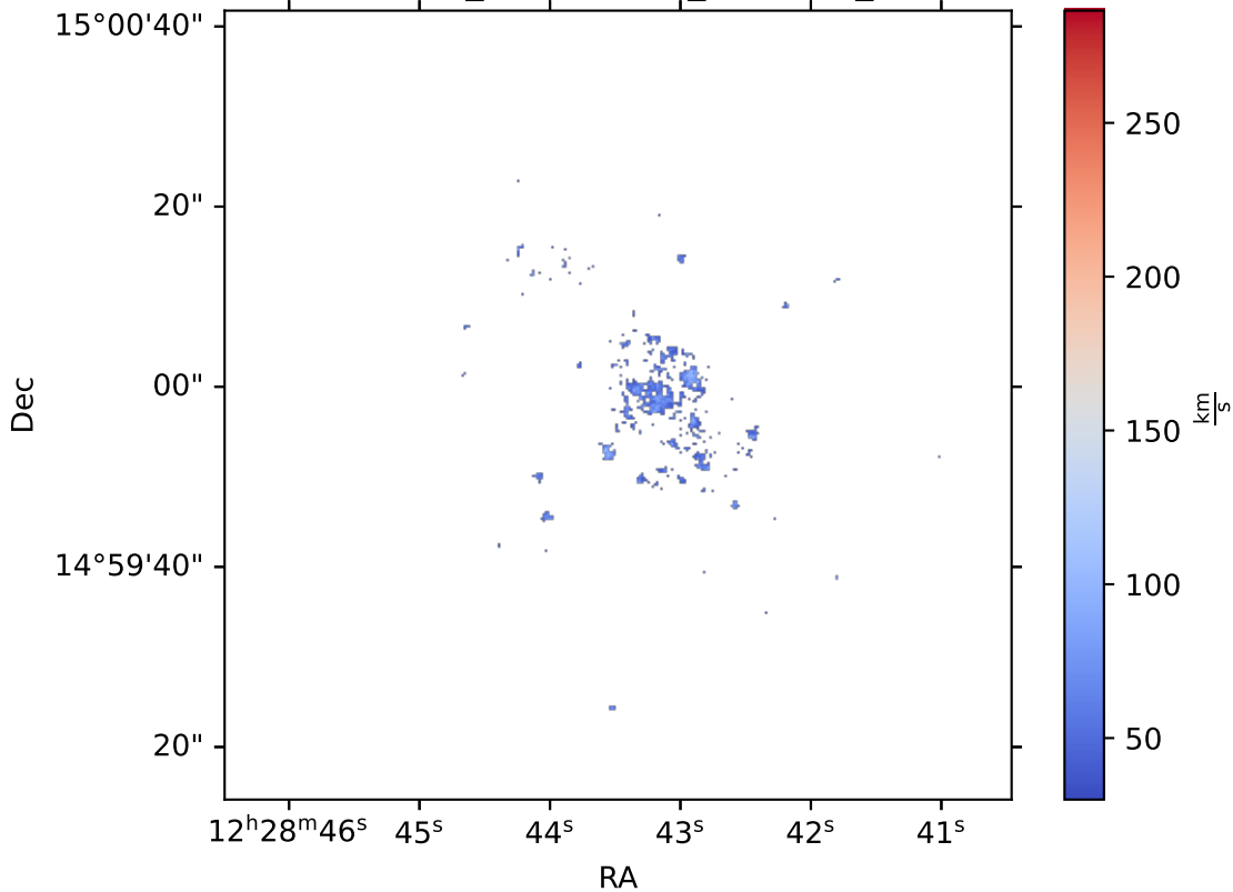
IC3392_multithresh_OIII5006_S
