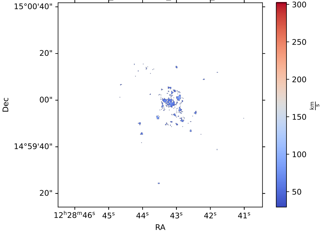
IC3392_multithresh_OIII5006_SIGMA
