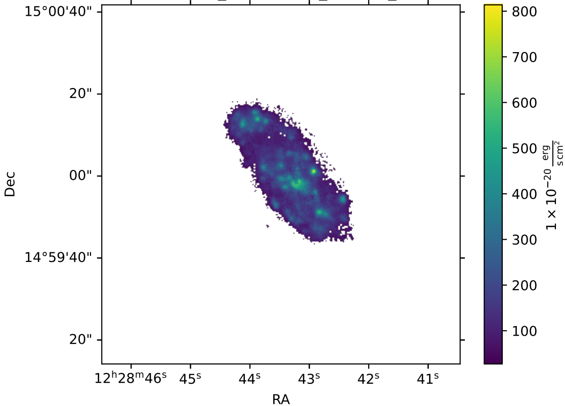
IC3392_multithresh_SII6716_I
