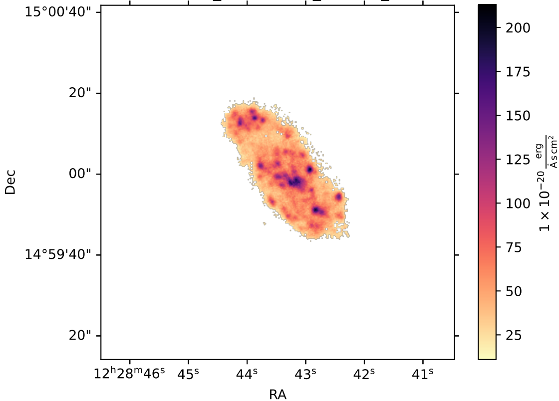
IC3392_multithresh_SII6716_P
