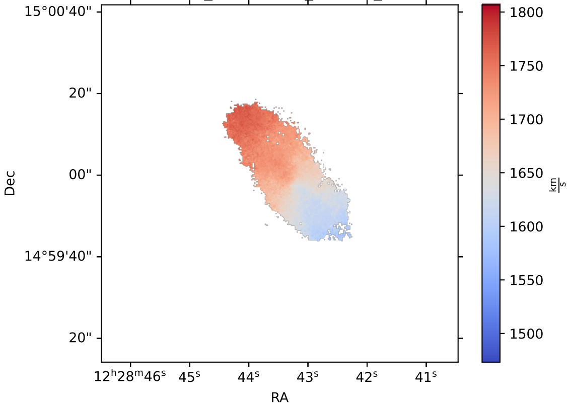
IC3392_multithresh_SII6716_VEL
