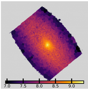
NGC4064: \log \Sigma_*
