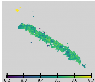
[O/H] (O3N2-M13, HII)
