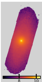
NGC4698: \log \Sigma_*
