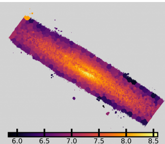
NGC4383: \log \Sigma_*
