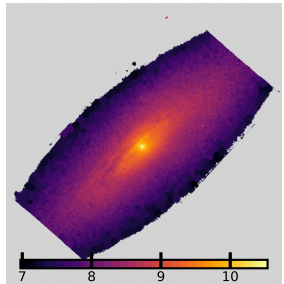
NGC4457: \log \Sigma_*
