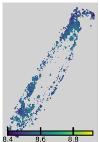
[O/H] (O3N2-M13, HII)
