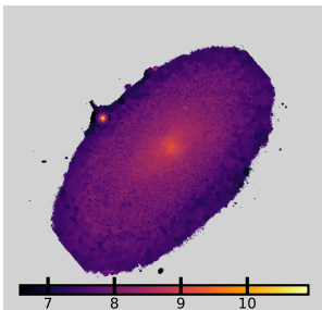
NGC4330: \log \Sigma_*
