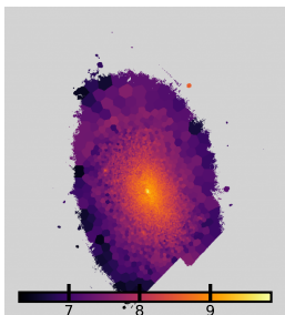
NGC4383: \log \Sigma_*
