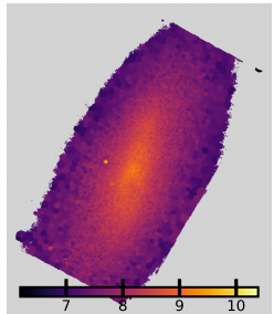
NGC4192: \log \Sigma_*
