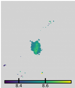
[O/H] (O3N2-M13, HII)
