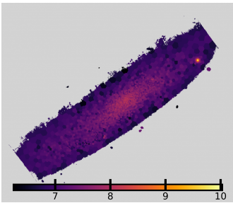
NGC4419: \log \Sigma_*
