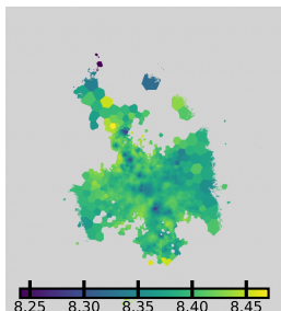
[O/H] (O3N2-M13, HII)
