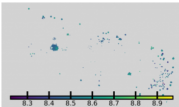
[O/H] (O3N2-M13, HII)
