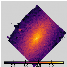
NGC4698: \log \Sigma_*
