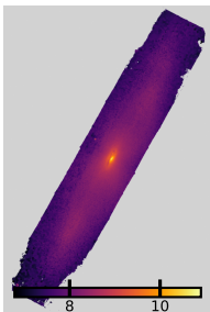
NGC4192: \log \Sigma_*
