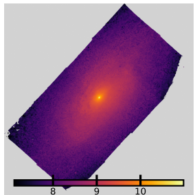
NGC4522: \log \Sigma_*
