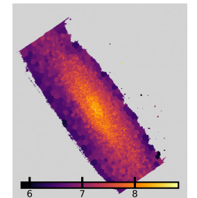
NGC4694: \log \Sigma_*
