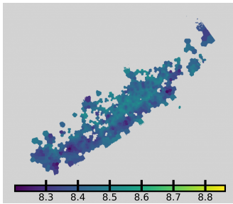
[O/H] (O3N2-M13, HII)
