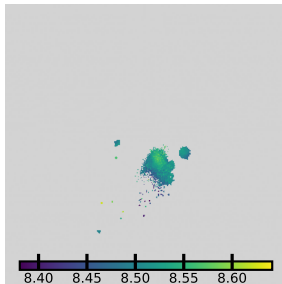
[O/H] (O3N2-M13, HII)
