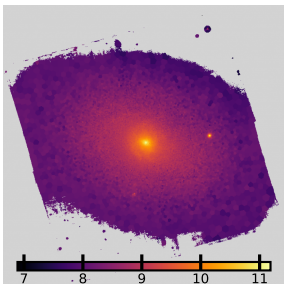
NGC4501: \log \Sigma_*
