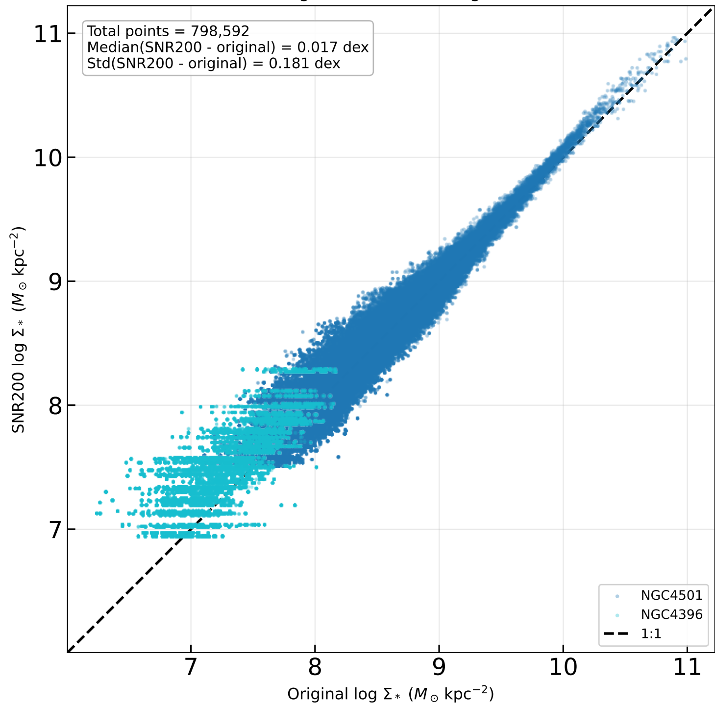
Original vs SNR200 \log \Sigma_*
