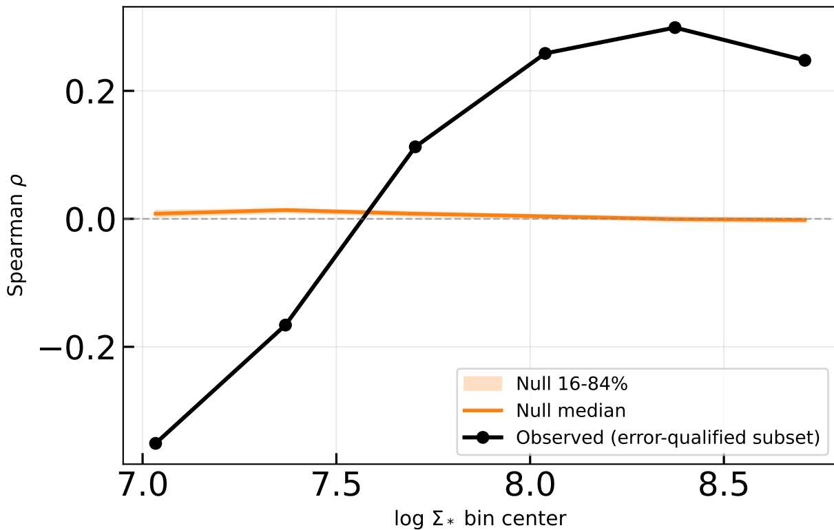
Observed vs null \rho(\log \Sigma_*)
