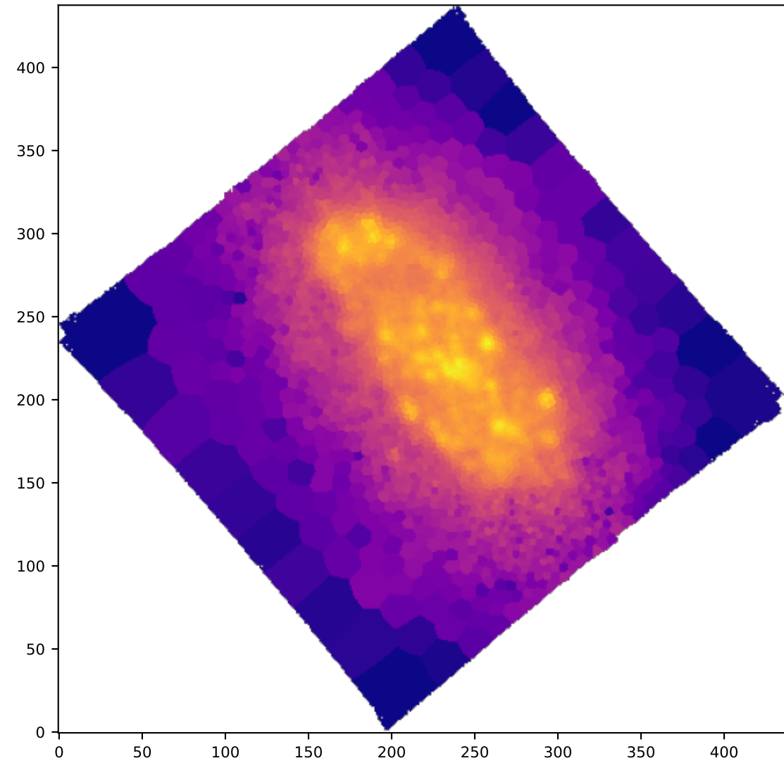
BIN SII6716_SIGMA
