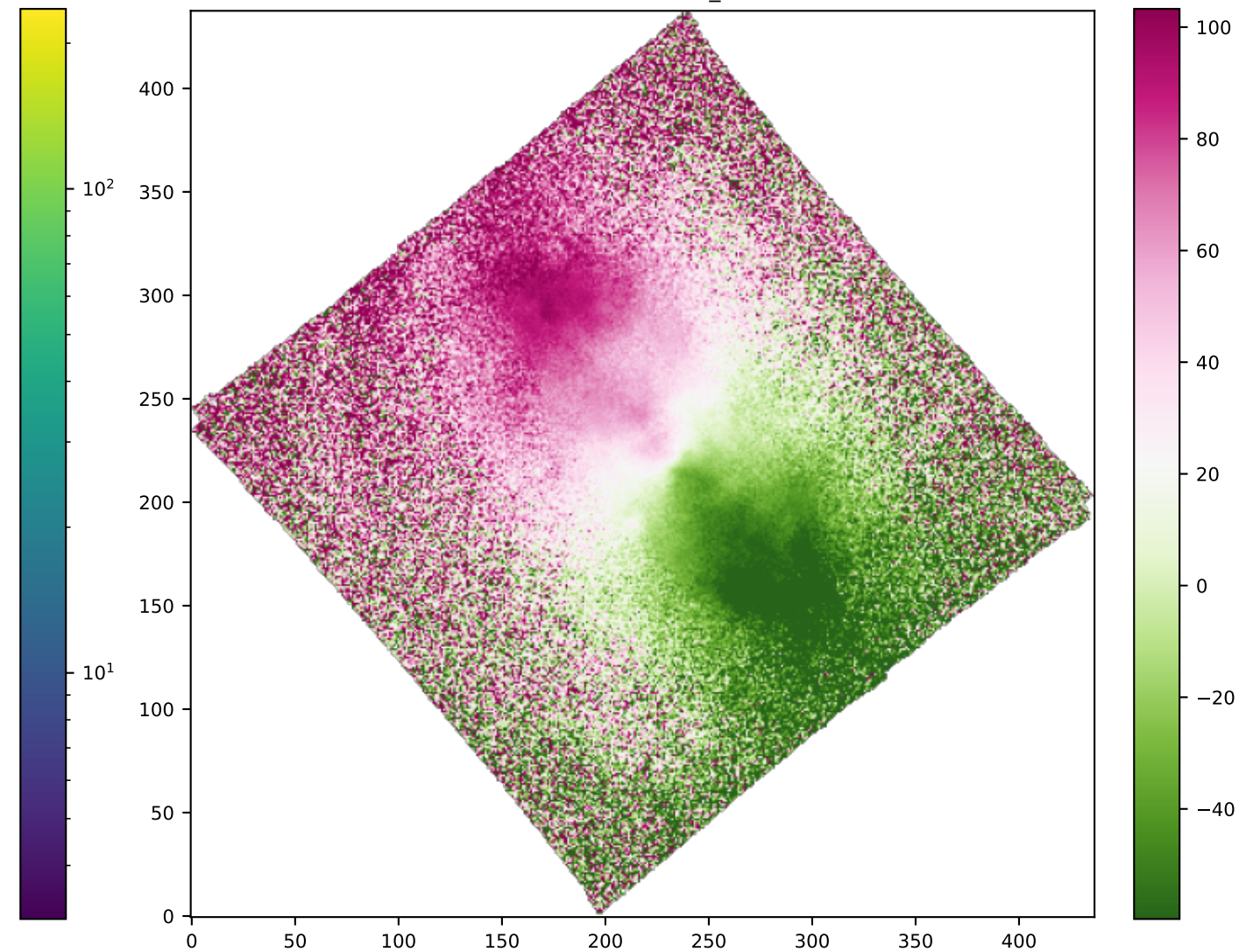
SPAXELS OI6363_VEL
