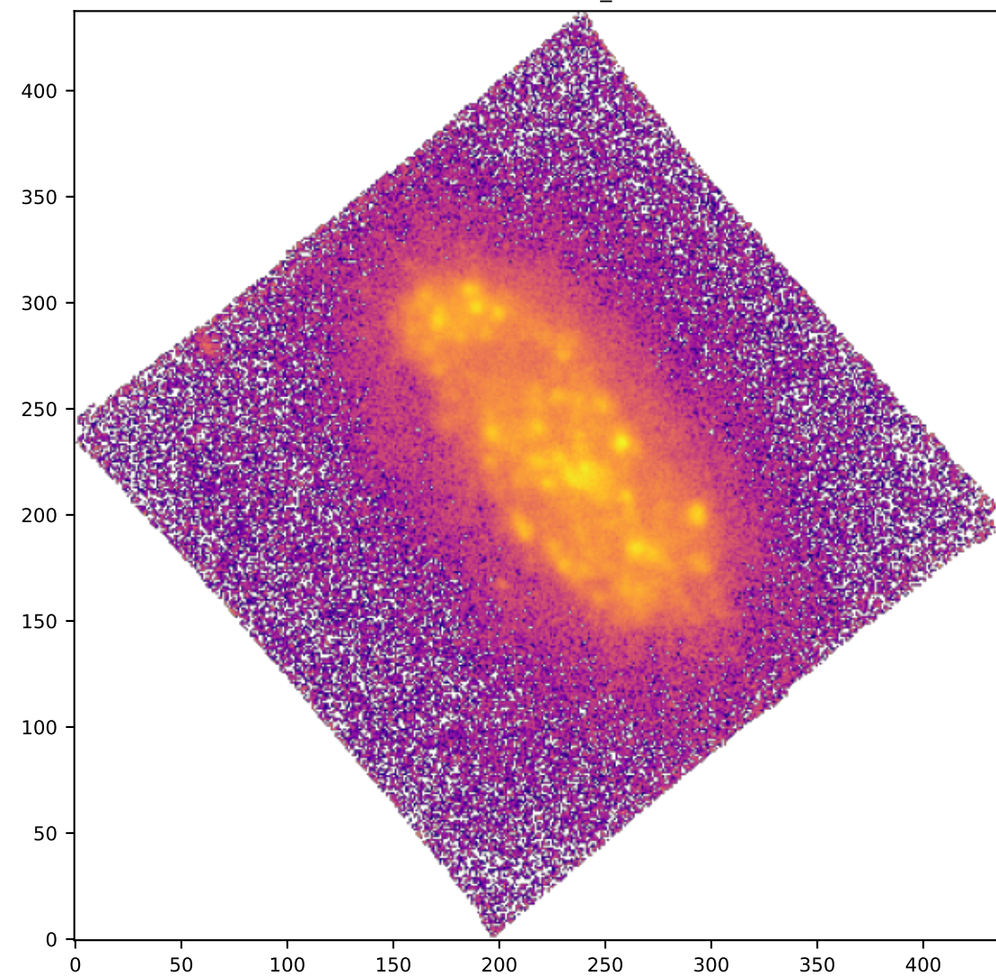
SPAXELS SII6716_SIGMA
