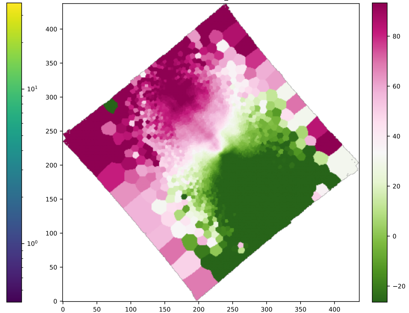
BIN HB4861_VEL
