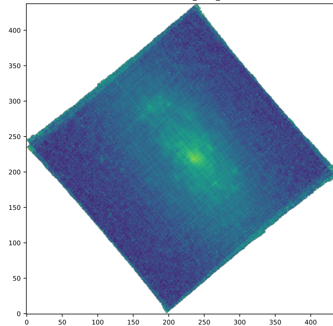
SPAXELS SII6716_SIGMA_ERR
