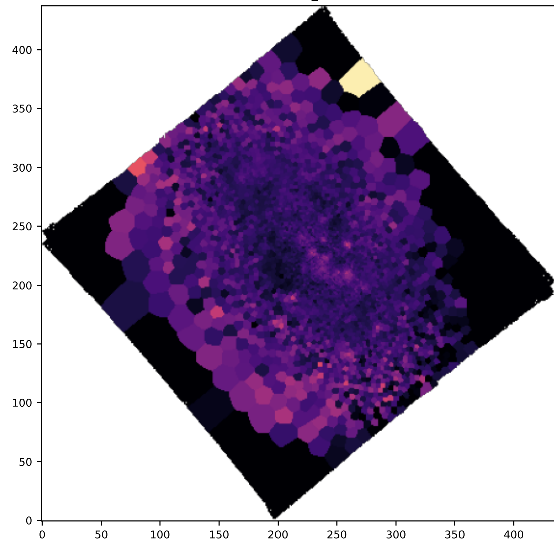
BIN OI6363_SIGMA
