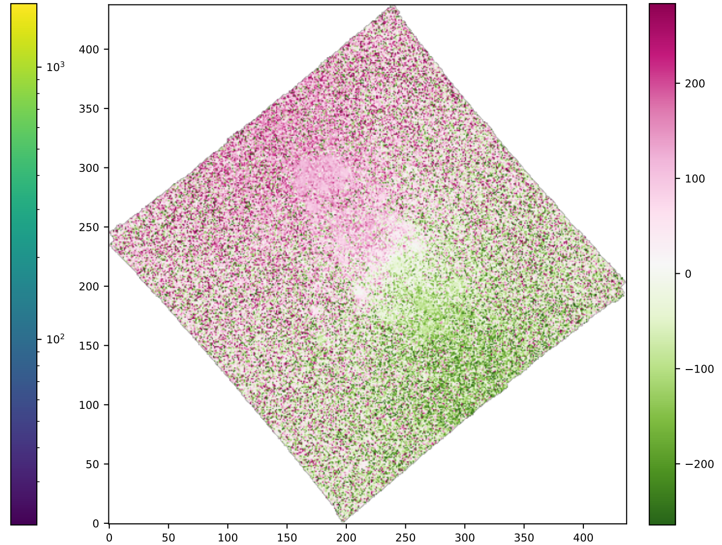
SPAXELS OIII5006_VEL
