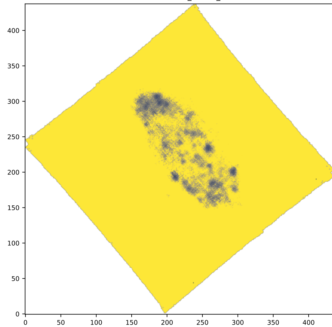
SPAXELS OI6363_SIGMA_ERR
