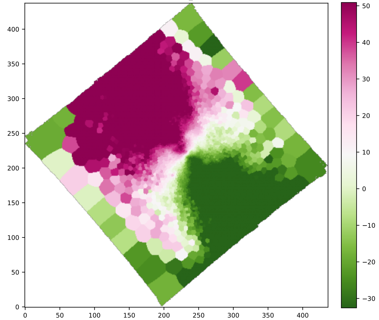
BIN OI6363_VEL
