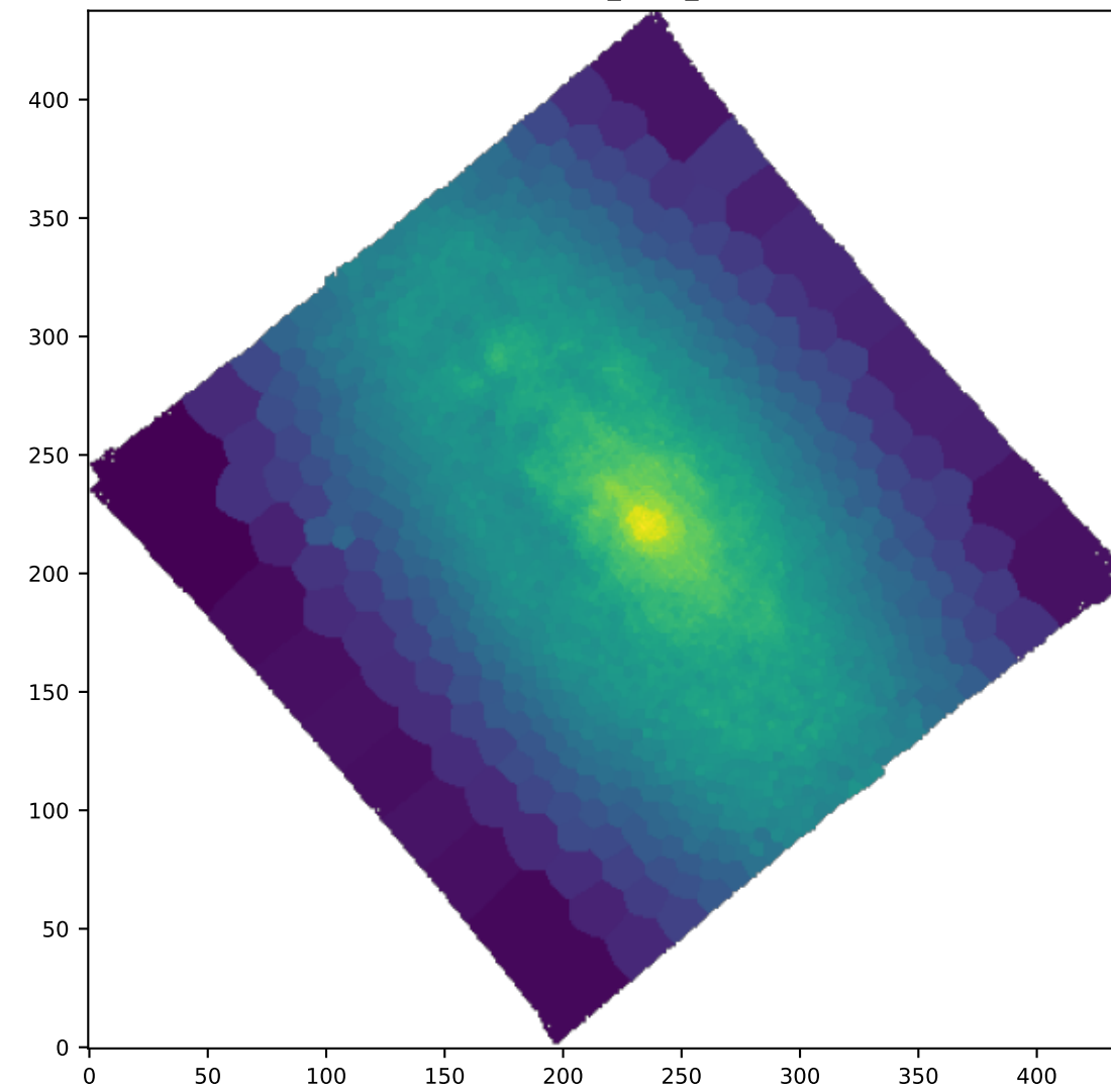
BIN OI6363_SIGMA_ERR
