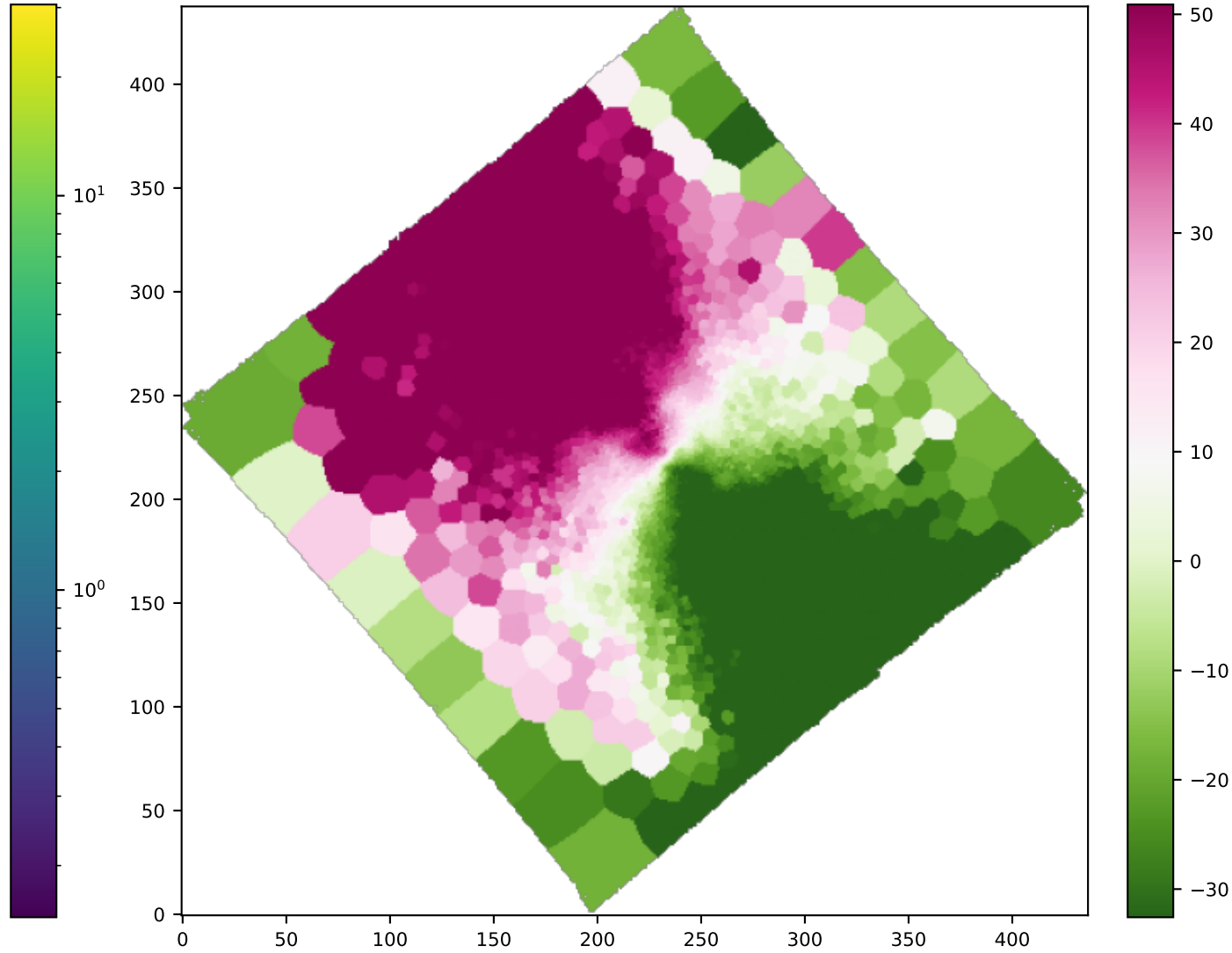
BIN SII6716_VEL
