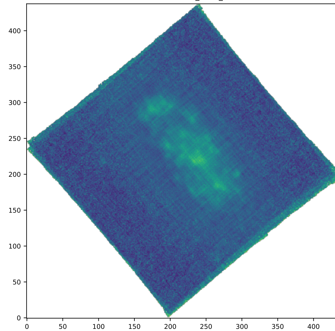
SPAXELS HB4861_SIGMA_ERR
