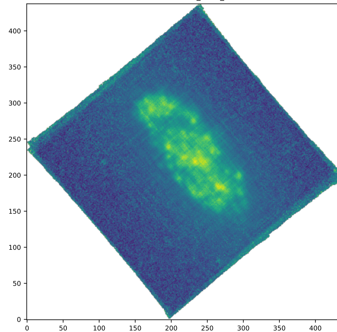
SPAXELS HA6562_SIGMA_ERR
