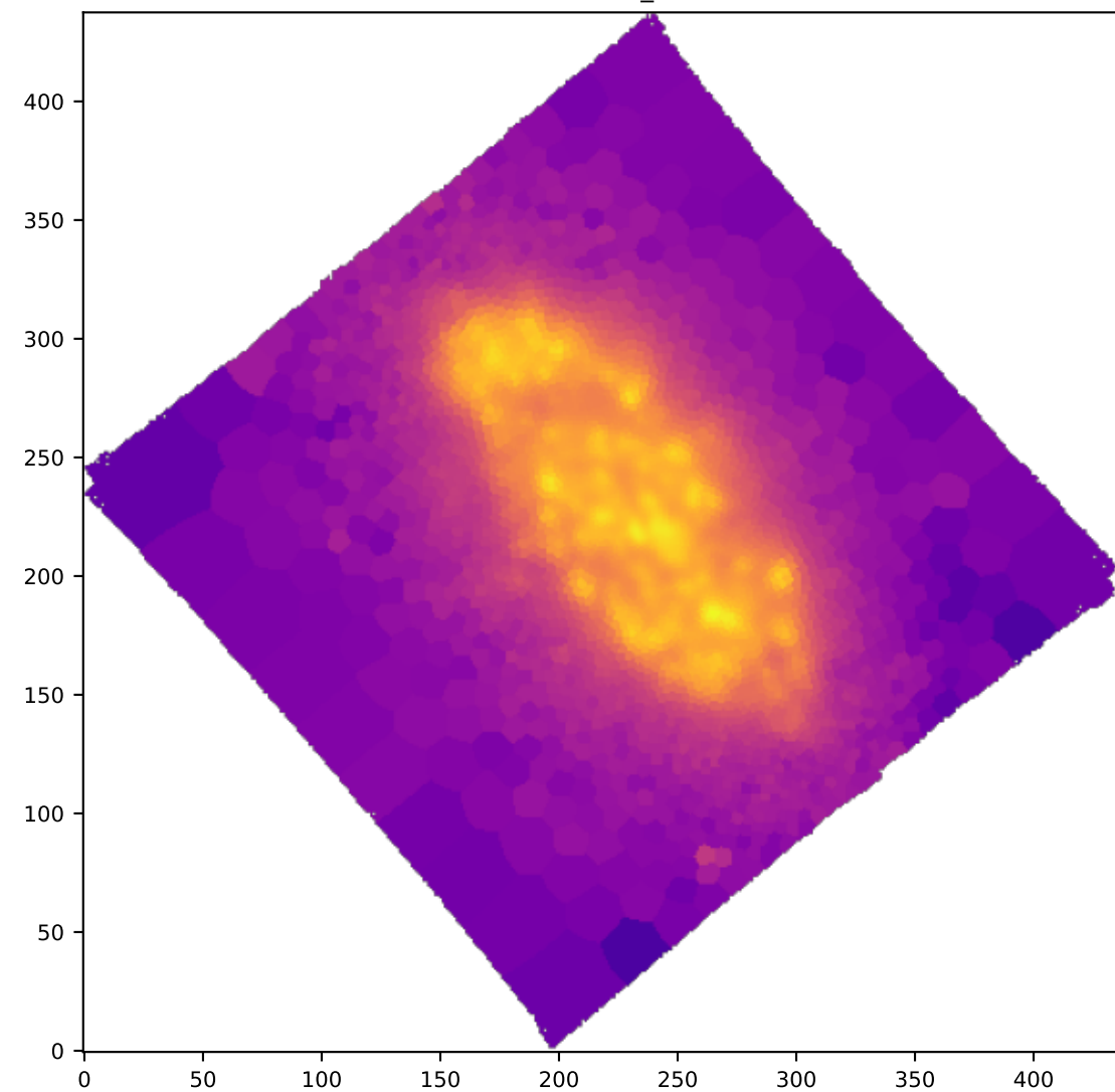
BIN HA6562_SIGMA
