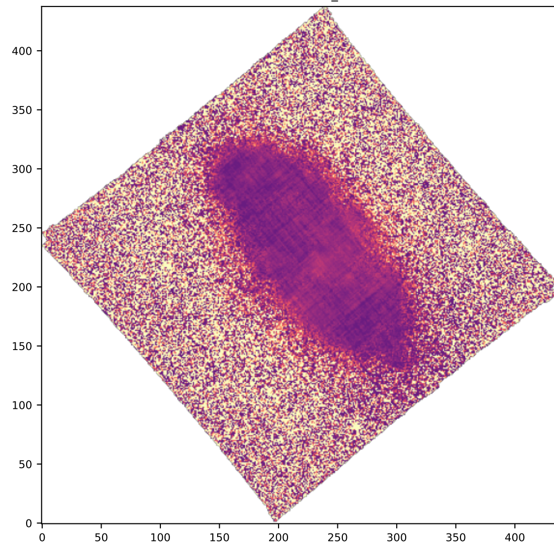
SPAXELS HB4861_SIGMA
