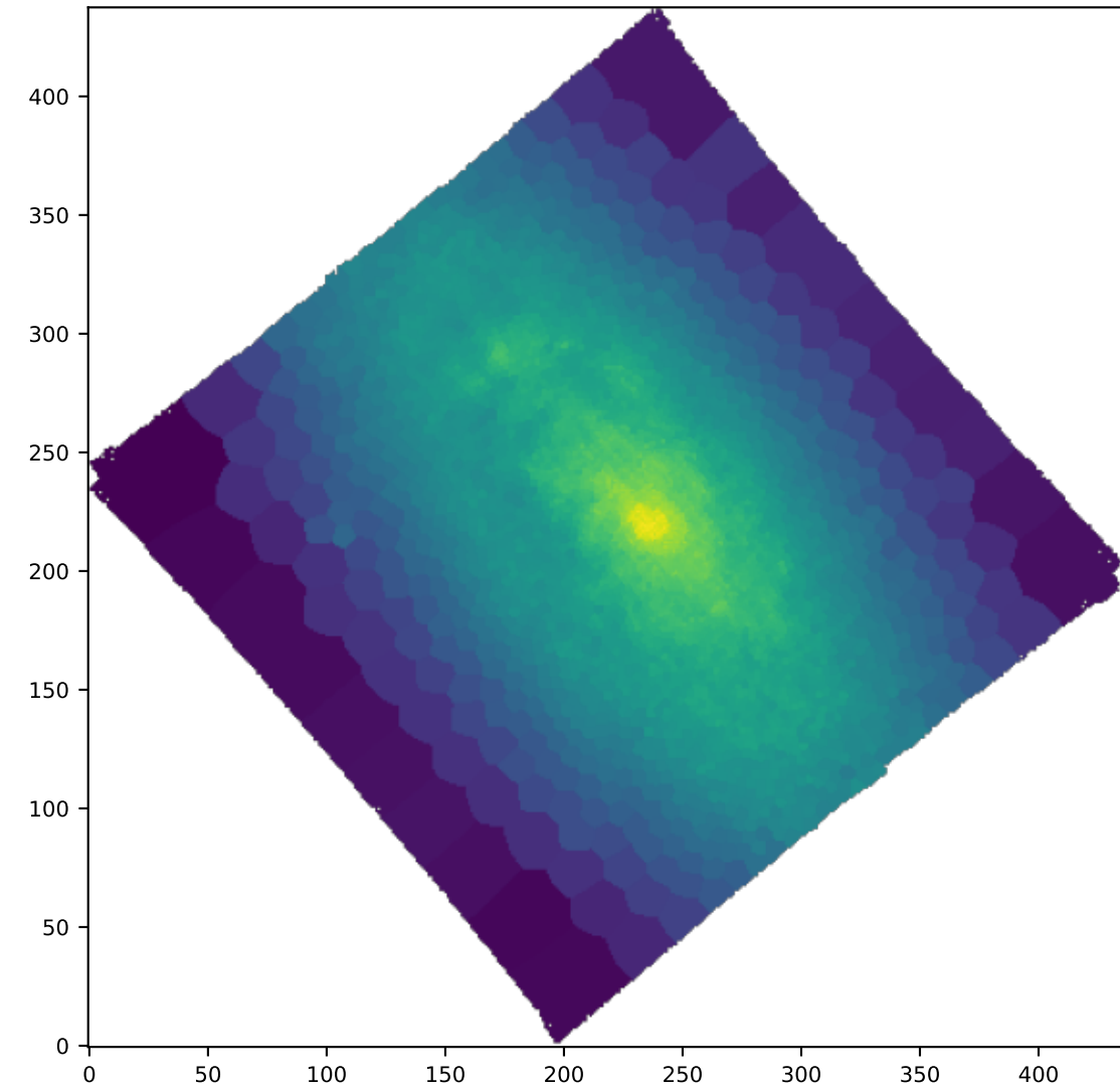
BIN SII6716_SIGMA_ERR
