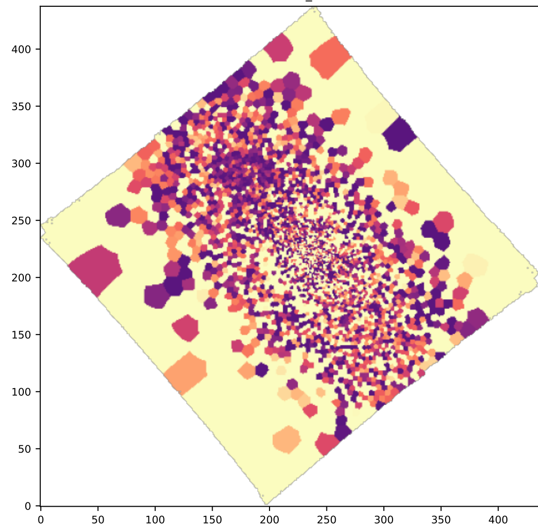
BIN OIII5006_SIGMA
