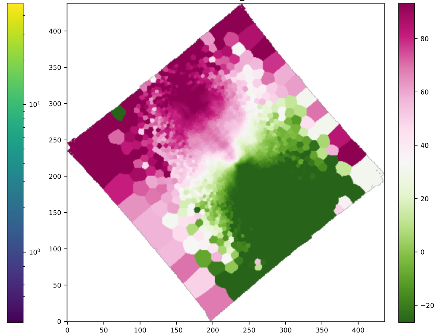
BIN HA6562_VEL
