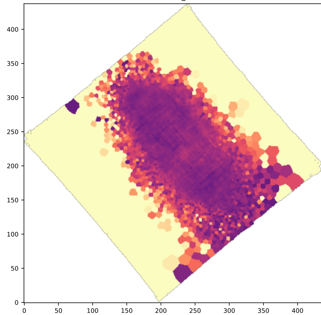
BIN HB4861_SIGMA
