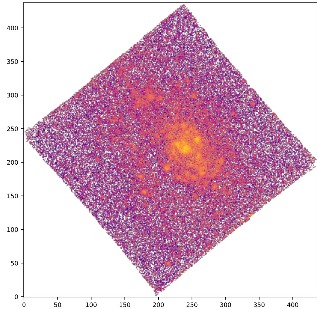
SPAXELS OIII5006_SIGMA
