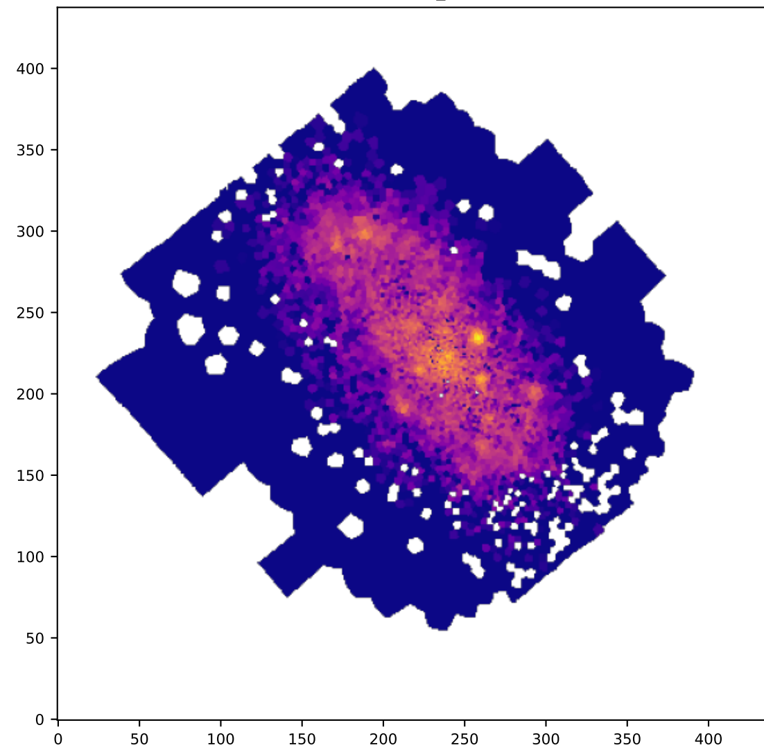
BIN OI6363_SIGMA
