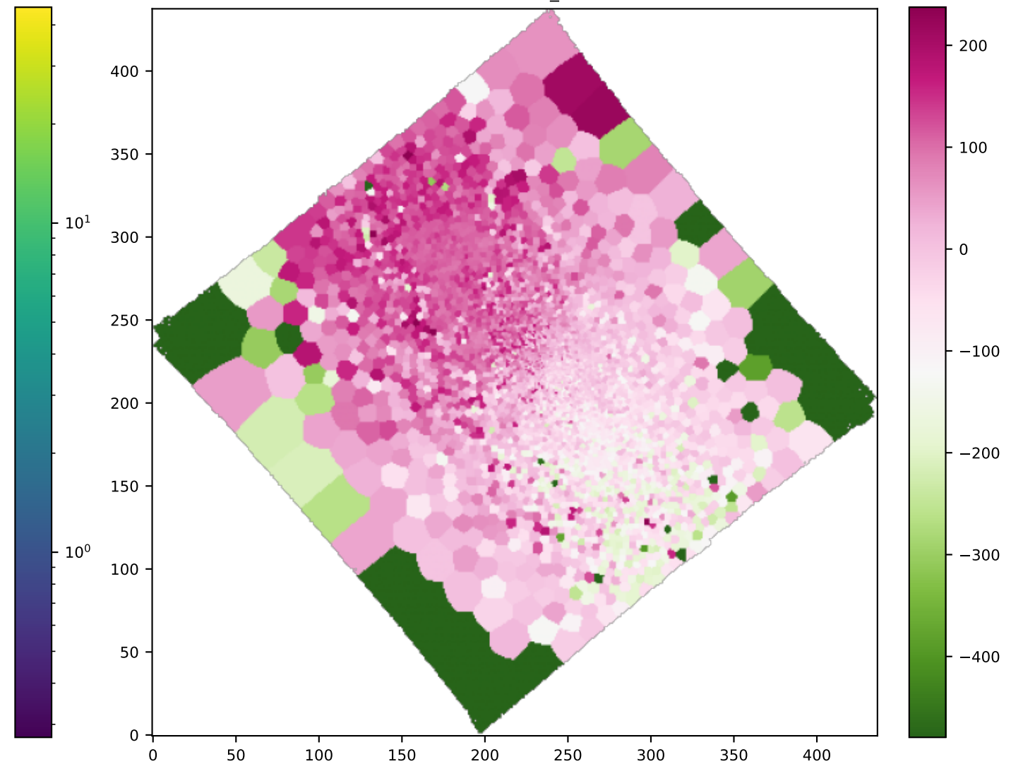
BIN OIII5006_VEL
