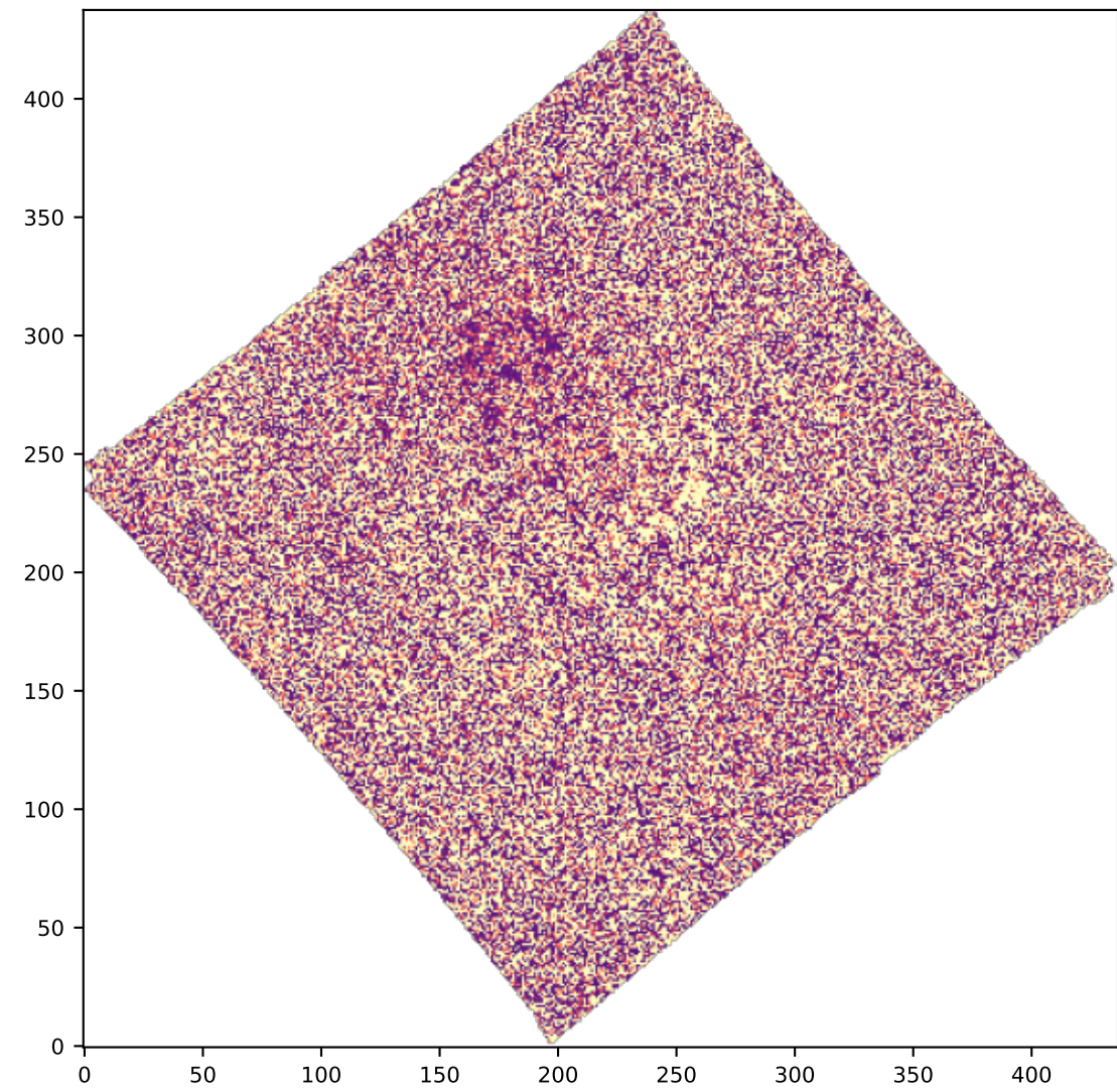
SPAXELS OIII5006_SIGMA
