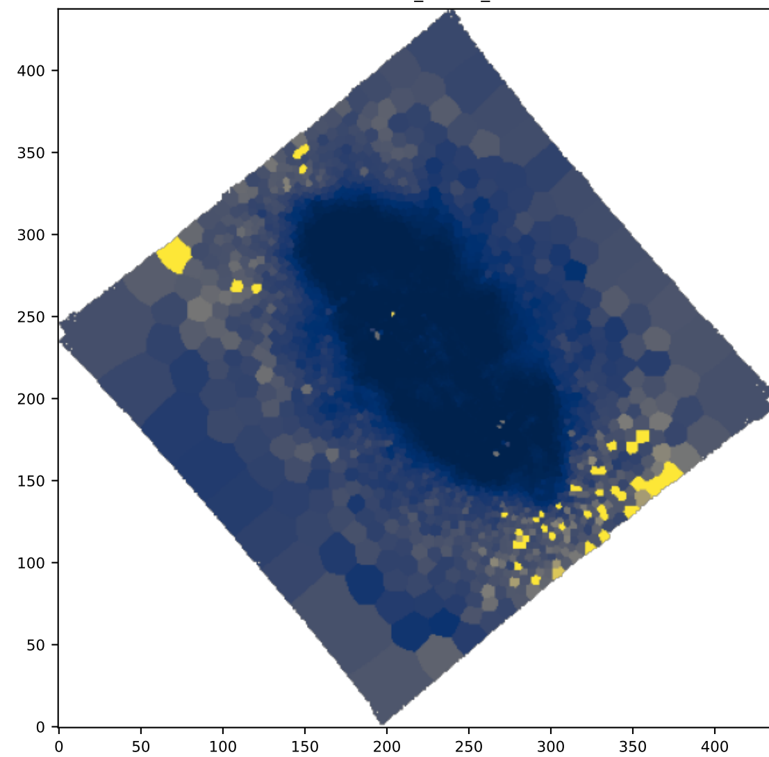
BIN HB4861_SIGMA_ERR
