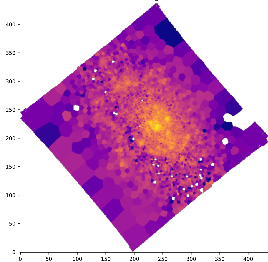
BIN OIII5006_SIGMA
