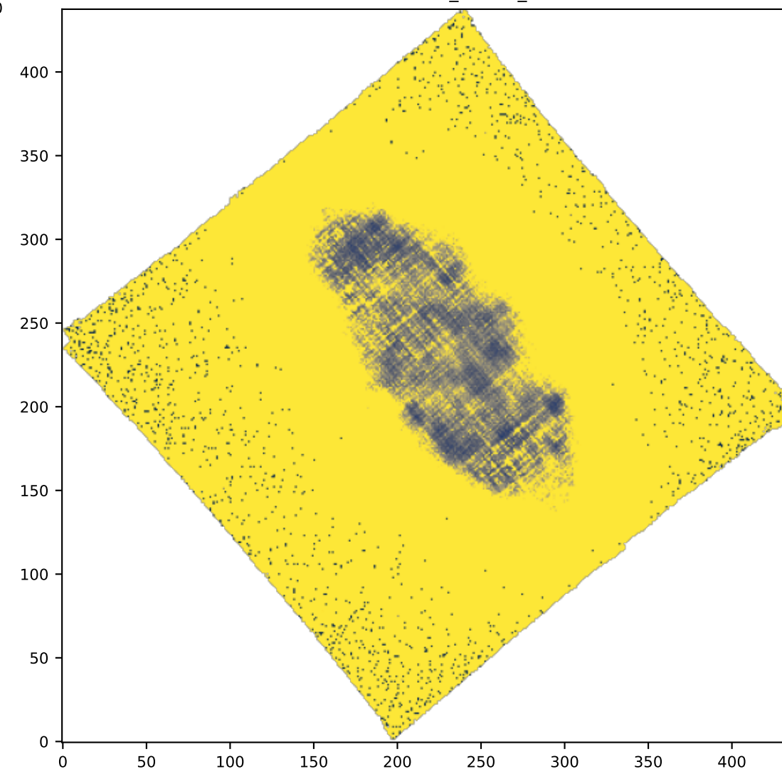
SPAXELS HB4861_SIGMA_ERR
