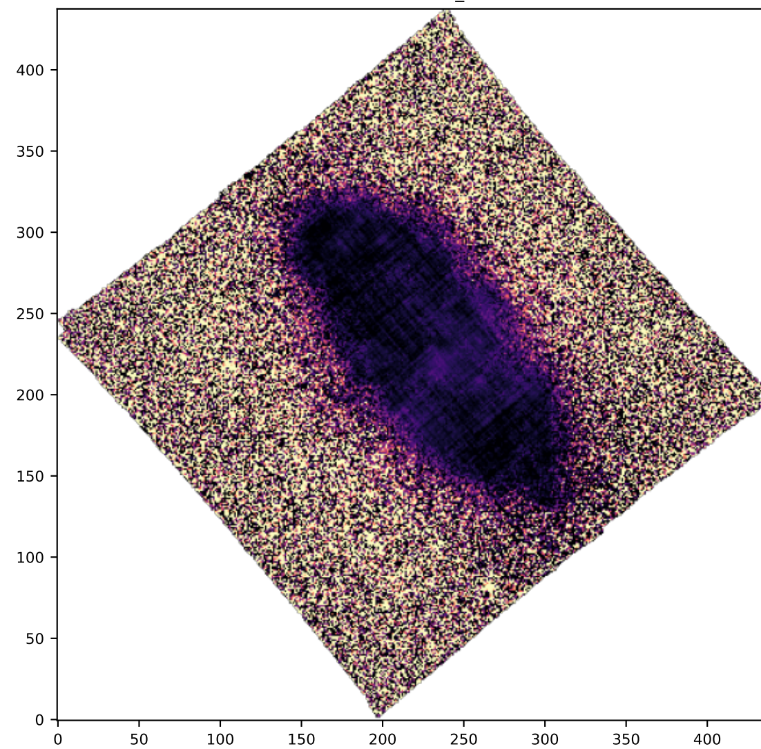
SPAXELS HA6562_SIGMA
