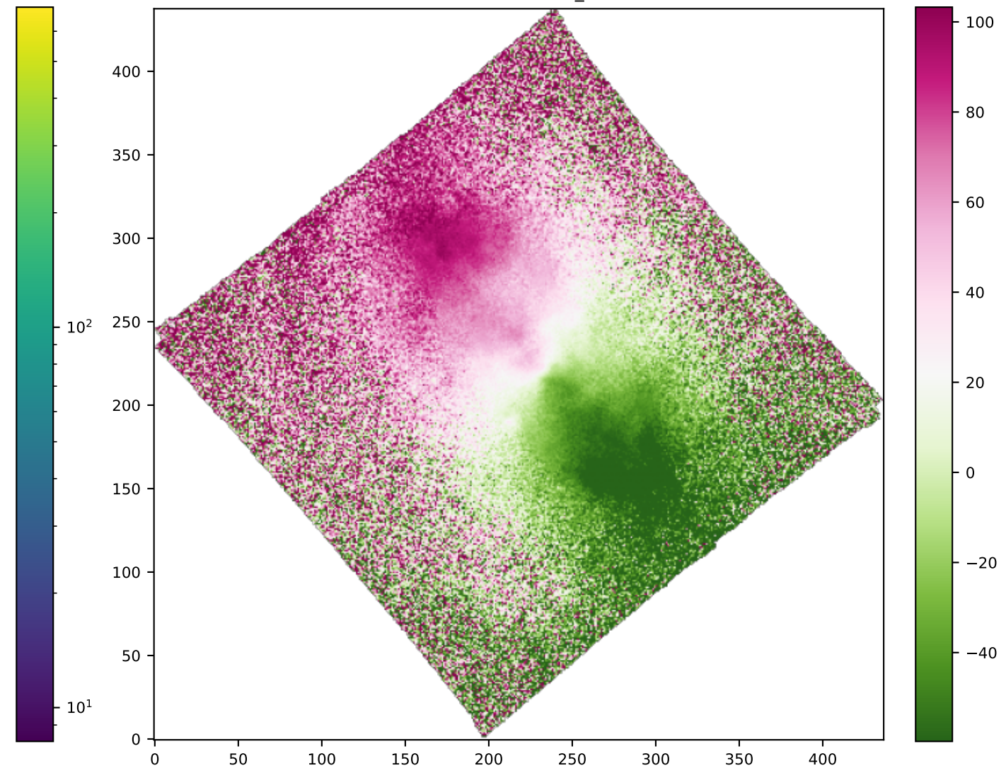
SPAXELS NII6583_VEL
