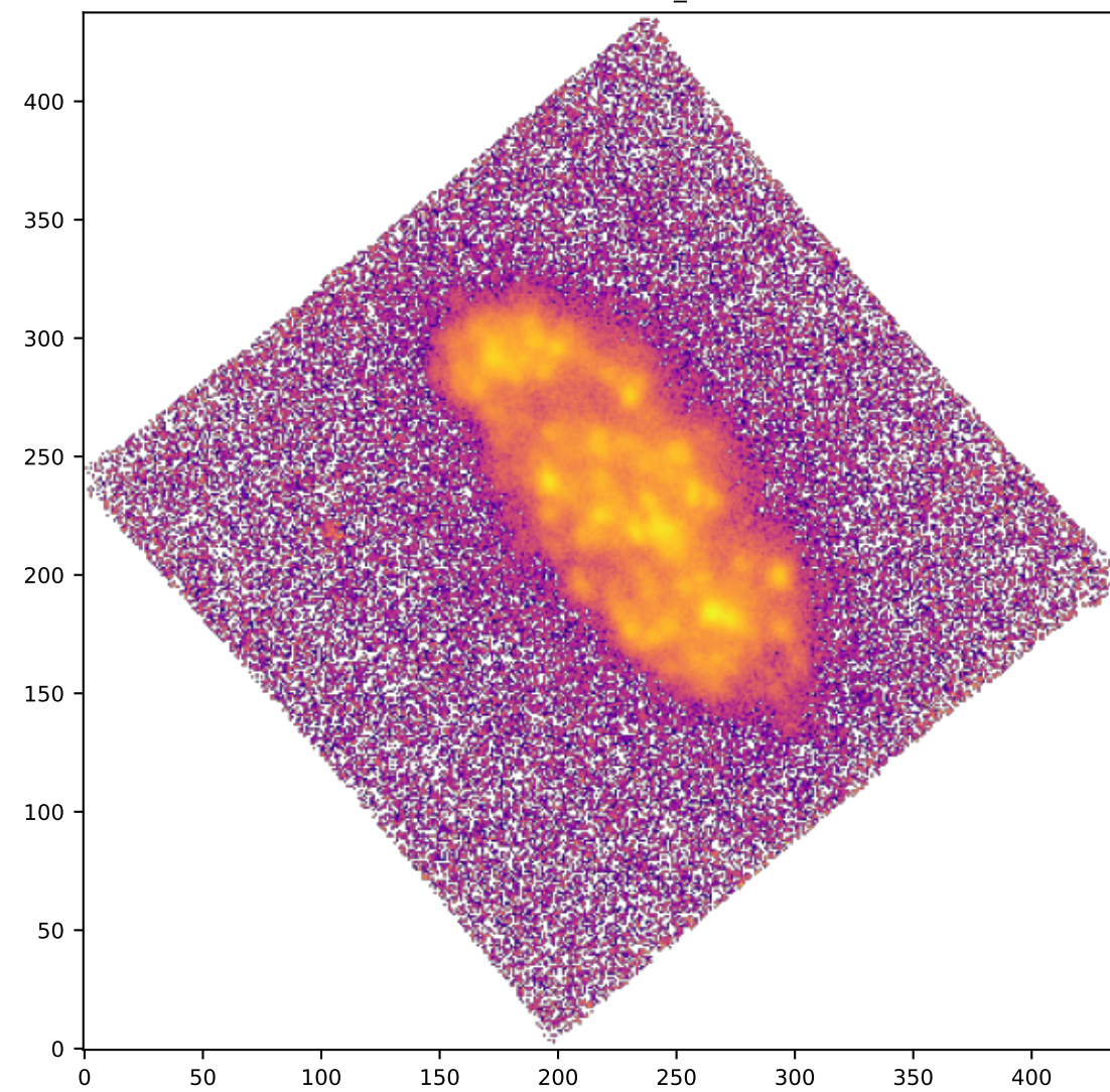
SPAXELS HB4861_SIGMA
