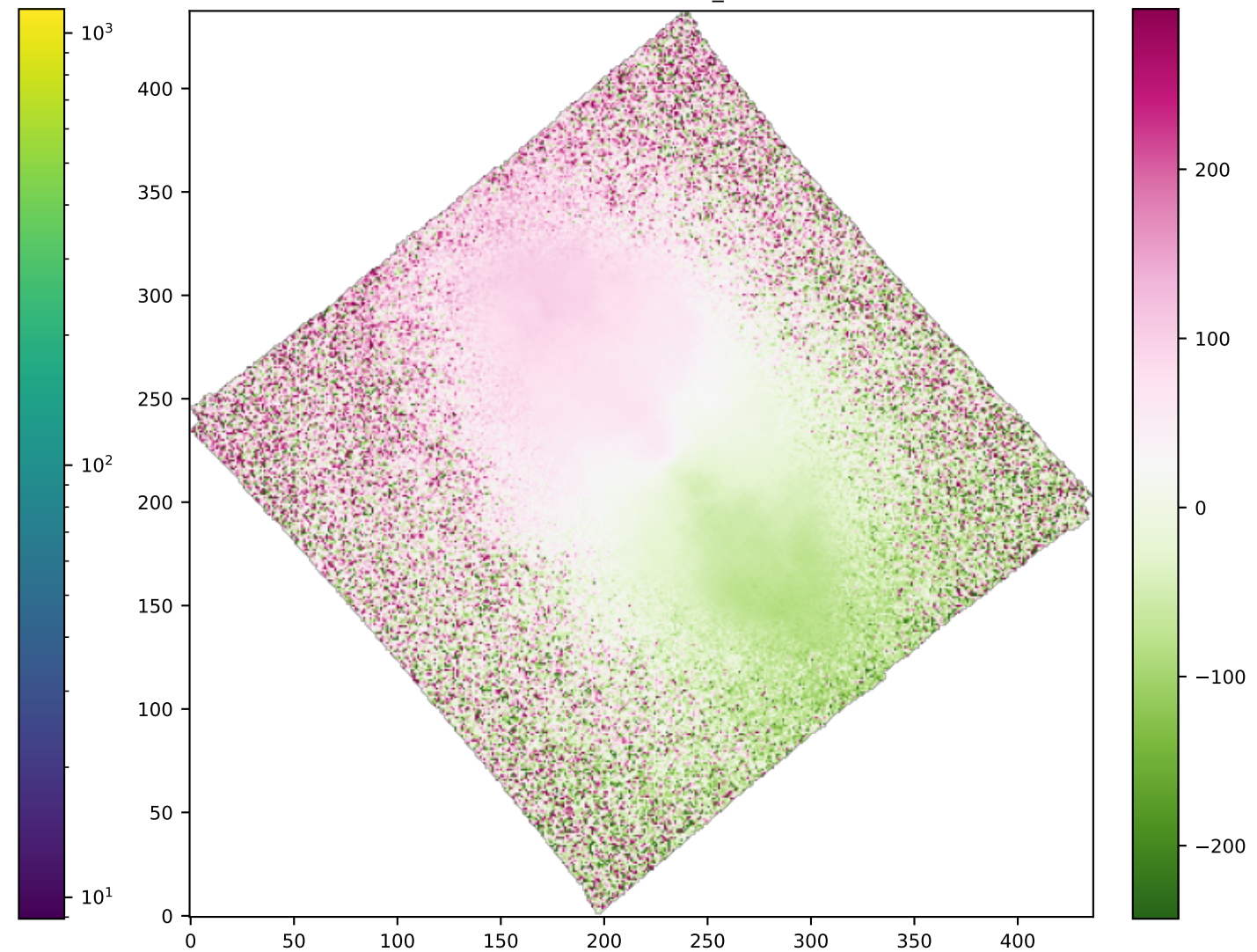
SPAXELS HA6562_VEL
