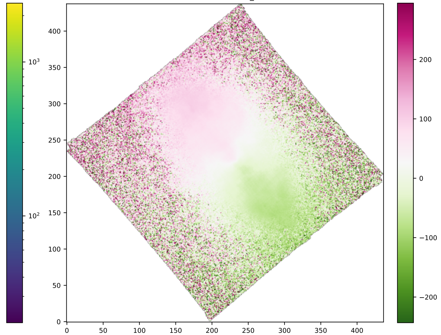
SPAXELS HB4861_VEL
