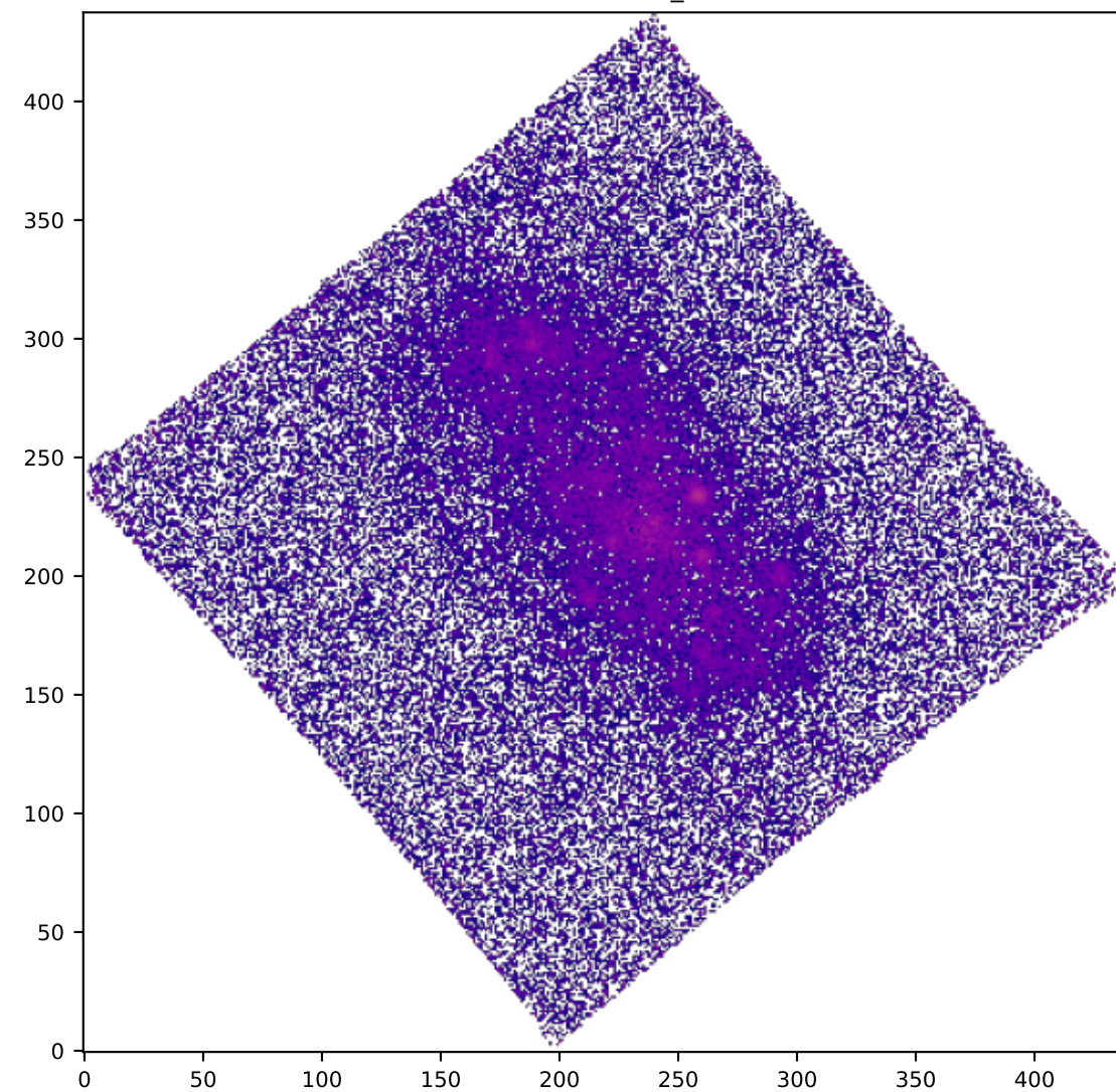
SPAXELS OI6363_SIGMA
