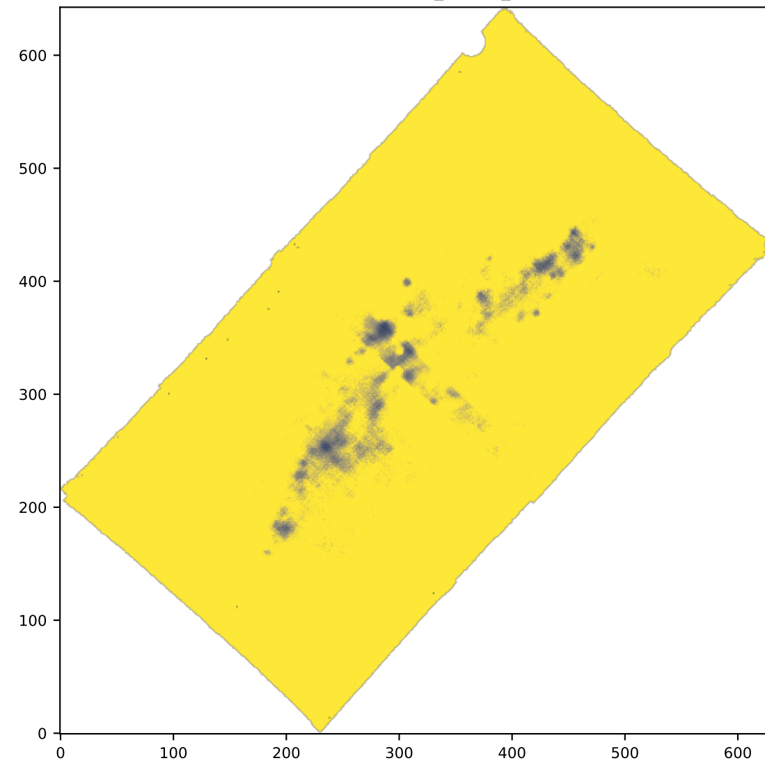
SPAXELS SII6716_SIGMA_ERR
