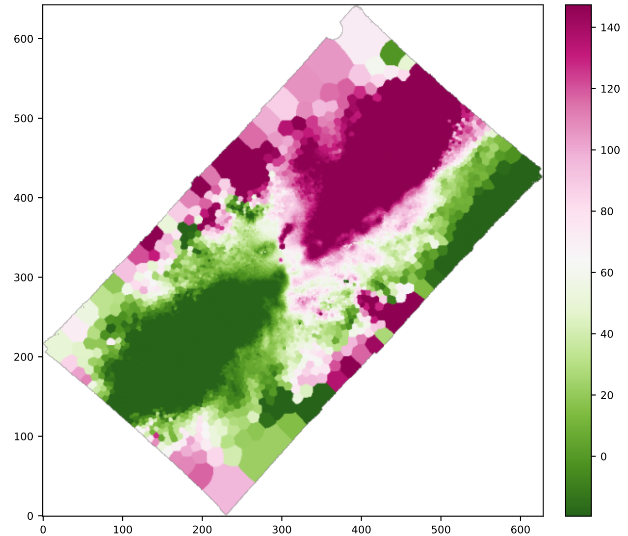
BIN SII6716_VEL
