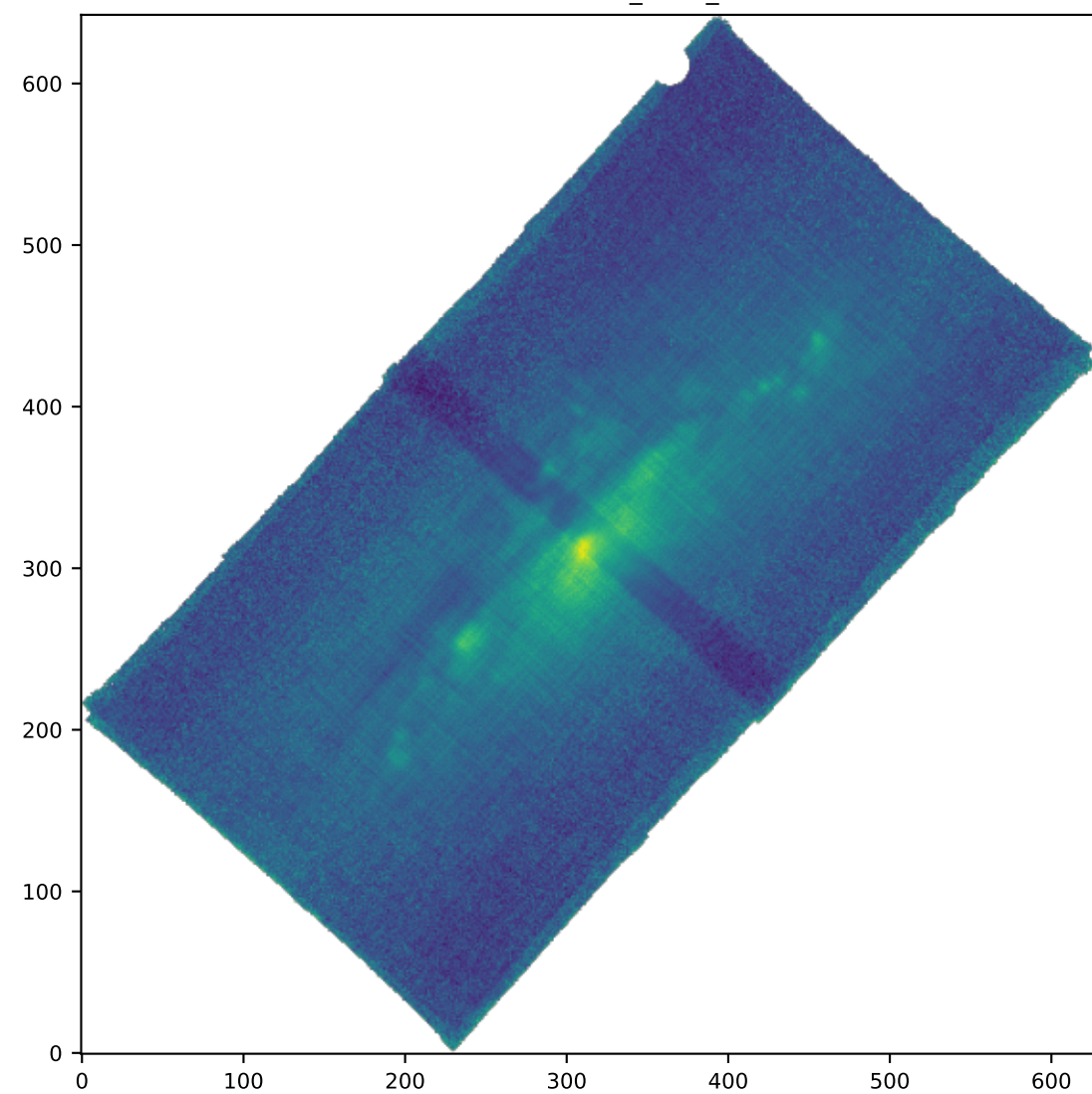
SPAXELS HB4861_SIGMA_ERR
