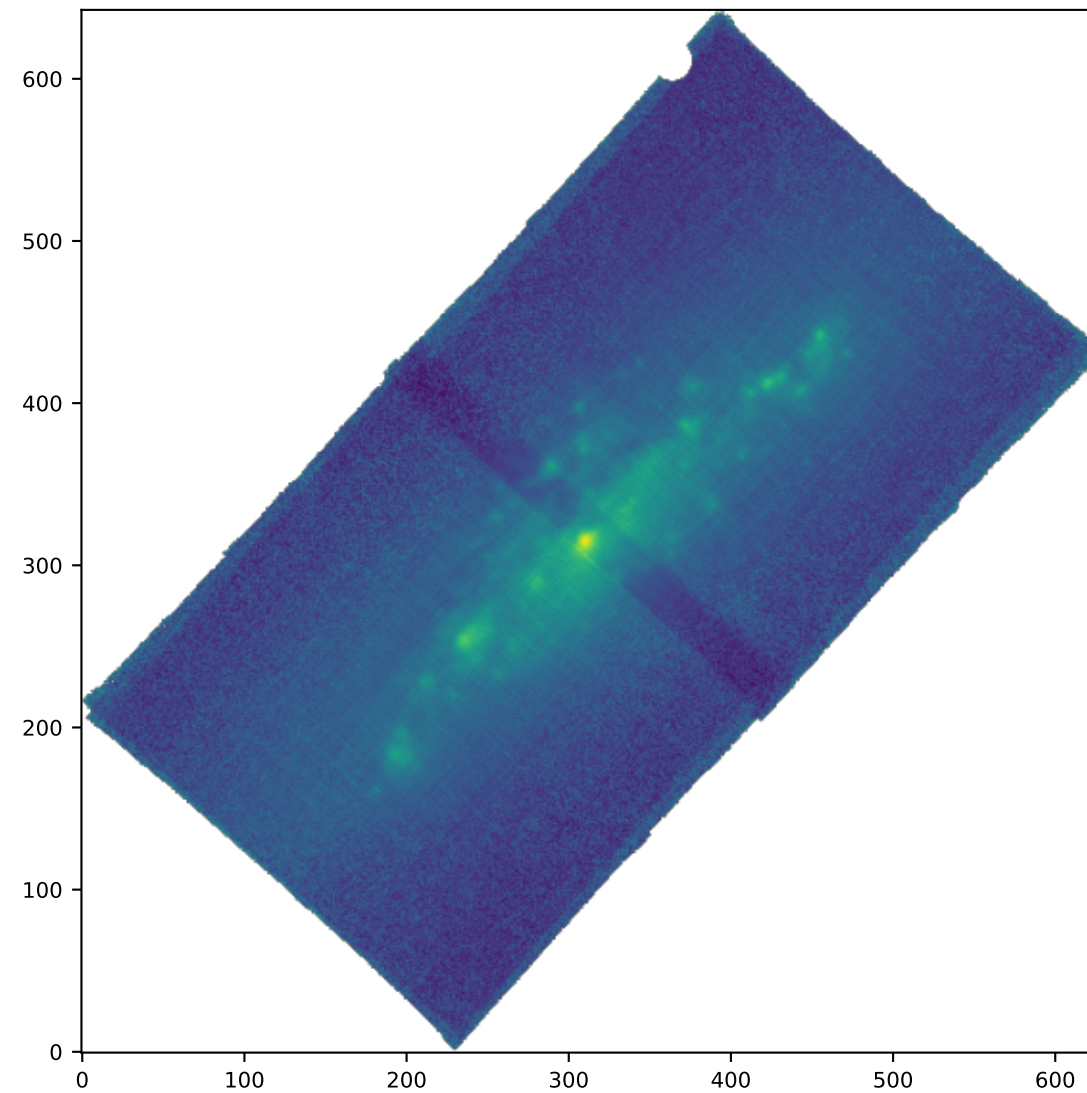
SPAXELS HA6562_SIGMA_ERR
