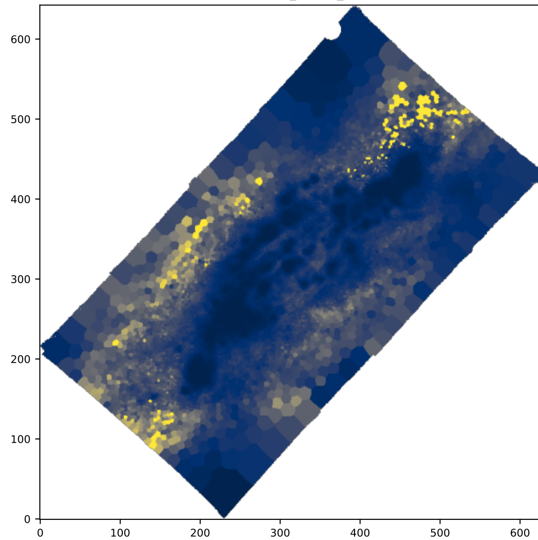
BIN HB4861_SIGMA_ERR
