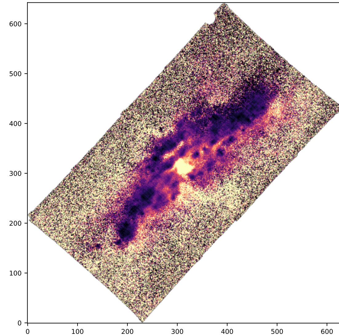
SPAXELS HA6562_SIGMA
