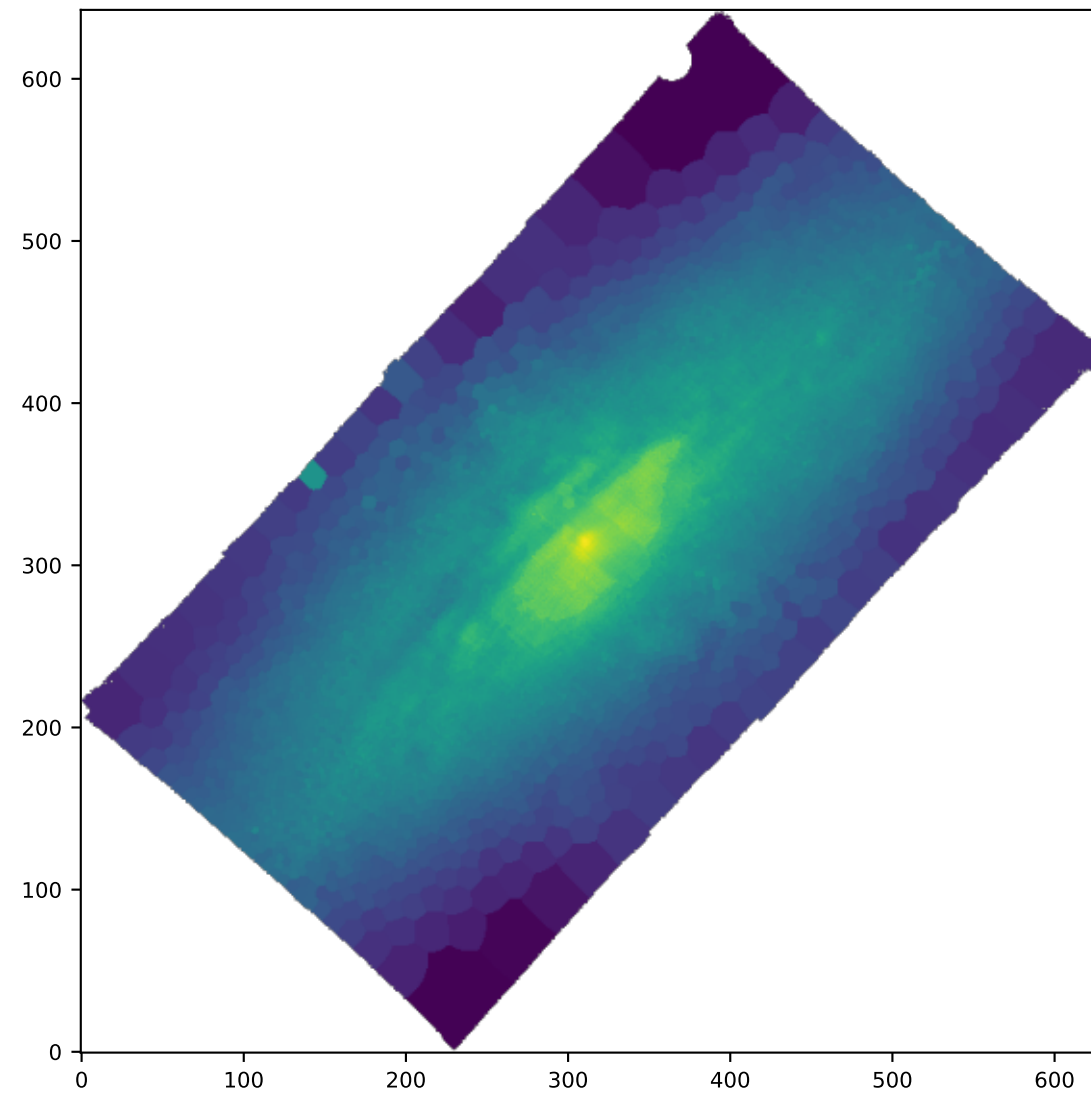
BIN SII6716_SIGMA_ERR
