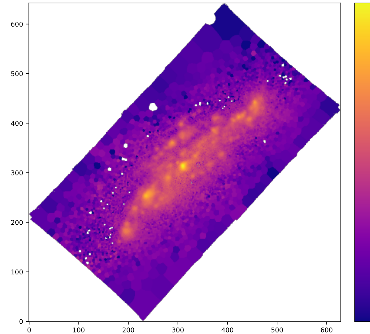
BIN HB4861_SIGMA
