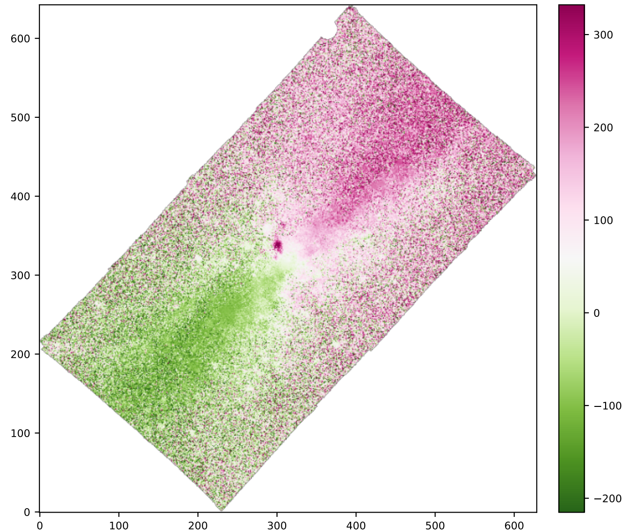
SPAXELS OIII5006_VEL
