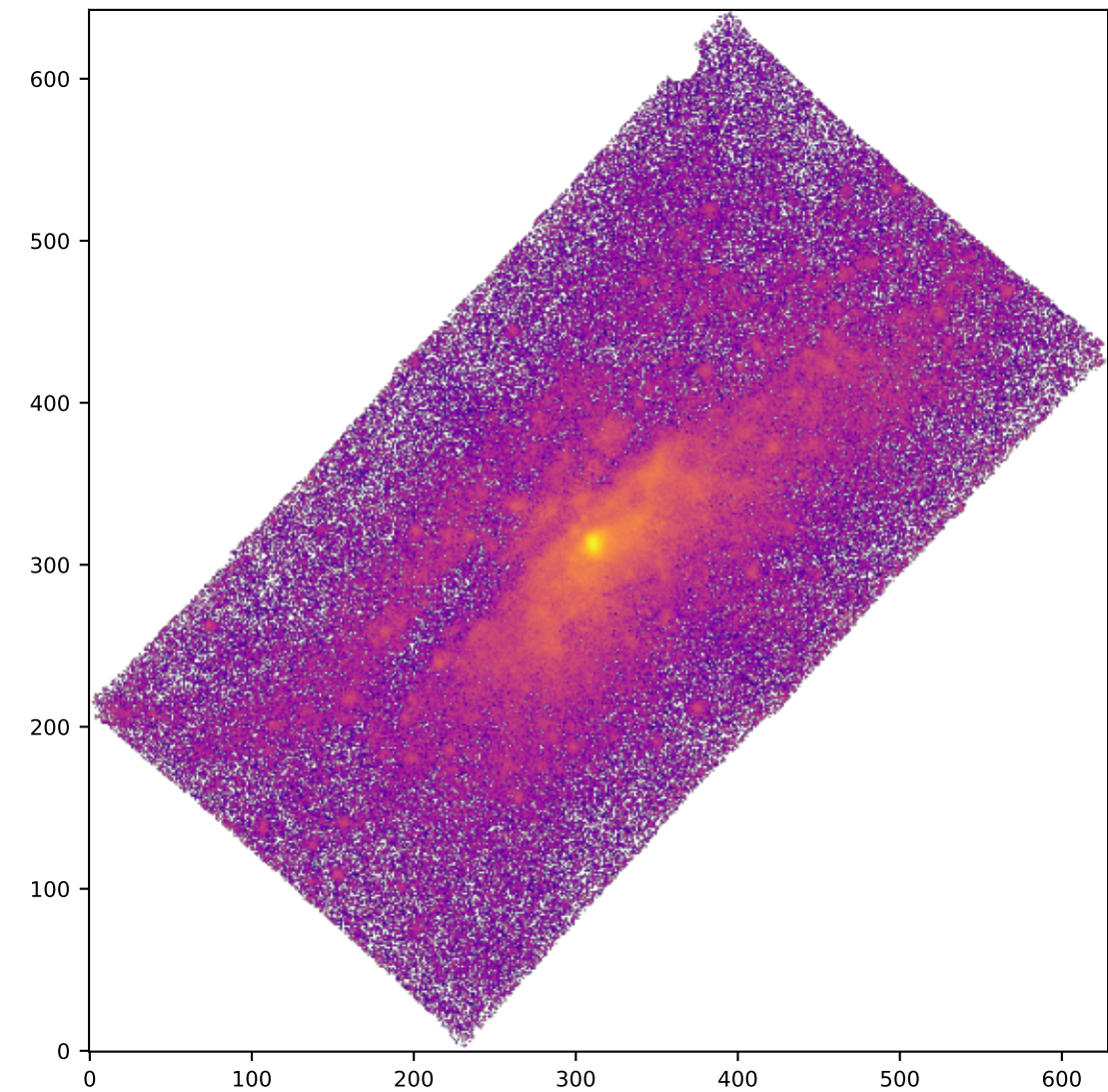
SPAXELS OIII5006_SIGMA
