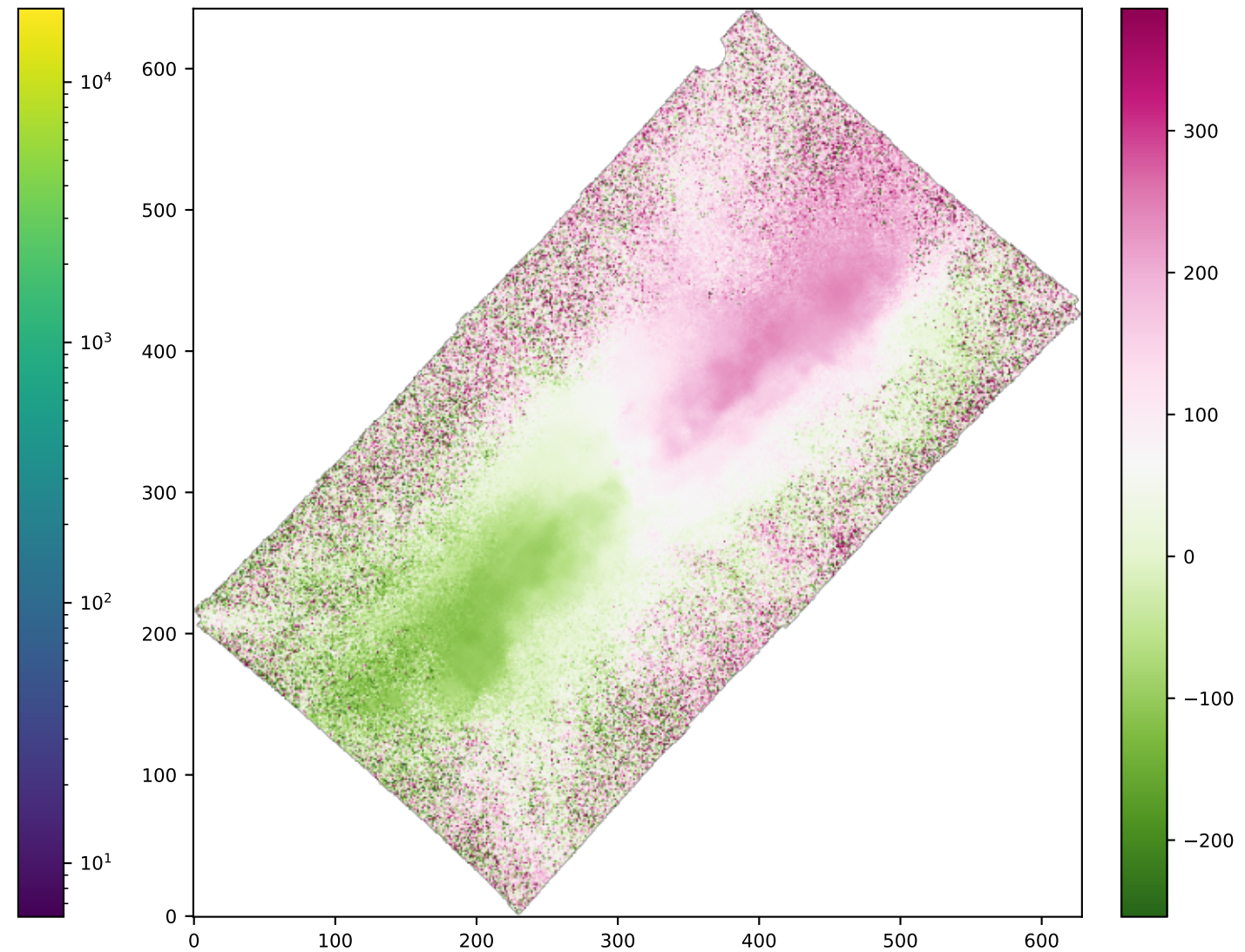
SPAXELS HA6562_VEL
