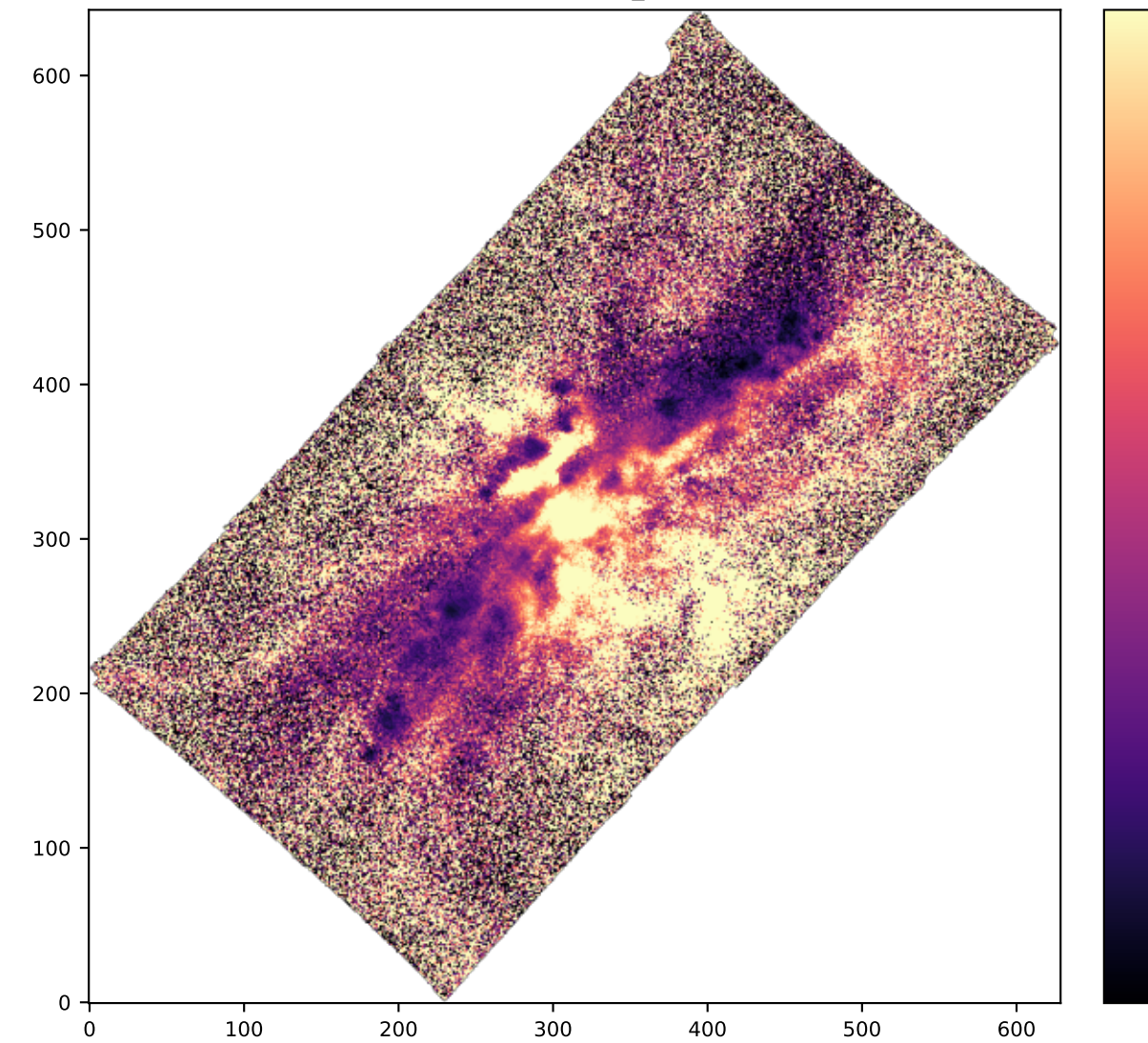
SPAXELS SII6716_SIGMA
