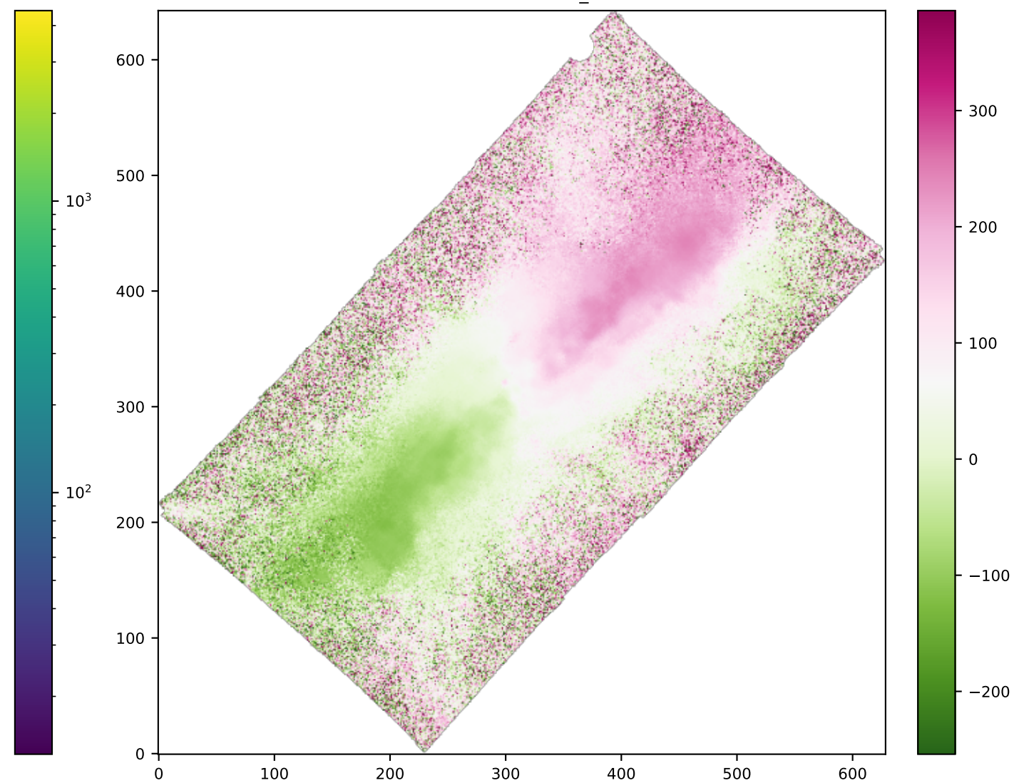
SPAXELS HB4861_VEL
