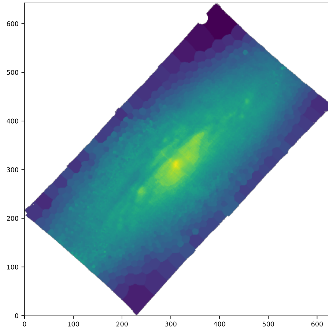
BIN HB4861_SIGMA_ERR
