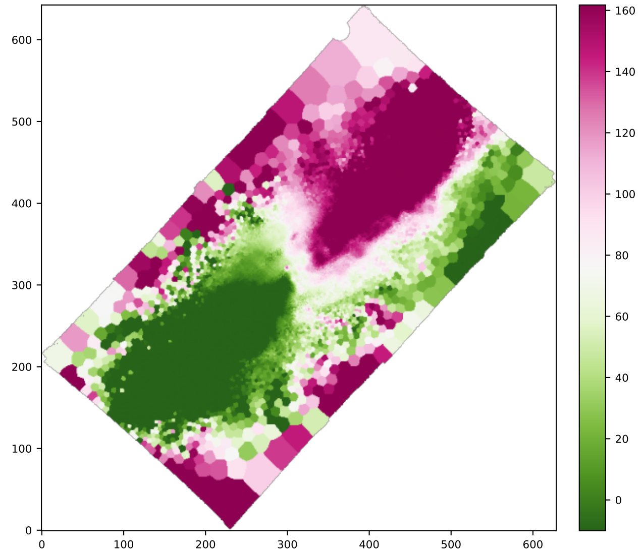
BIN HB4861_VEL
