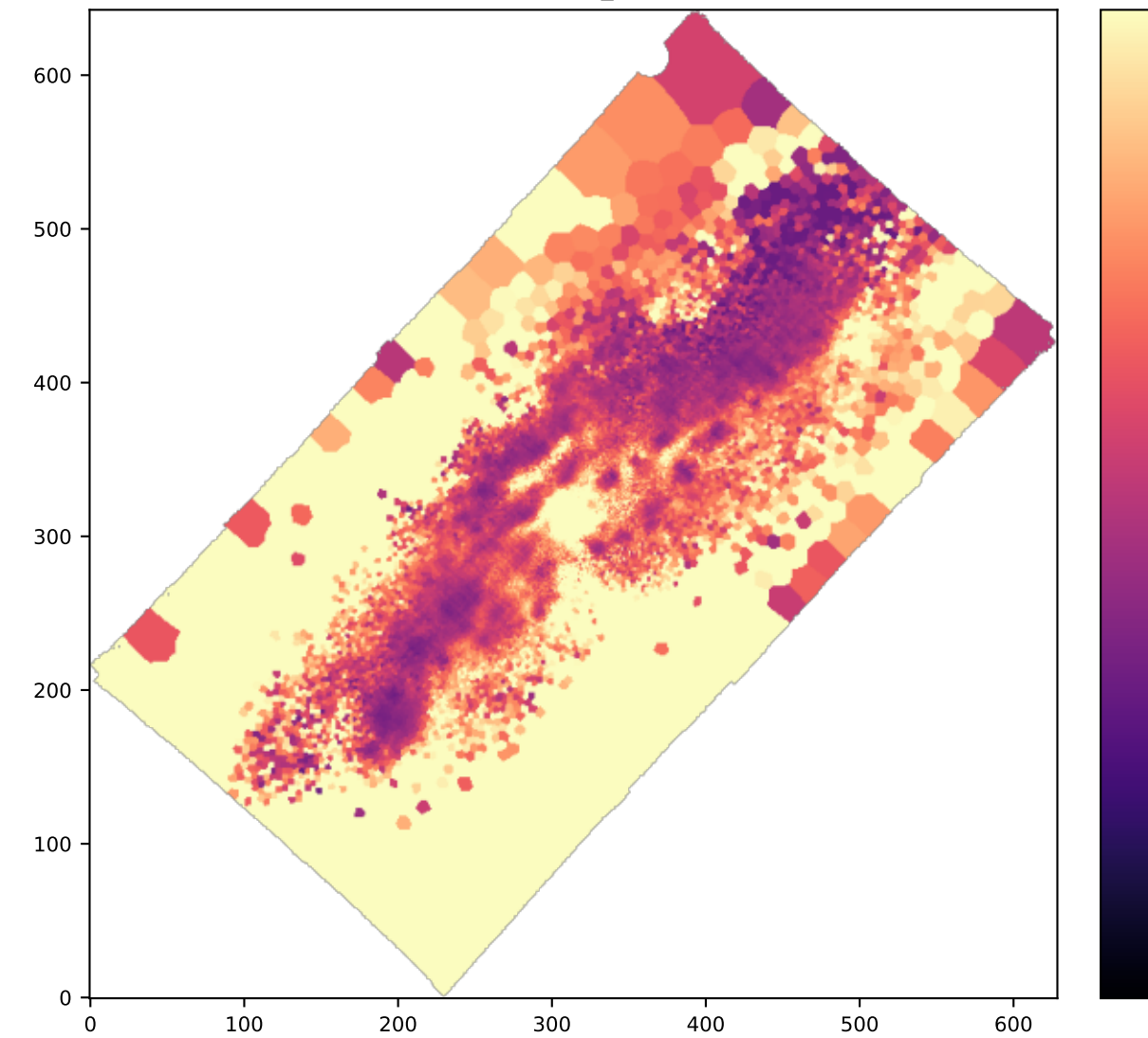
BIN HB4861_SIGMA
