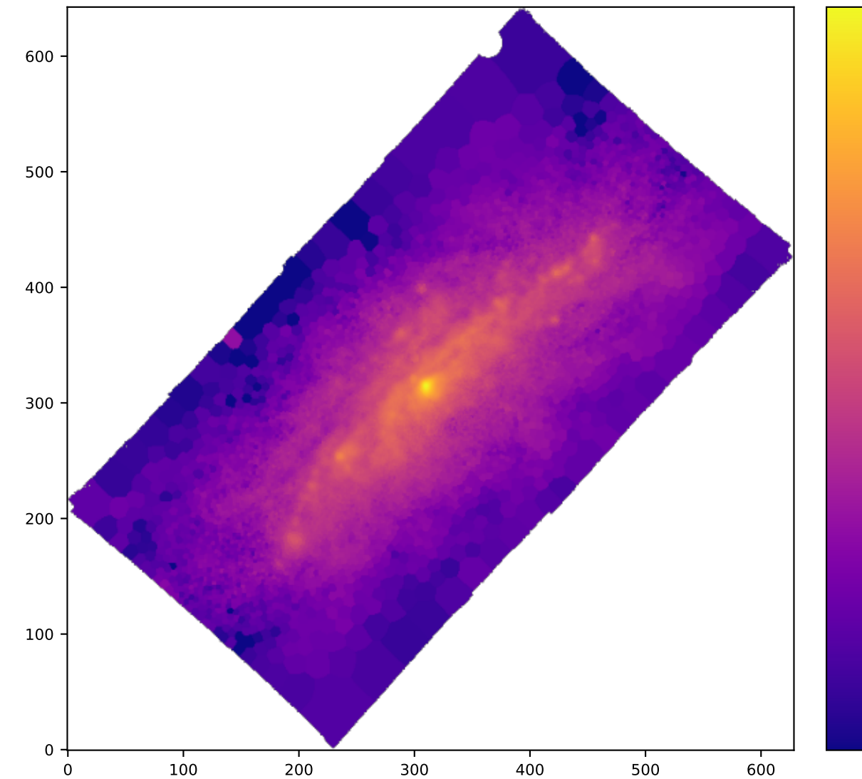
BIN SII6716_SIGMA
