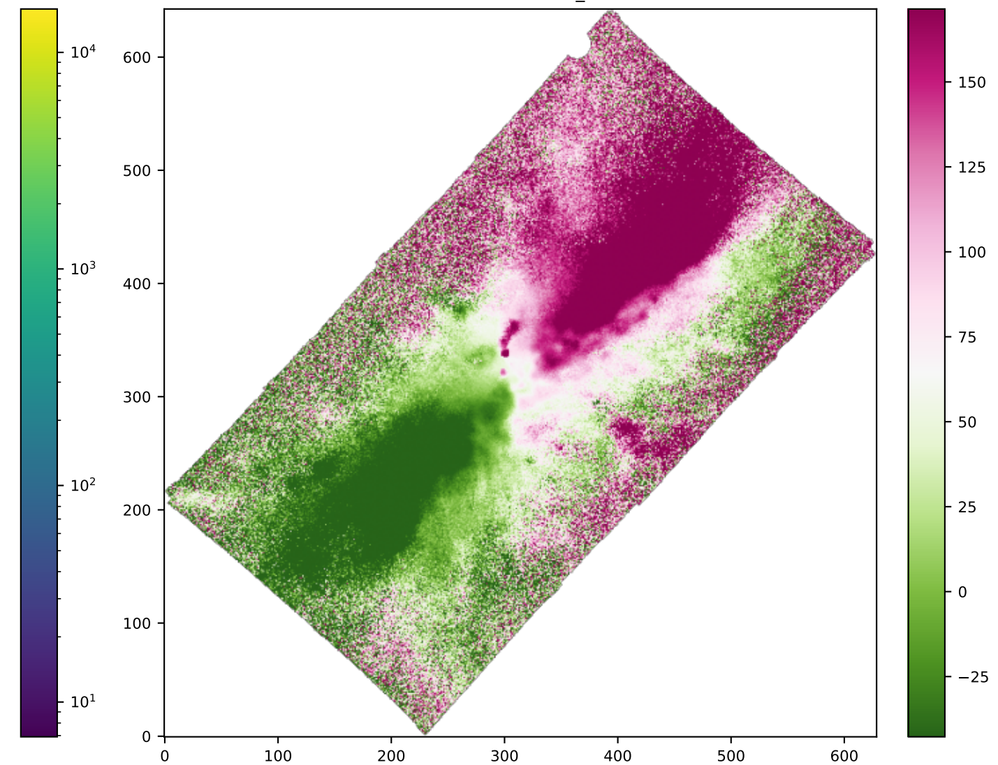
SPAXELS NII6583_VEL
