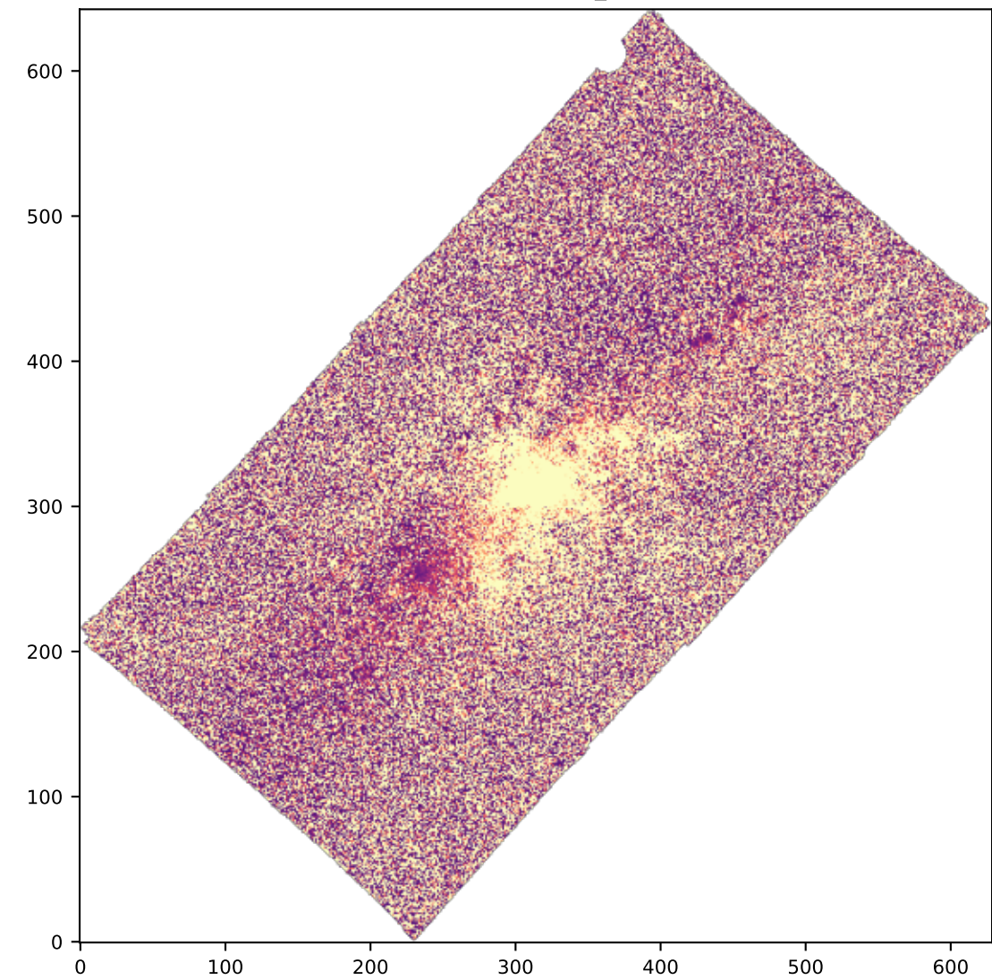
SPAXELS OIII5006_SIGMA
