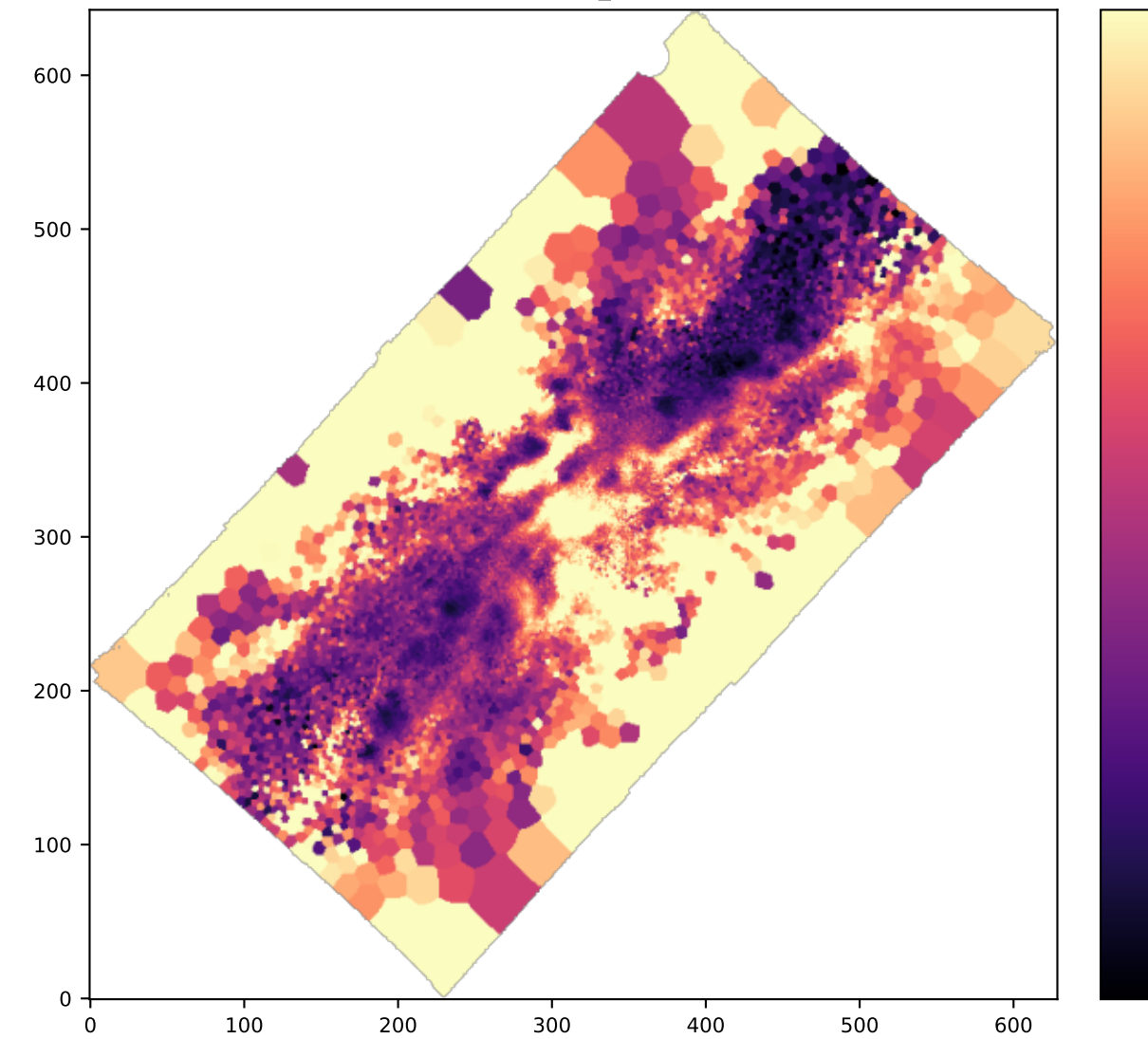
BIN SII6716_SIGMA
