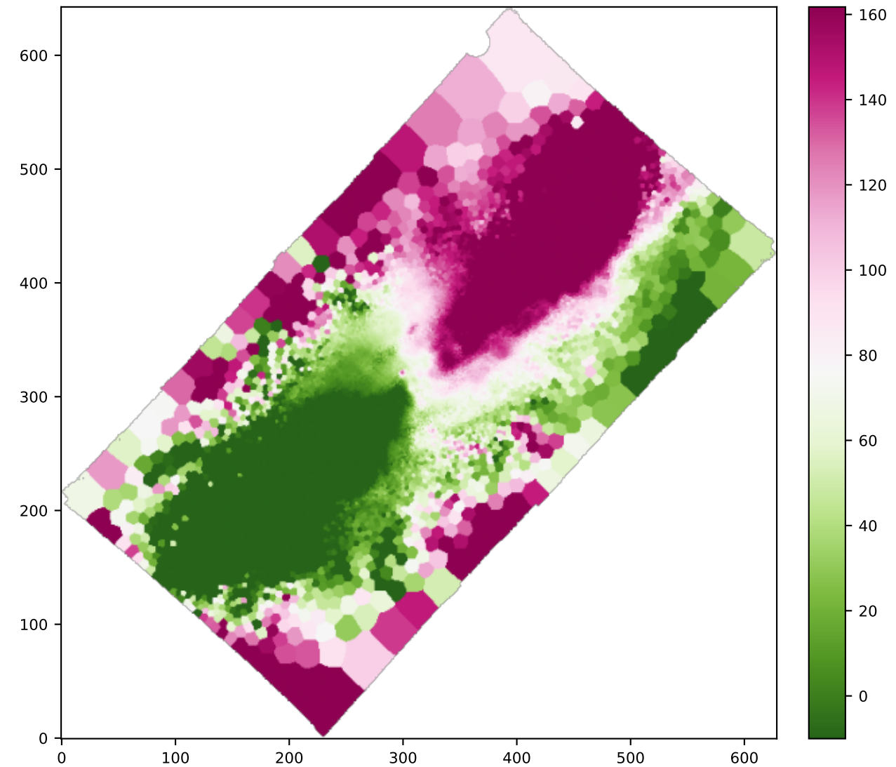
BIN HA6562_VEL
