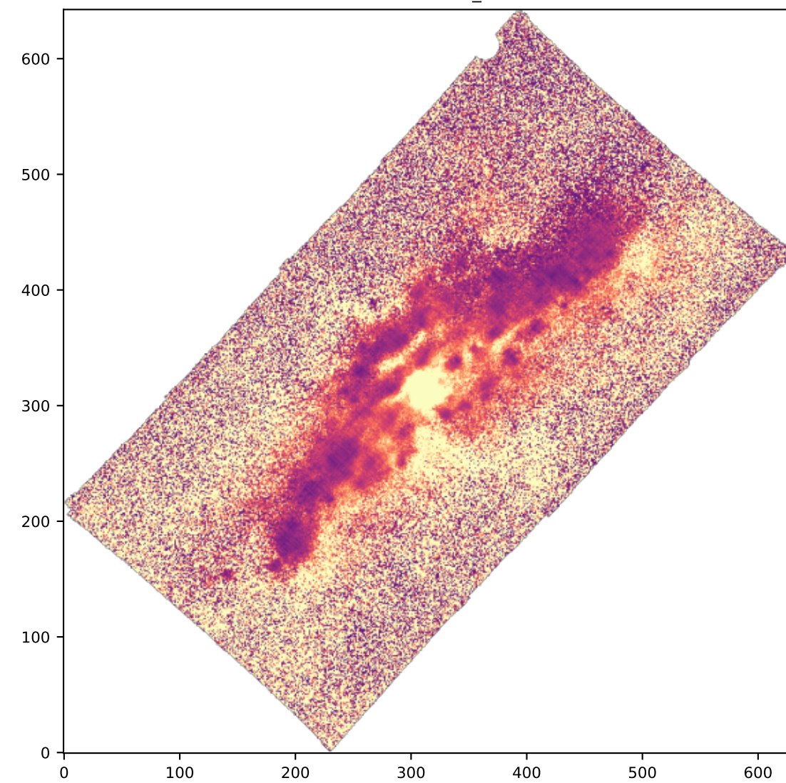
SPAXELS HB4861_SIGMA
