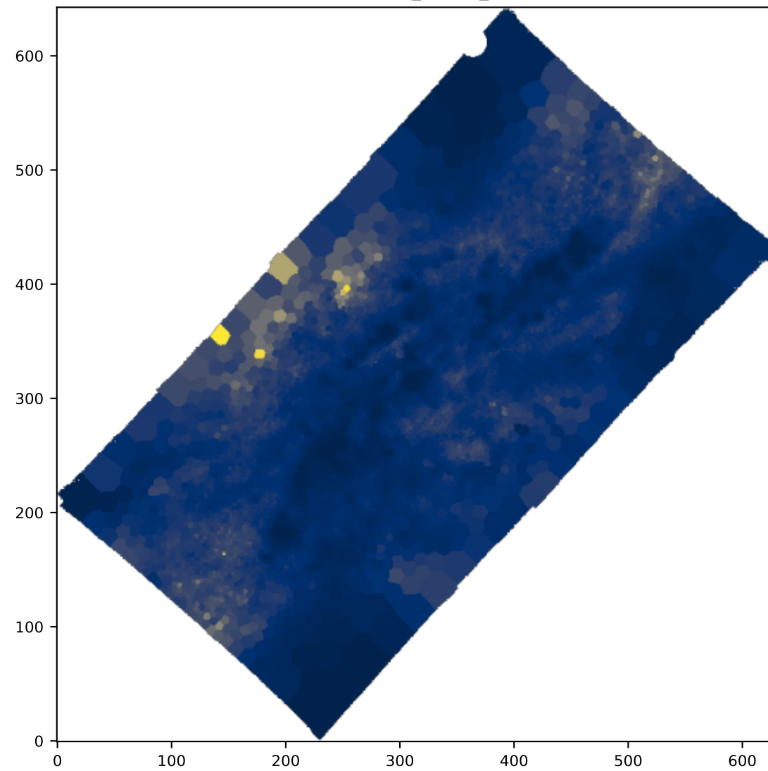
BIN SII6716_SIGMA_ERR
