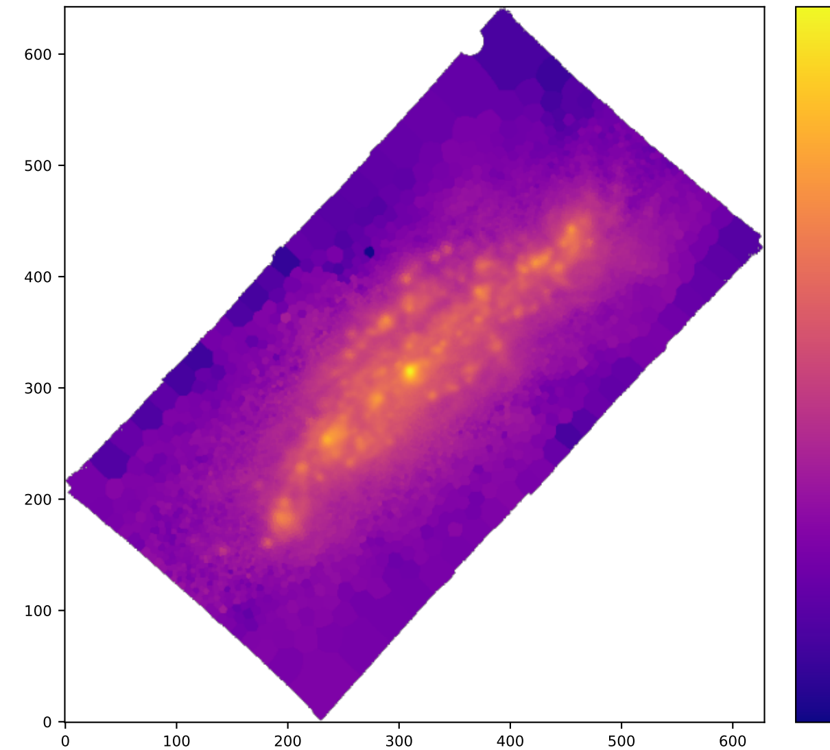
BIN HA6562_SIGMA
