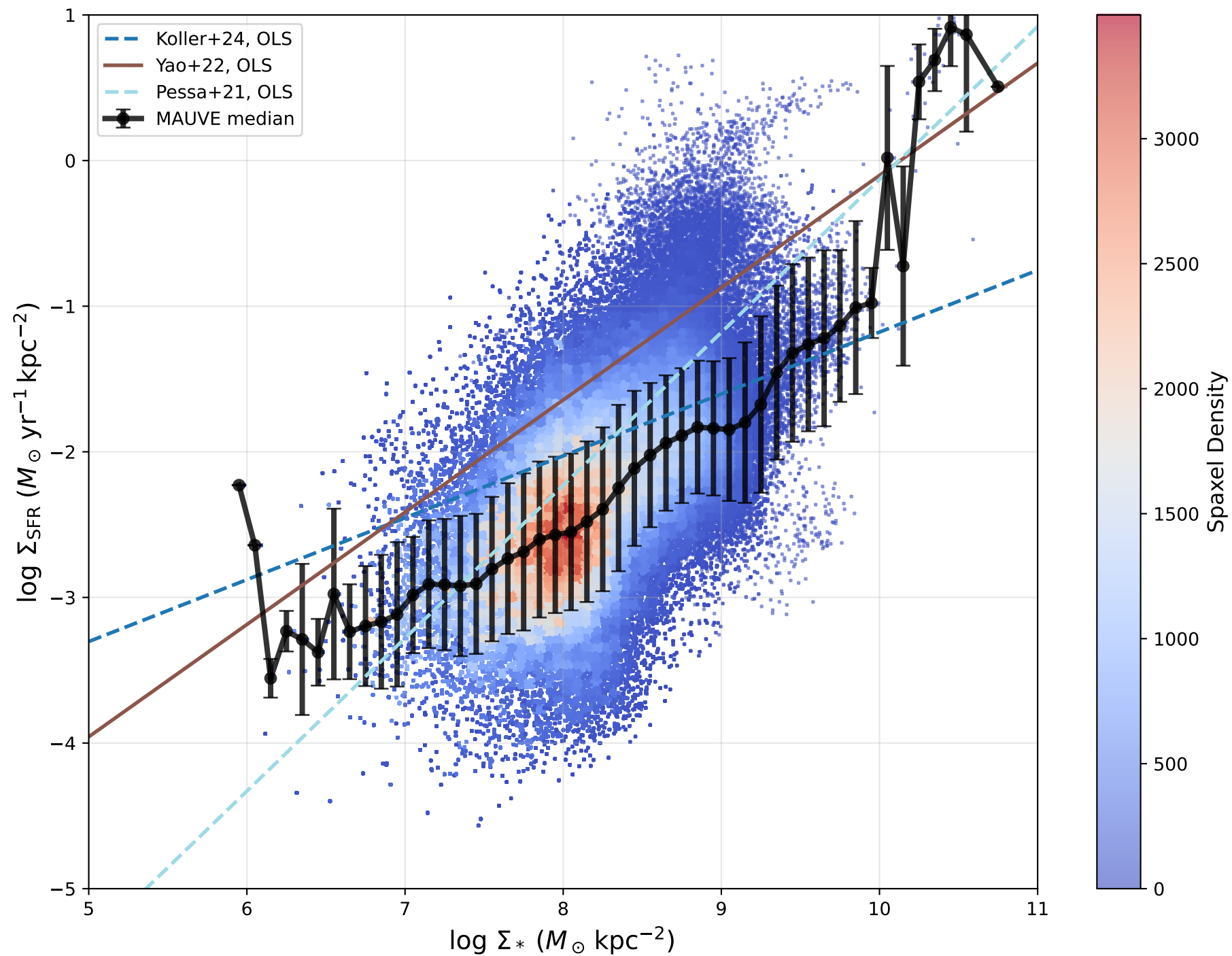
14 MAUVE galaxies: Combined resolved Star Formation Main Sequence
