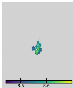
[O/H] (O3N2-M13, HII)
