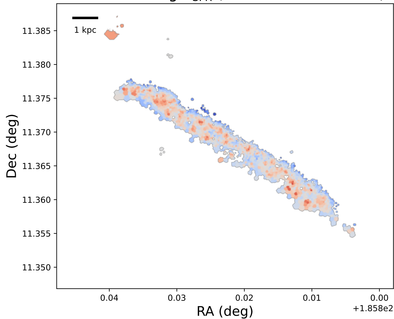
NGC4330: \Delta \log \Sigma_{\text{SFR}} (offset from bin mean)
