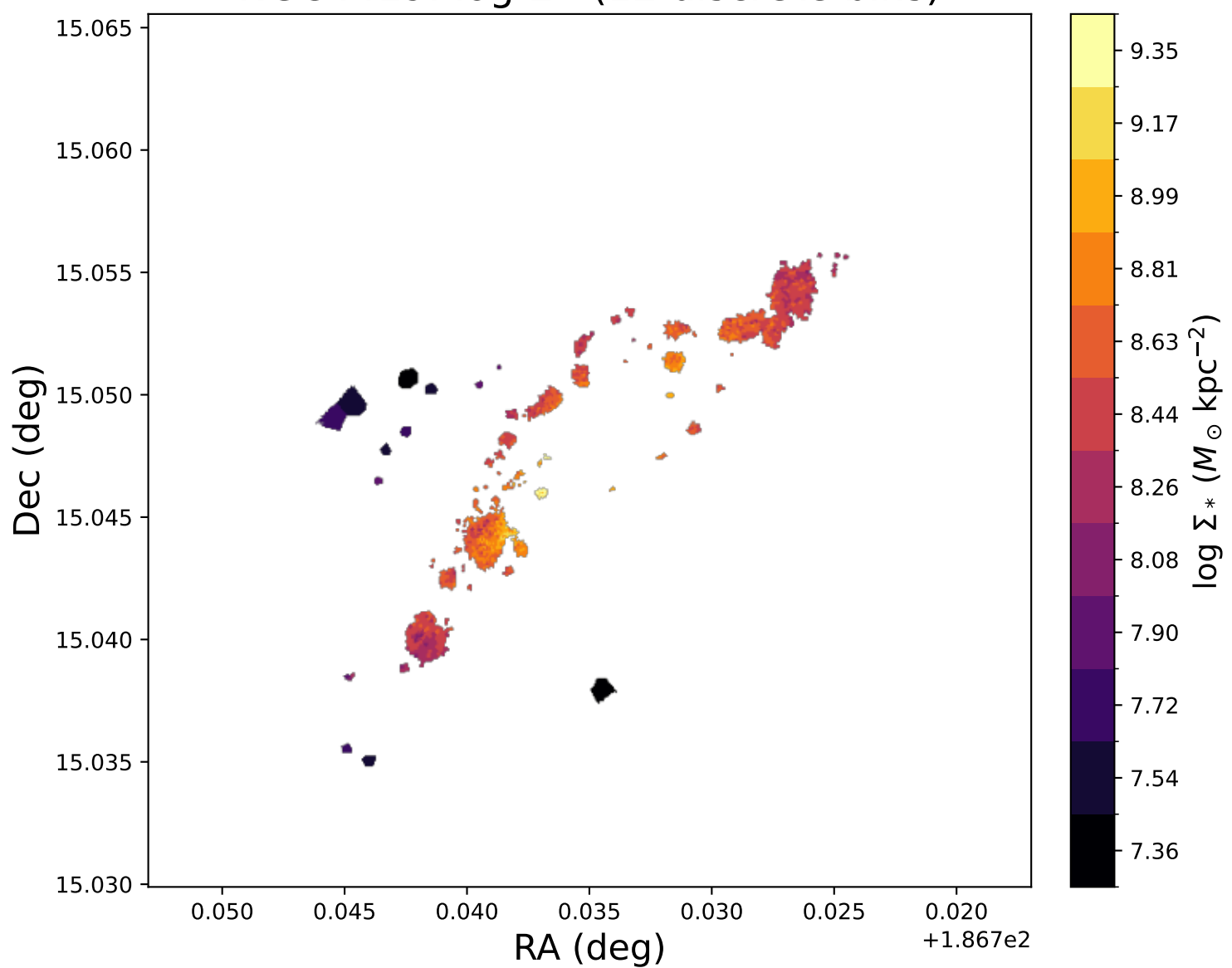
NGC4419: \log \Sigma_* (12 discrete bins)
