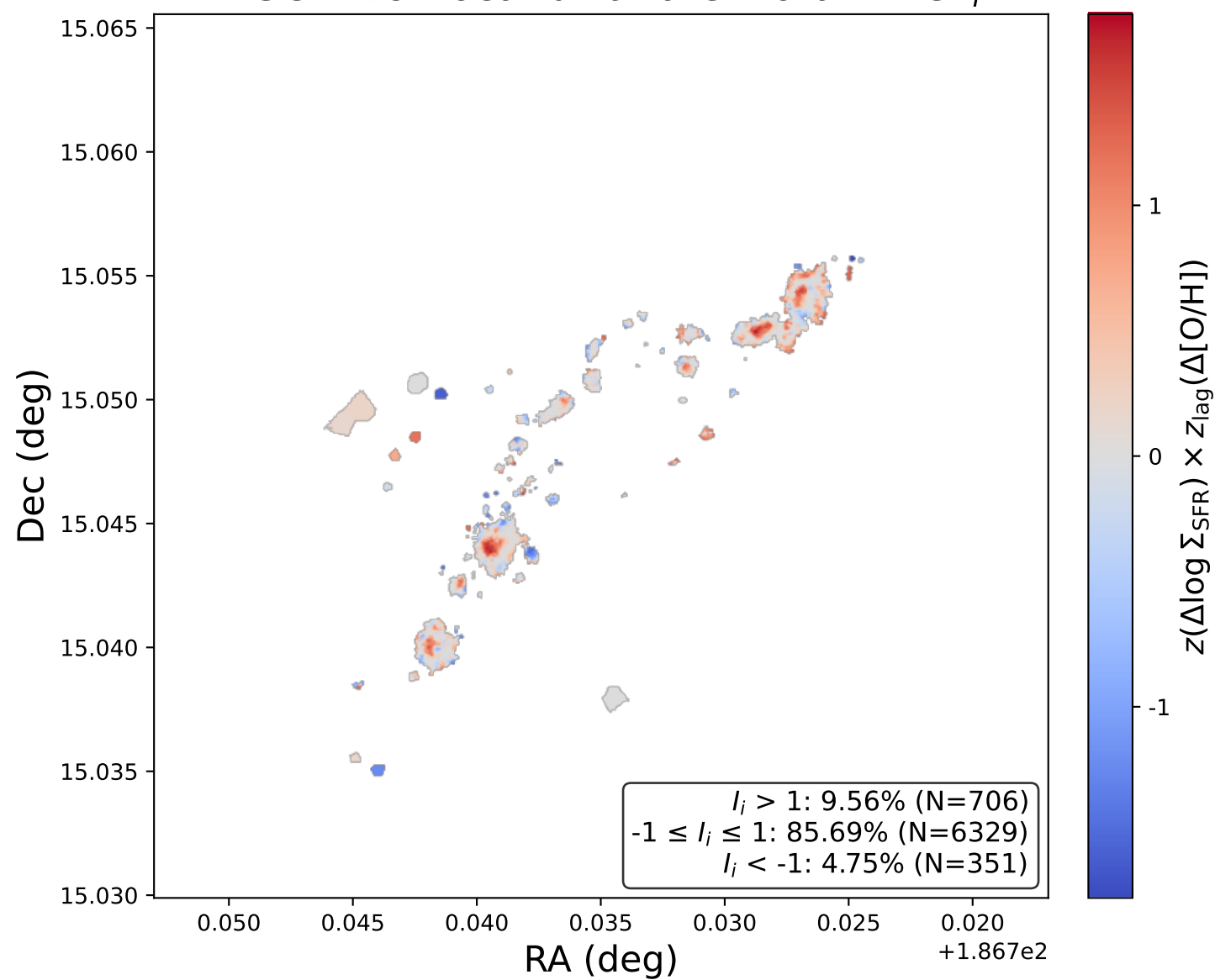
NGC4419: local bivariate Moran-like I_i
