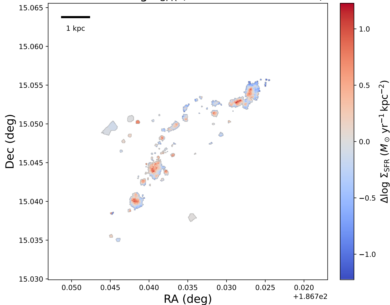
NGC4419: \Delta \log \Sigma_{\text{SFR}} (offset from bin mean)
