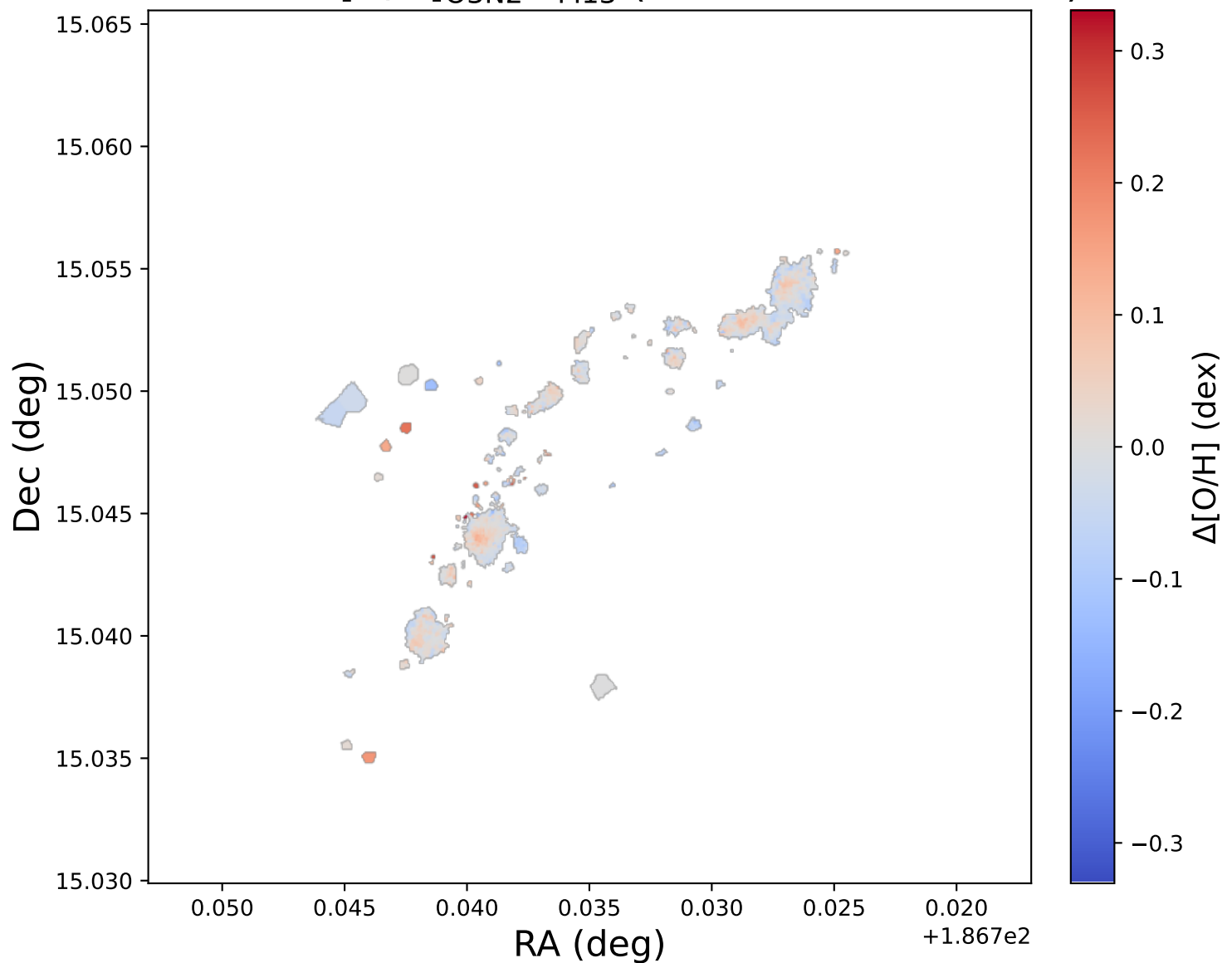
NGC4419: \Delta[\text{O}/\text{H}]_{\text{O3N2} - \text{M13}} (offset from bin mean)
