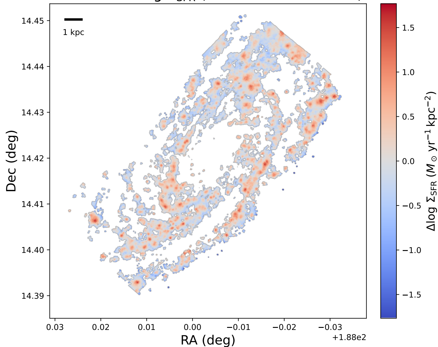
NGC4501: \Delta \log \Sigma_{\text{SFR}} (offset from bin mean)
