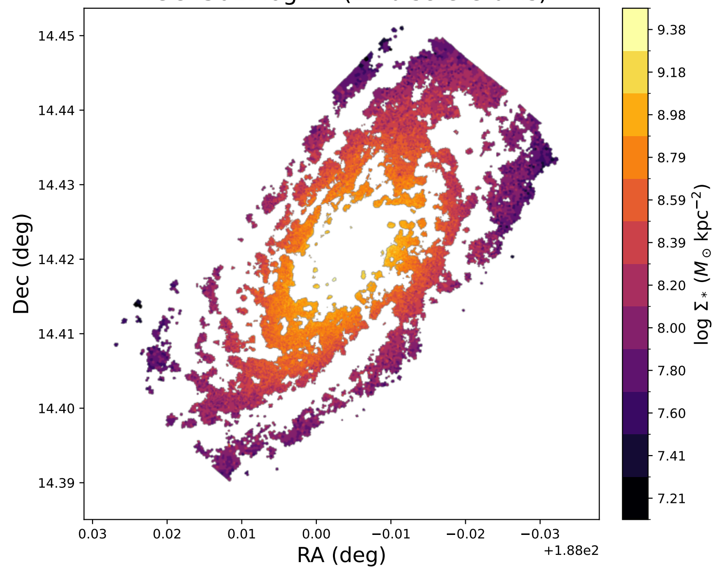
NGC4501: \log \Sigma_* (12 discrete bins)
