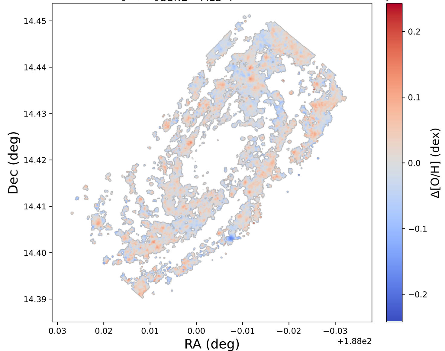
NGC4501: \Delta[\text{O}/\text{H}]_{\text{O3N2} - \text{M13}} (offset from bin mean)
