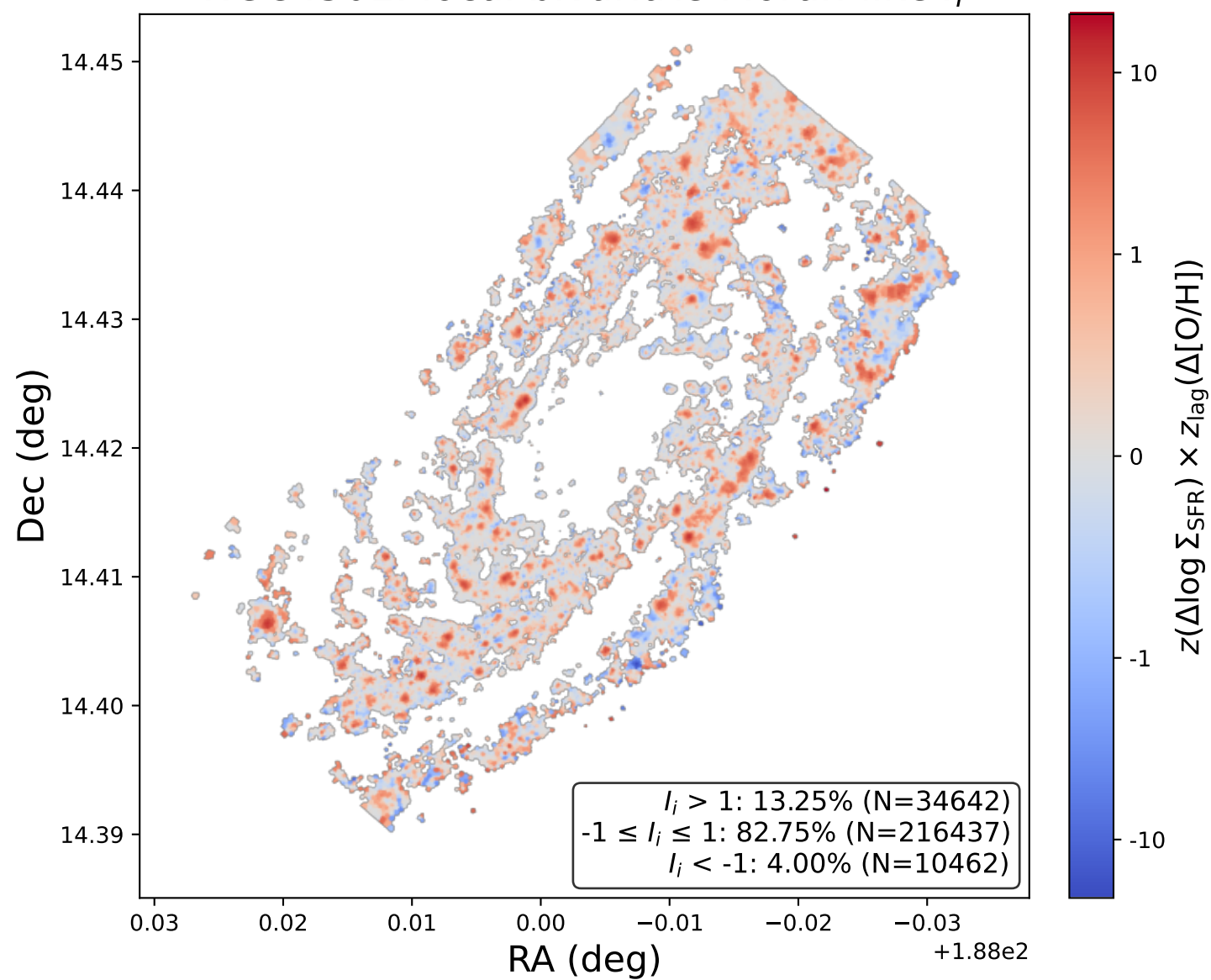
NGC4501: local bivariate Moran-like I_i
