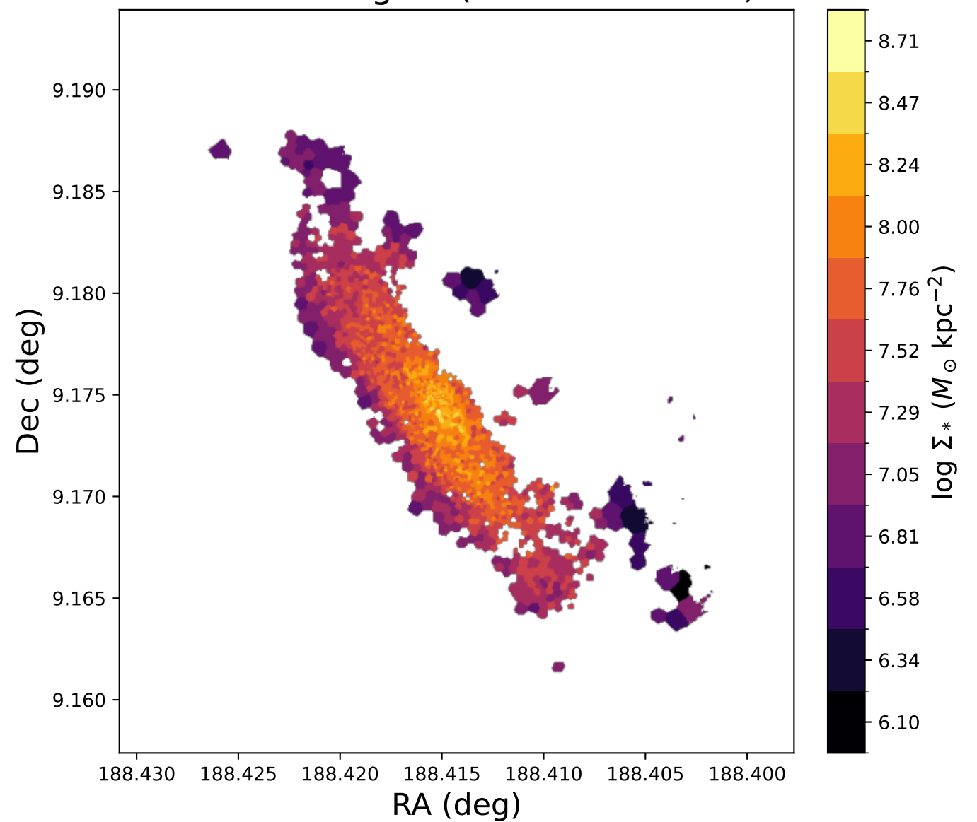
NGC4522: \log \Sigma_{*} (12 discrete bins)
