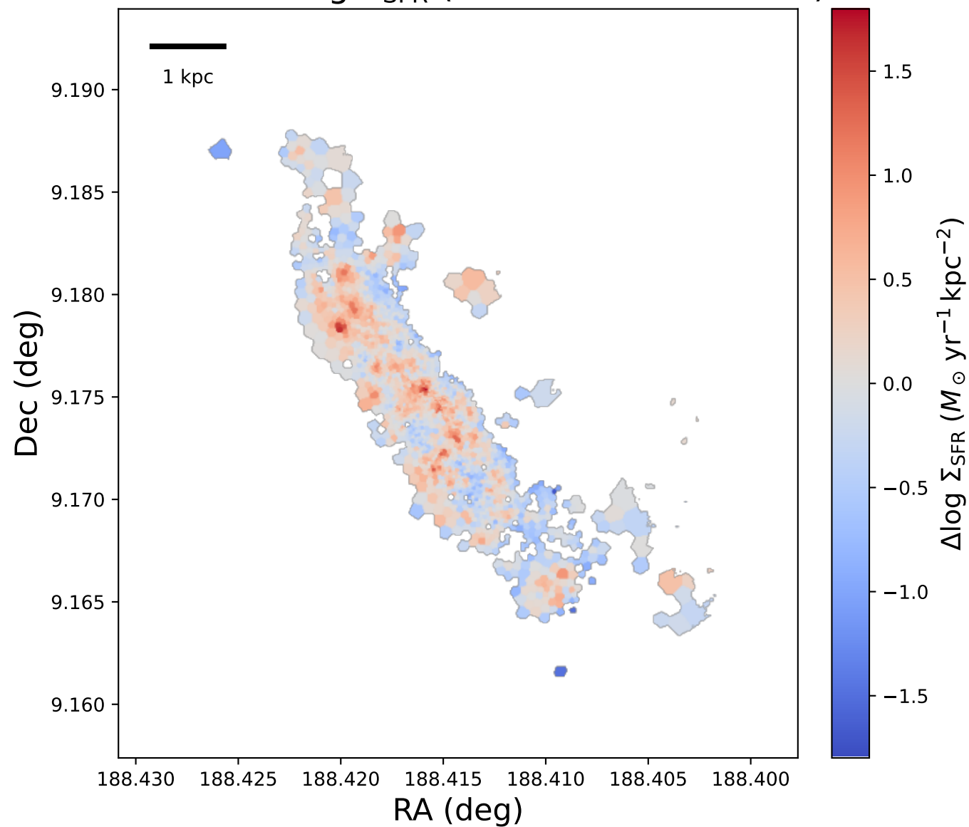
NGC4522: \Delta \log \Sigma_{\text{SFR}} (offset from bin mean)
