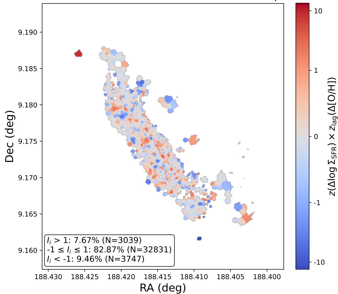
NGC4522: local bivariate Moran-like I_i
