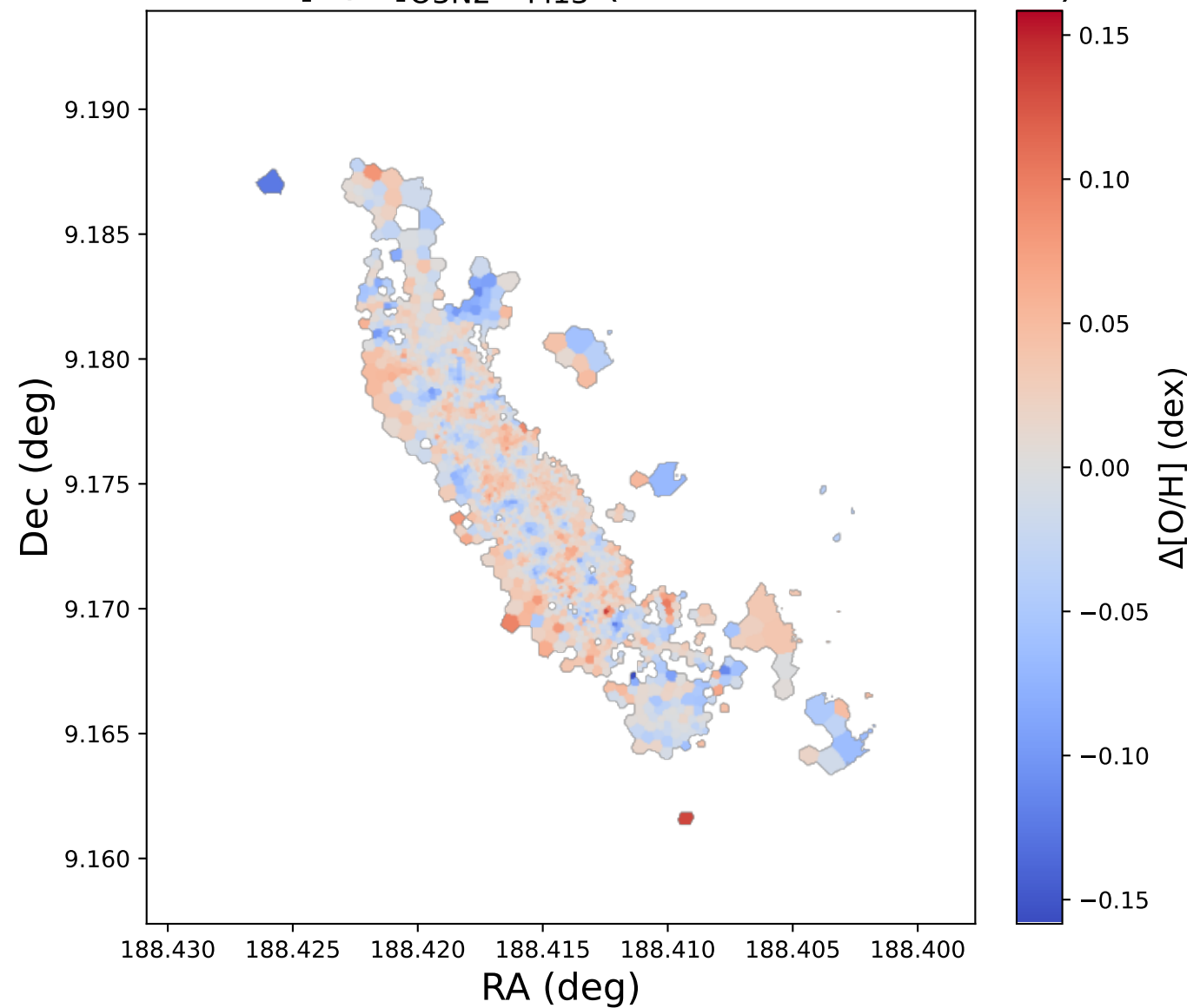
NGC4522: \Delta[\text{O}/\text{H}]_{\text{O3N2} - \text{M13}} (offset from bin mean)
