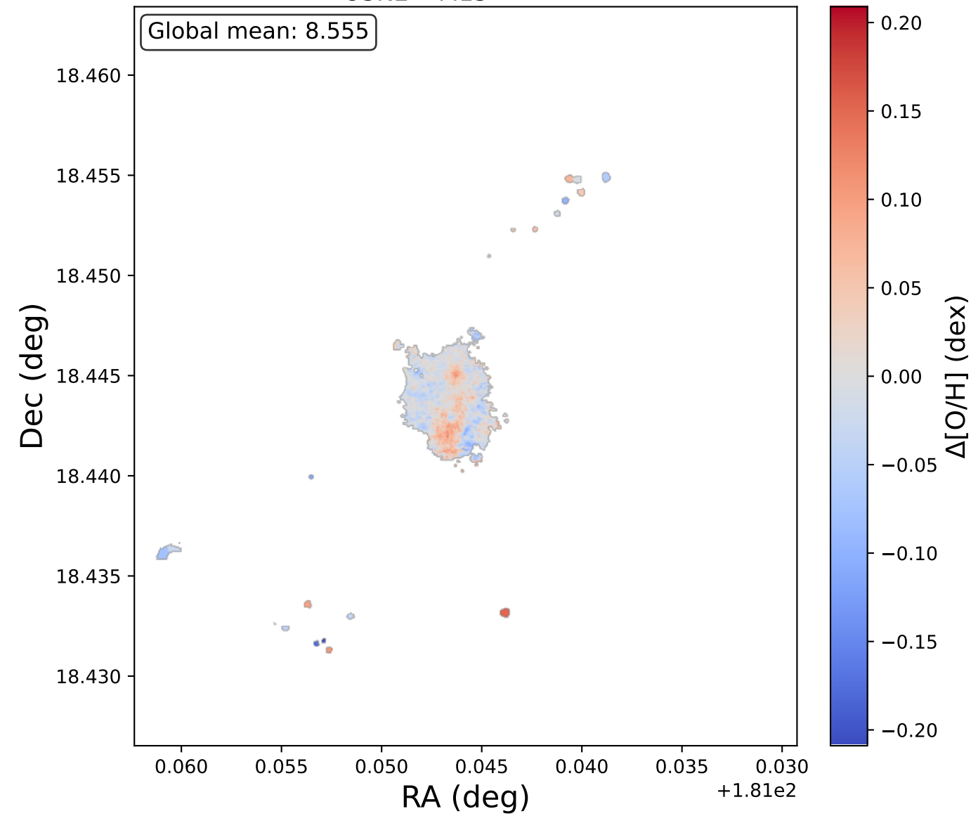
NGC4064: \Delta[\text{O}/\text{H}]_{\text{O3N2} - \text{M13}} (offset from bin mean)
