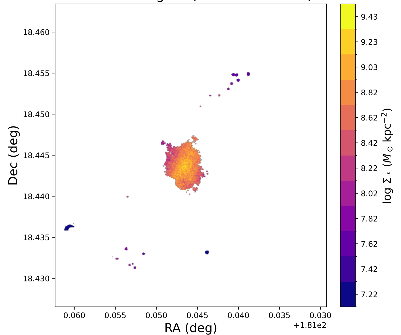
NGC4064: \log \Sigma_{*} (12 discrete bins)
