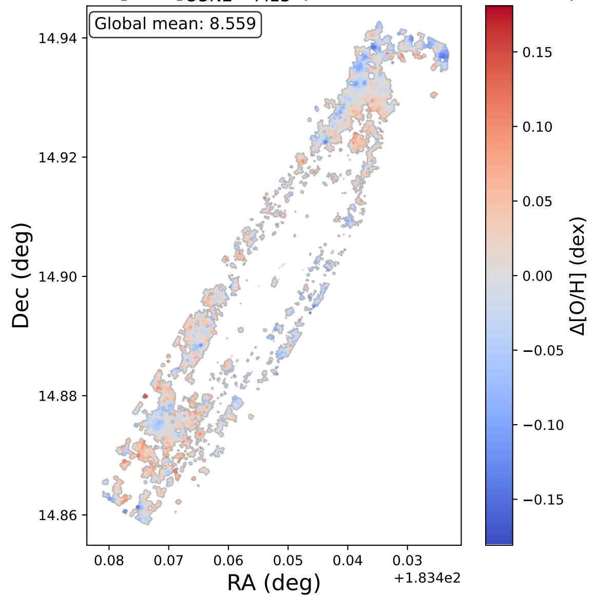
NGC4192: \Delta[\text{O}/\text{H}]_{\text{O3N2-M13}} (offset from bin mean)
