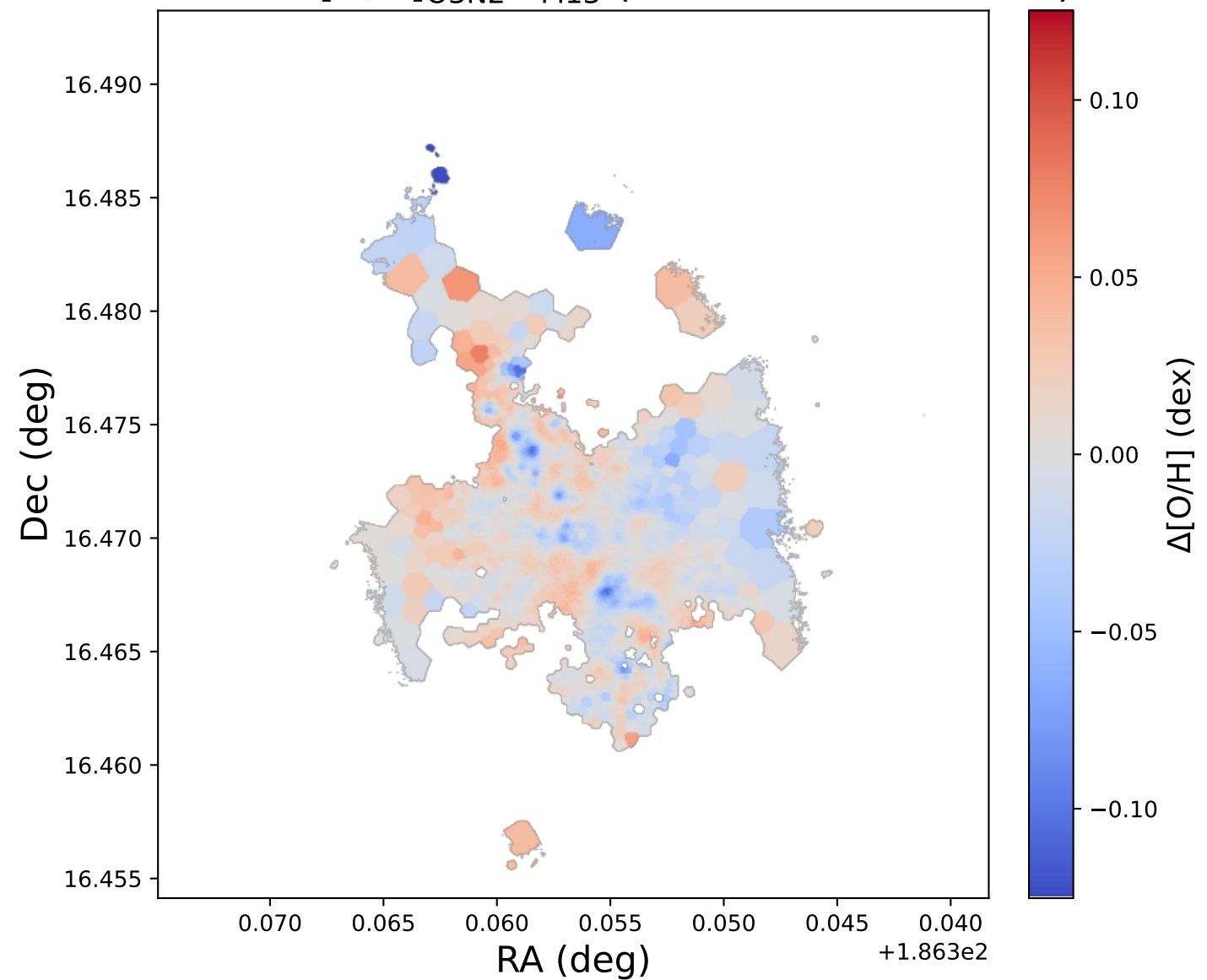
NGC4383: \Delta[\text{O}/\text{H}]_{\text{O3N2} - \text{M13}} (offset from bin mean)
