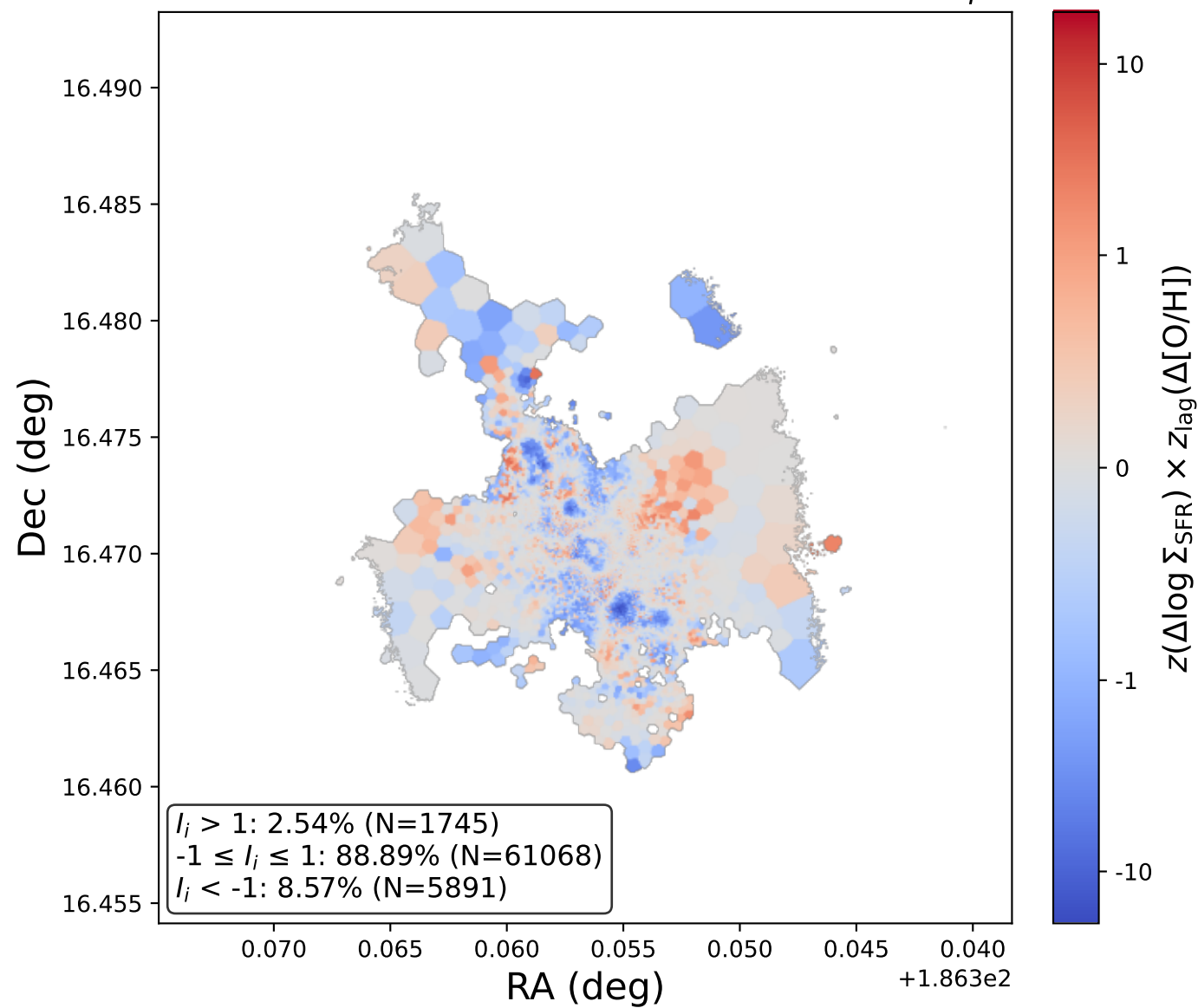
NGC4383: local bivariate Moran-like I_i
