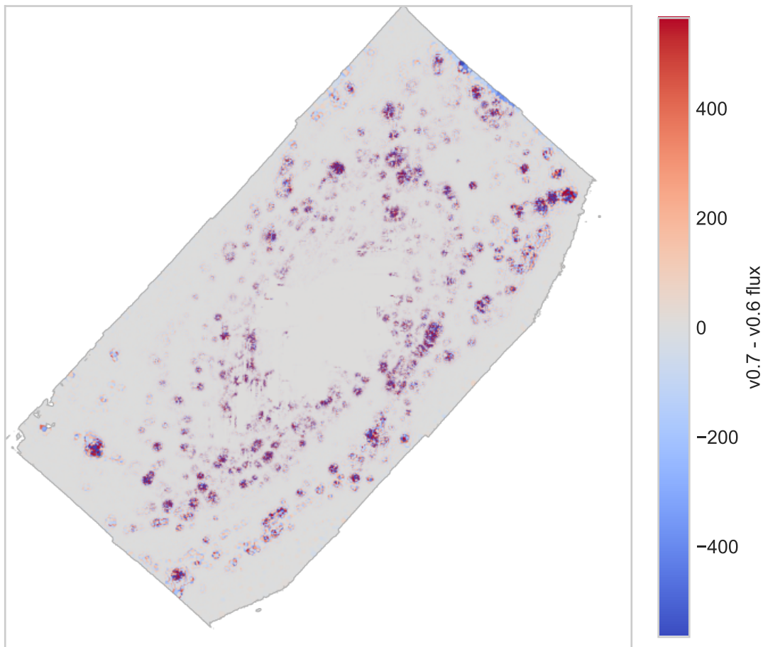
DIFF (v0.7 - v0.6): GAS HA6562_FLUX
