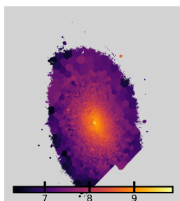
NGC4383: \log \Sigma_*
