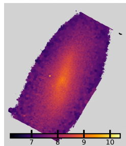
NGC4192: \log \Sigma_*
