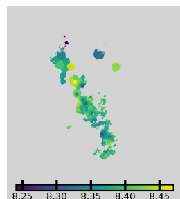
[O/H] (O3N2-M13, HII)
