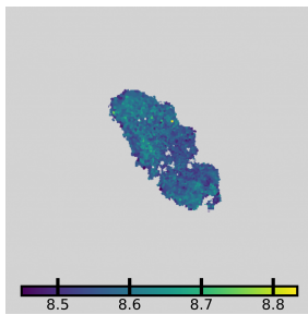
[O/H] (O3N2-M13, HII)
