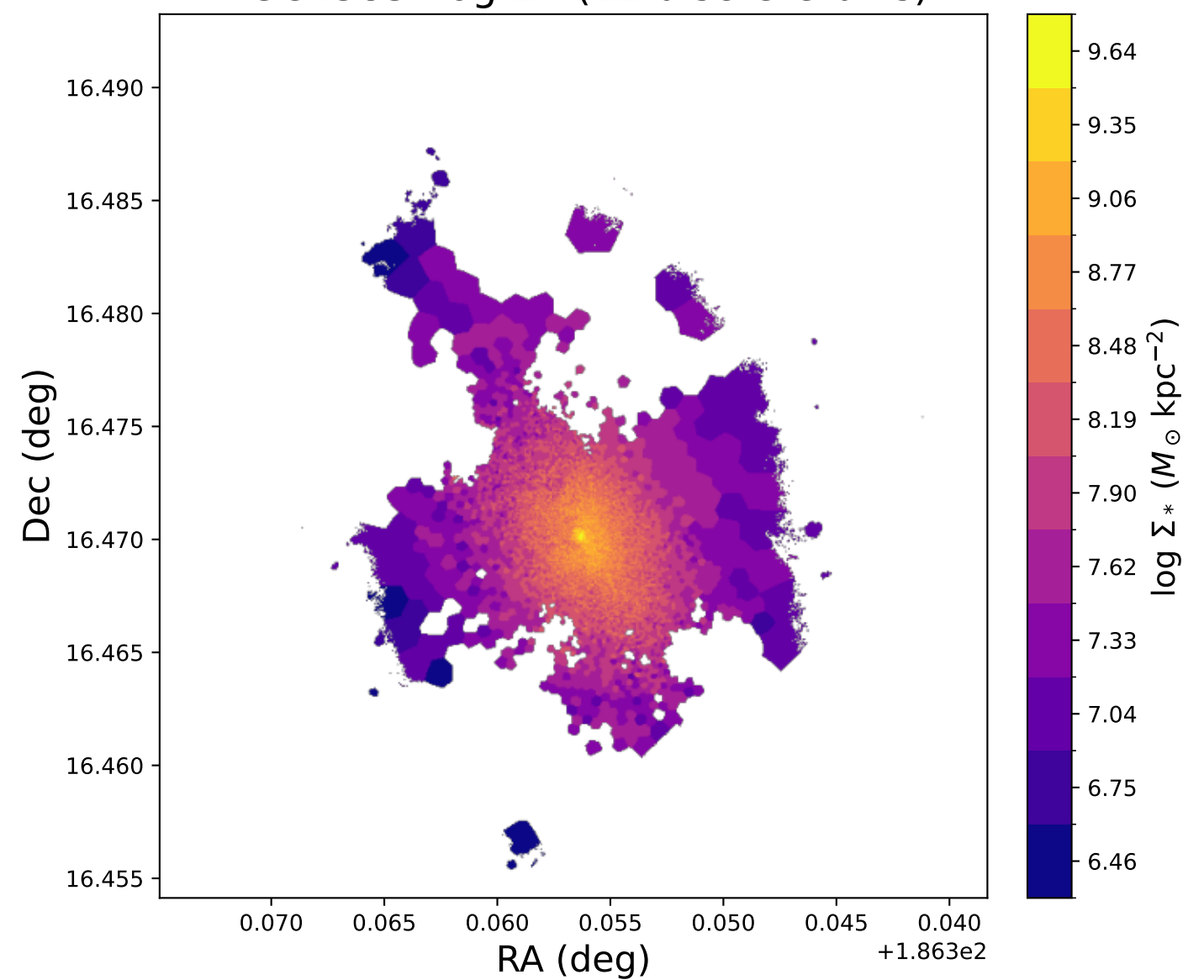
NGC4383: \log \Sigma_{*} (12 discrete bins)
