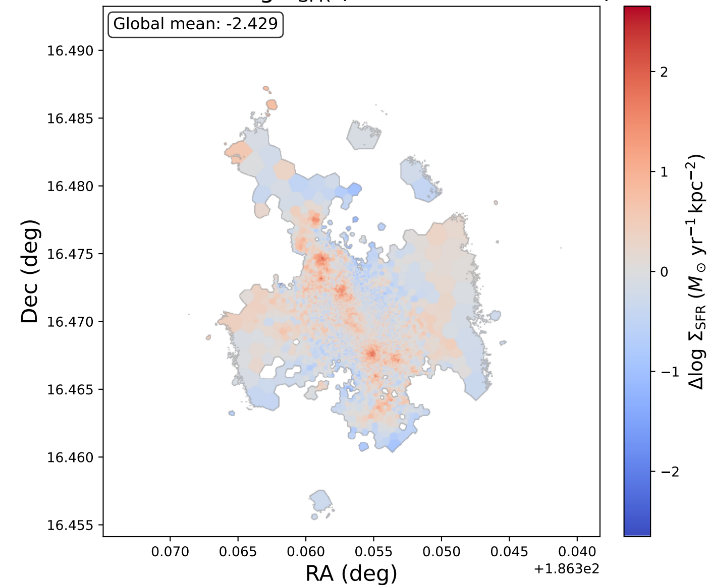
NGC4383: \Delta \log \Sigma_{\text{SFR}} (offset from bin mean)
