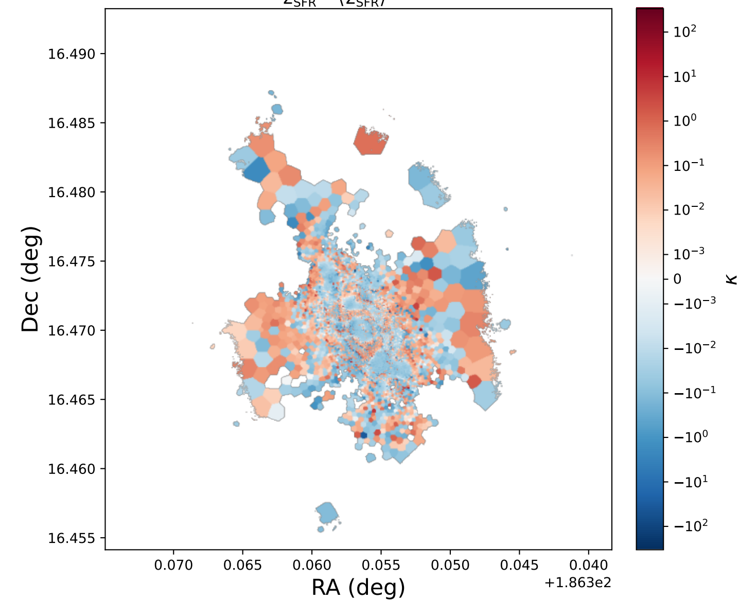
NGC4383: Slope \kappa = \frac{[\text{O}/\text{H}] - \langle [\text{O}/\text{H}] \rangle}{\Sigma_{\text{SFR}} - \langle \Sigma_{\text{SFR}} \rangle} (O3N2-M13, HII regions)
