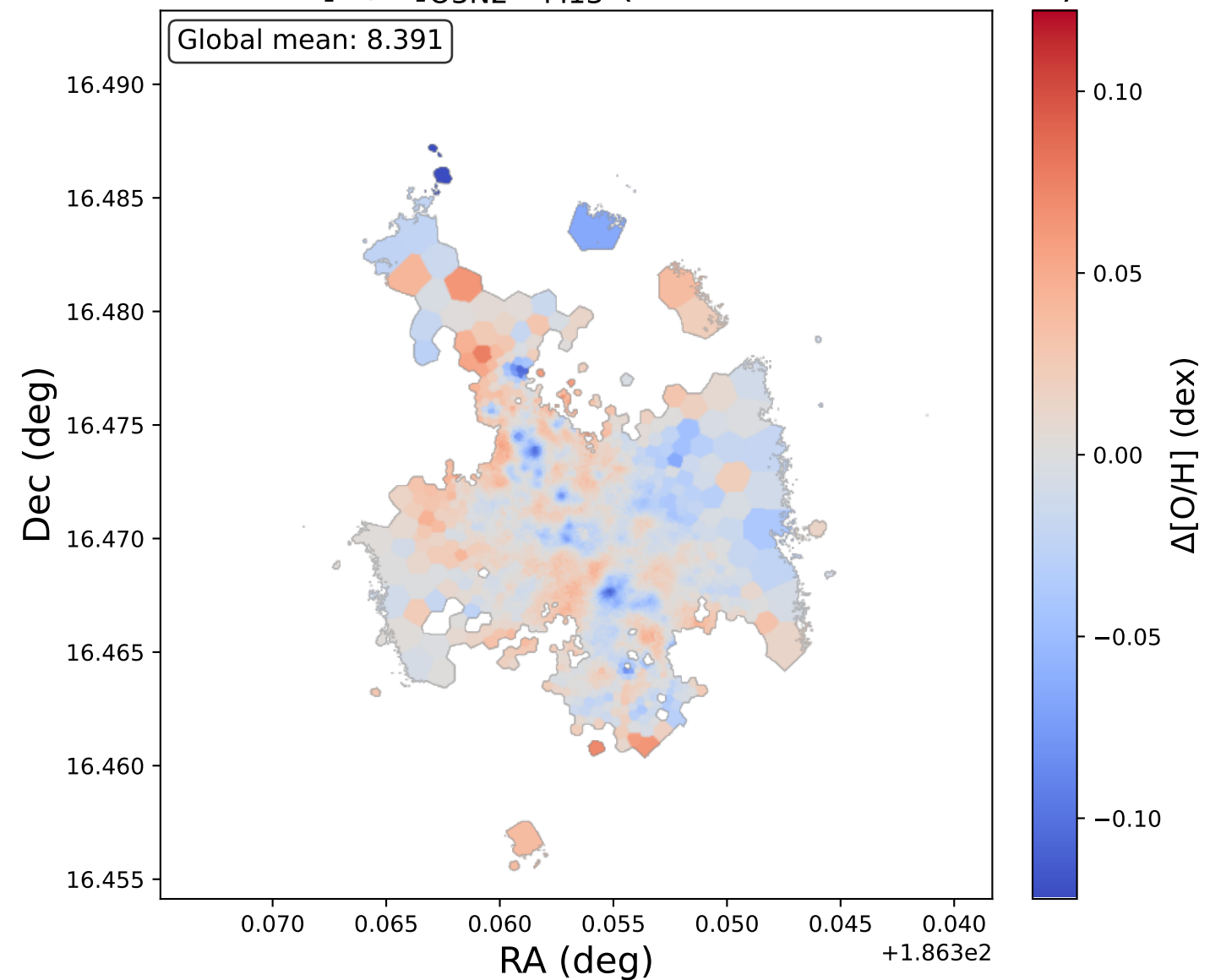
NGC4383: \Delta[\text{O}/\text{H}]_{\text{O3N2-M13}} (offset from bin mean)
