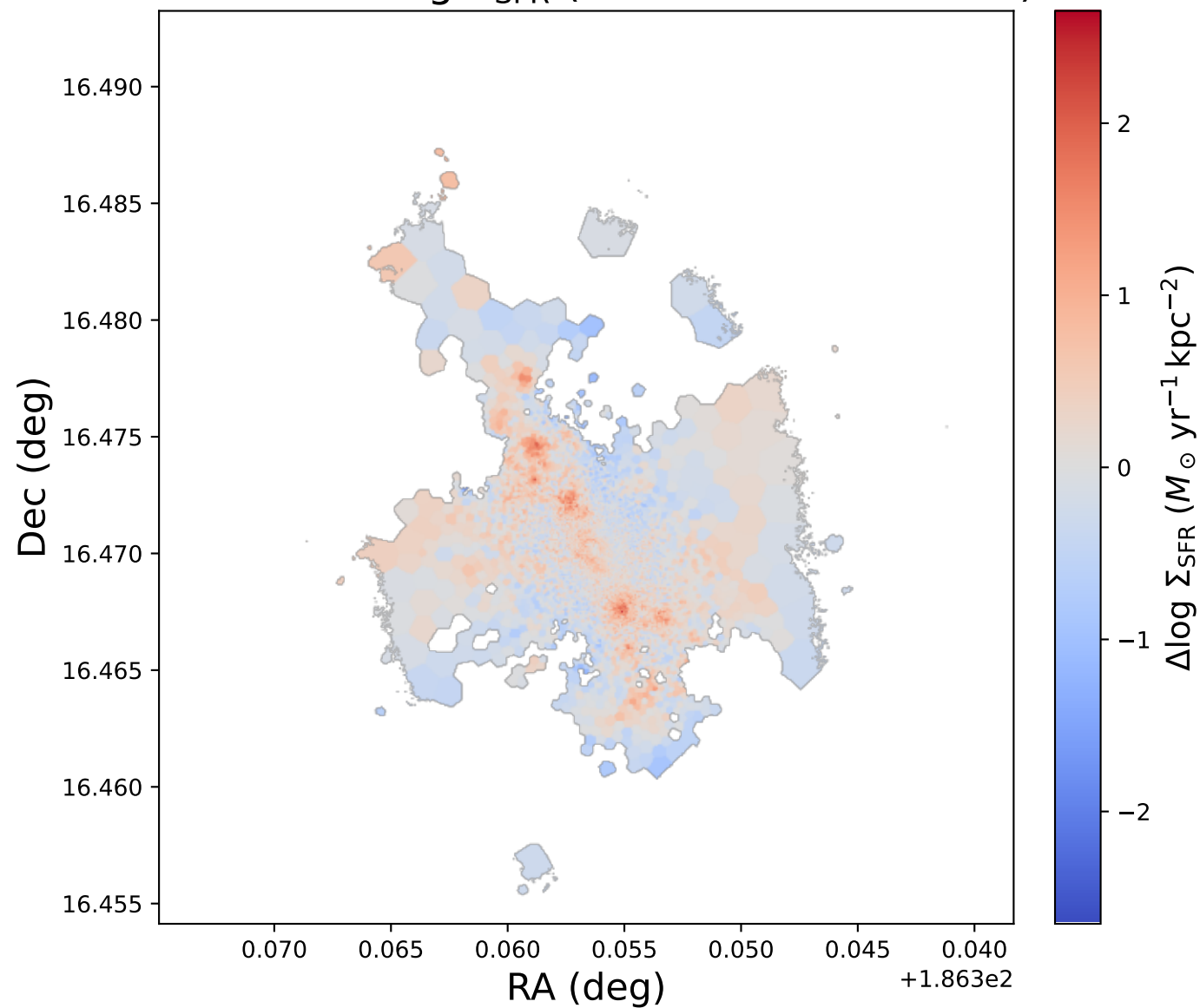
NGC4383: \Delta \log \Sigma_{\text{SFR}} (offset from bin mean)
