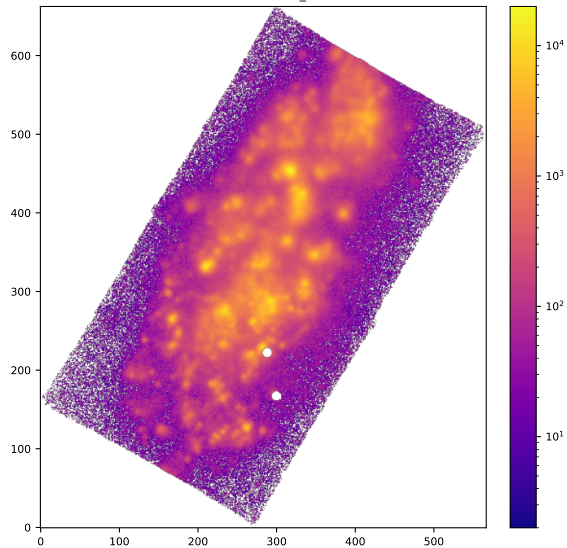
SPAXELS HB4861_SIGMA
