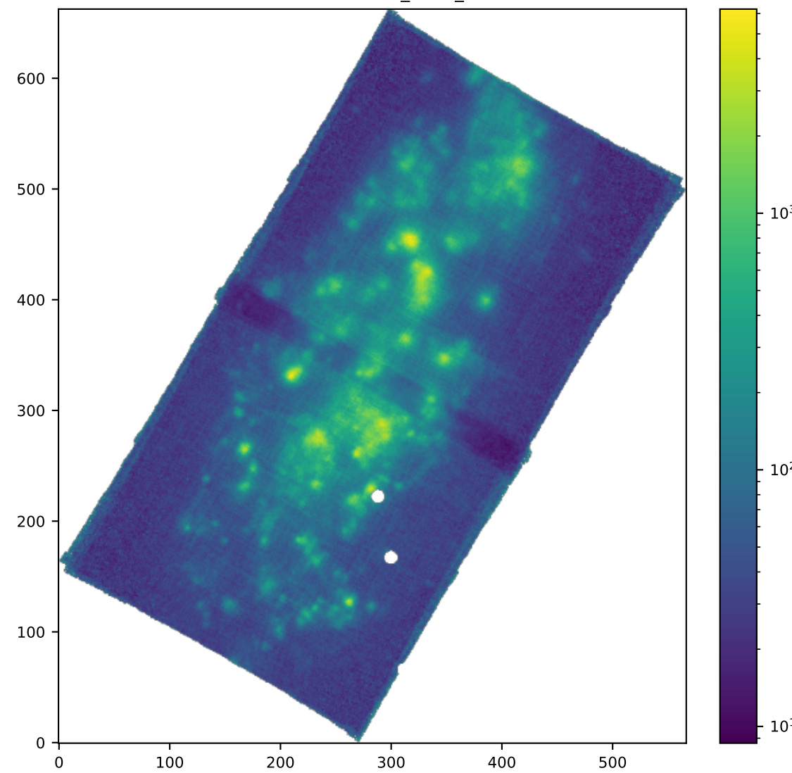
SPAXELS HA6562_SIGMA_ERR
