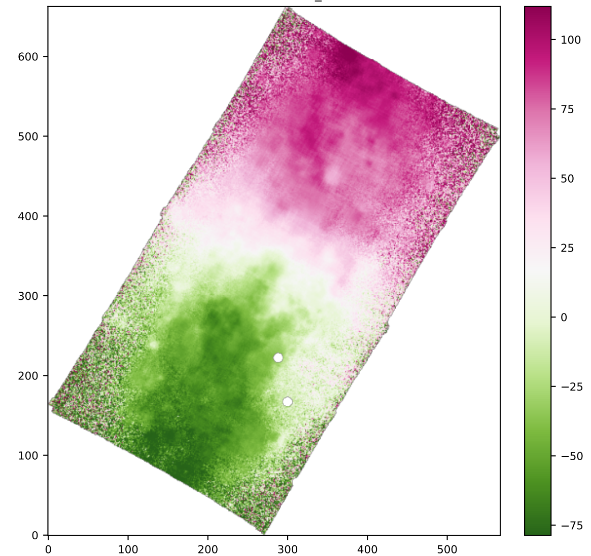
SPAXELS HB4861_VEL
