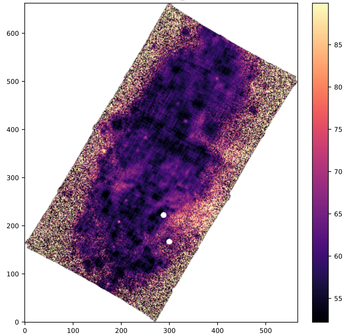
SPAXELS HA6562_SIGMA
