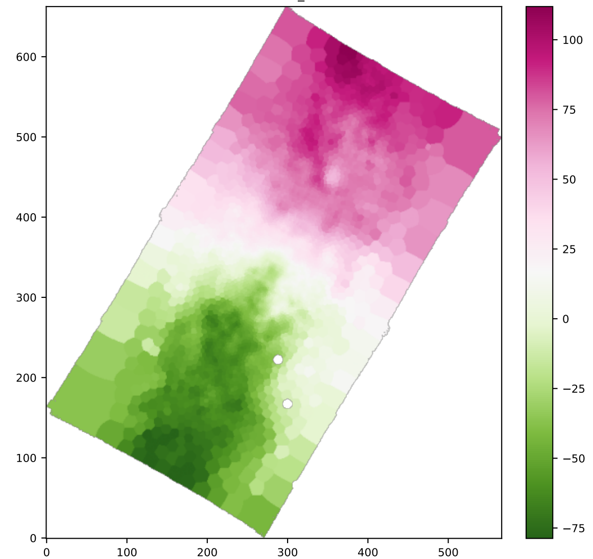
BIN HA6562_VEL
