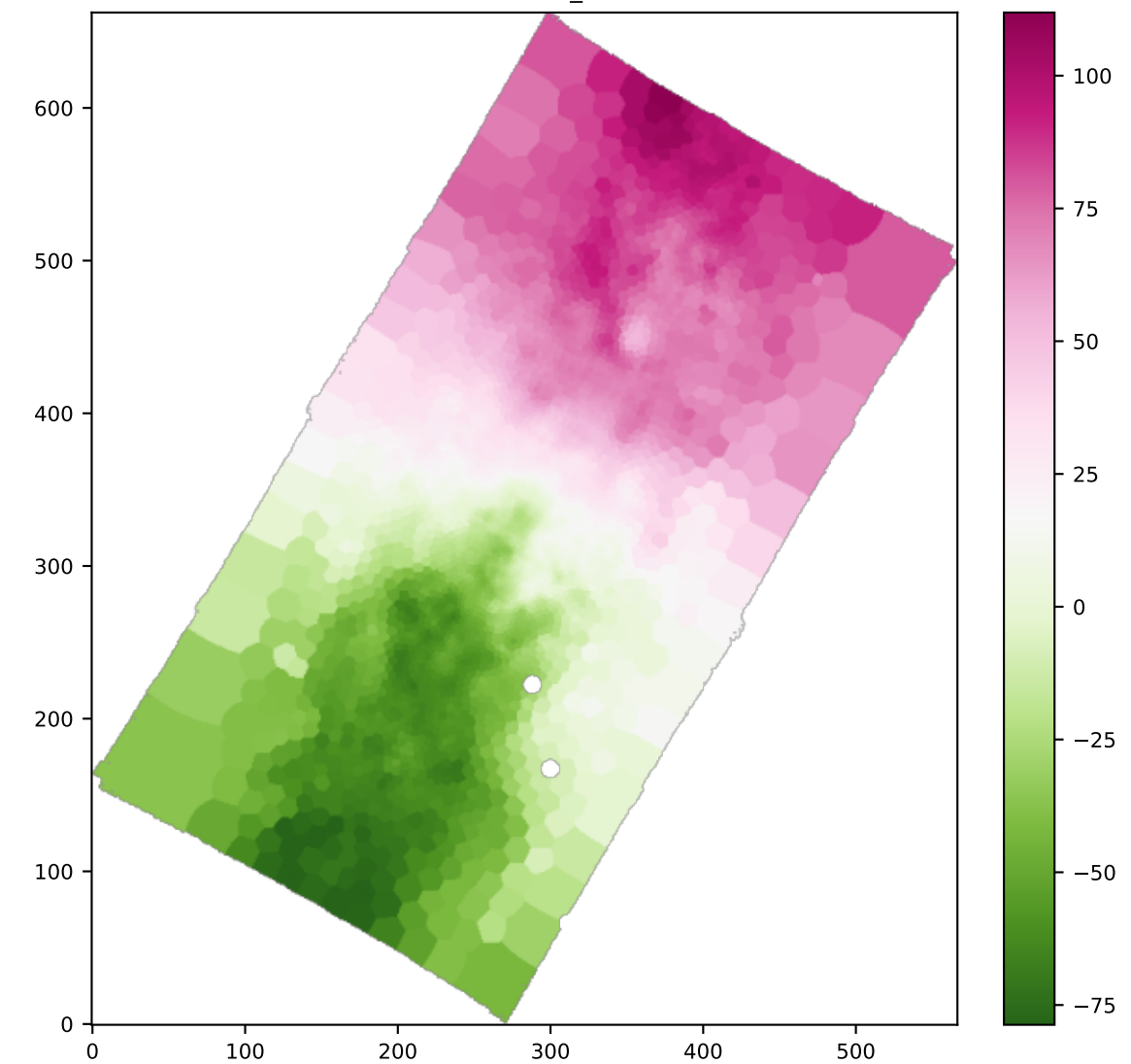
BIN HB4861_VEL
