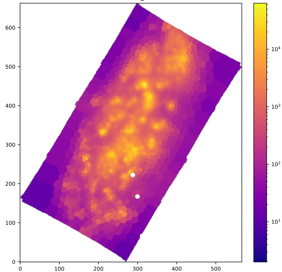
BIN HA6562_SIGMA
