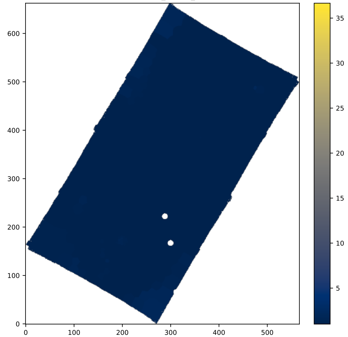
BIN HB4861_SIGMA_ERR
