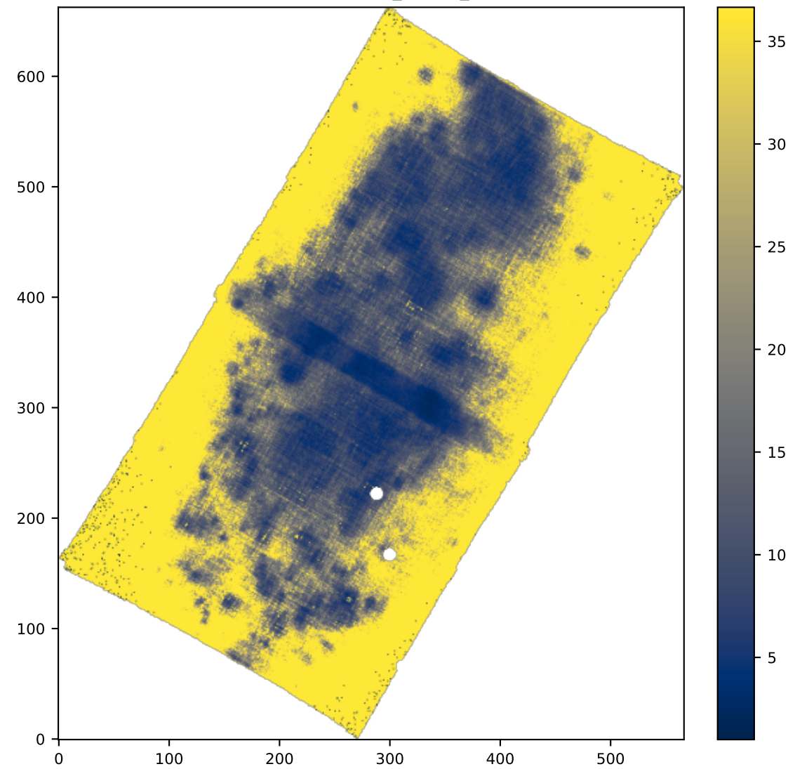
SPAXELS HB4861_SIGMA_ERR
