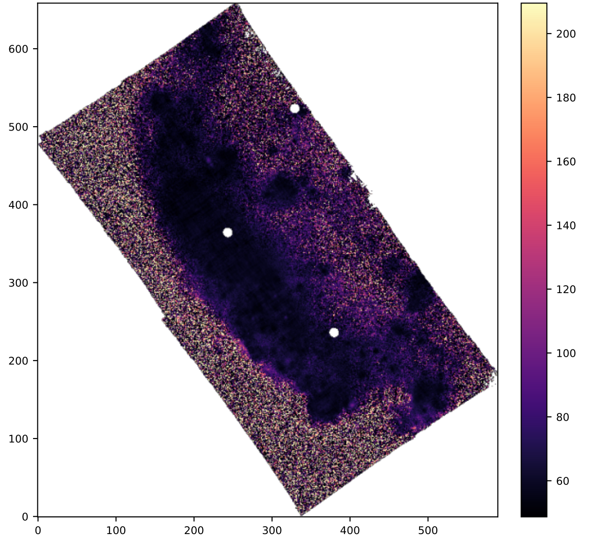
SPAXELS HA6562_SIGMA
