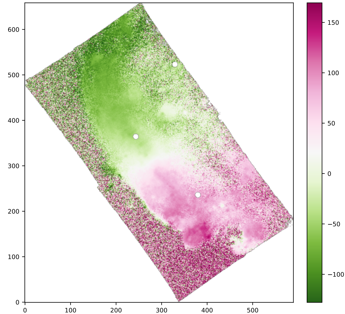
SPAXELS OI6300_VEL
