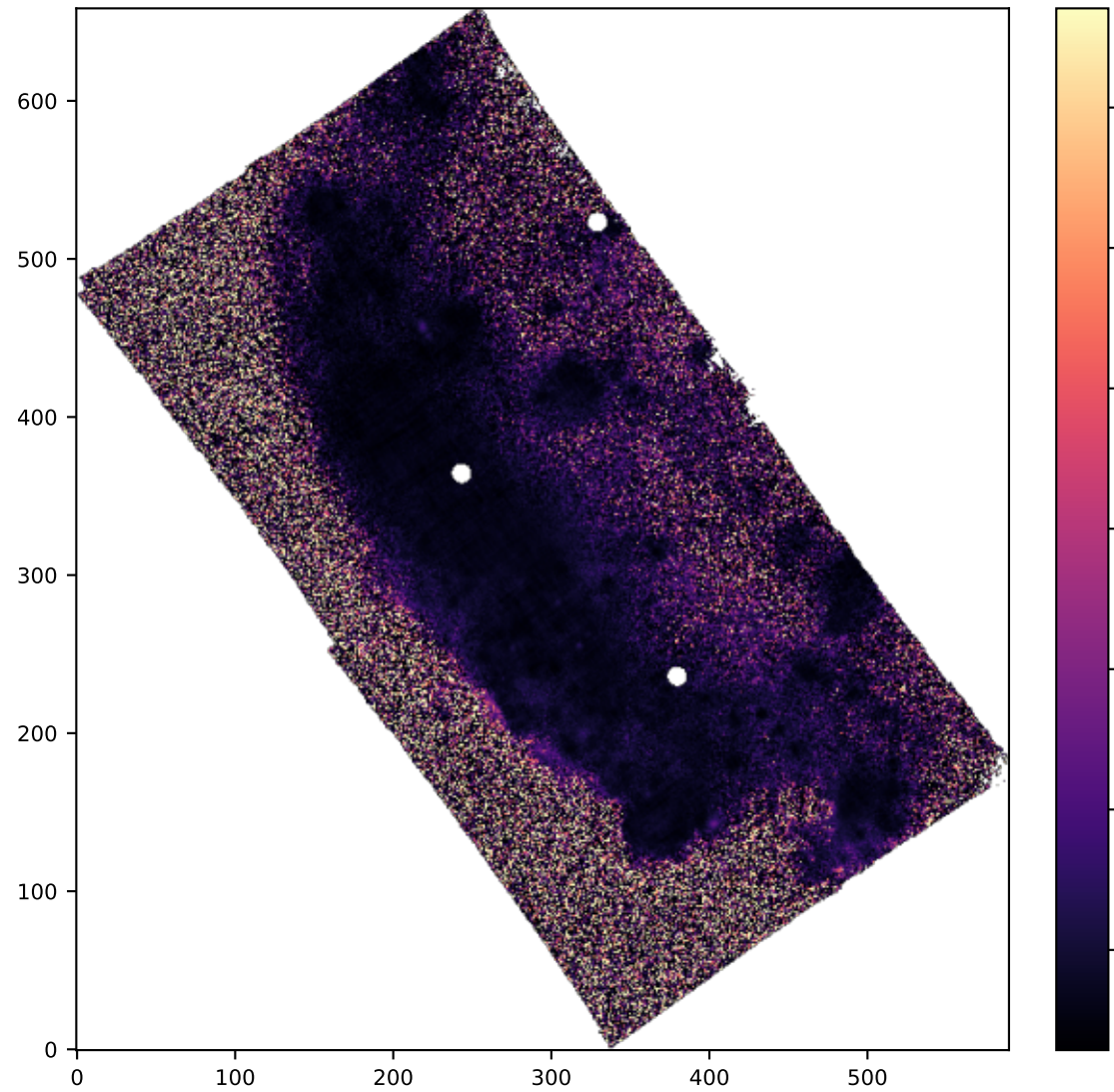
SPAXELS HB4861_SIGMA
