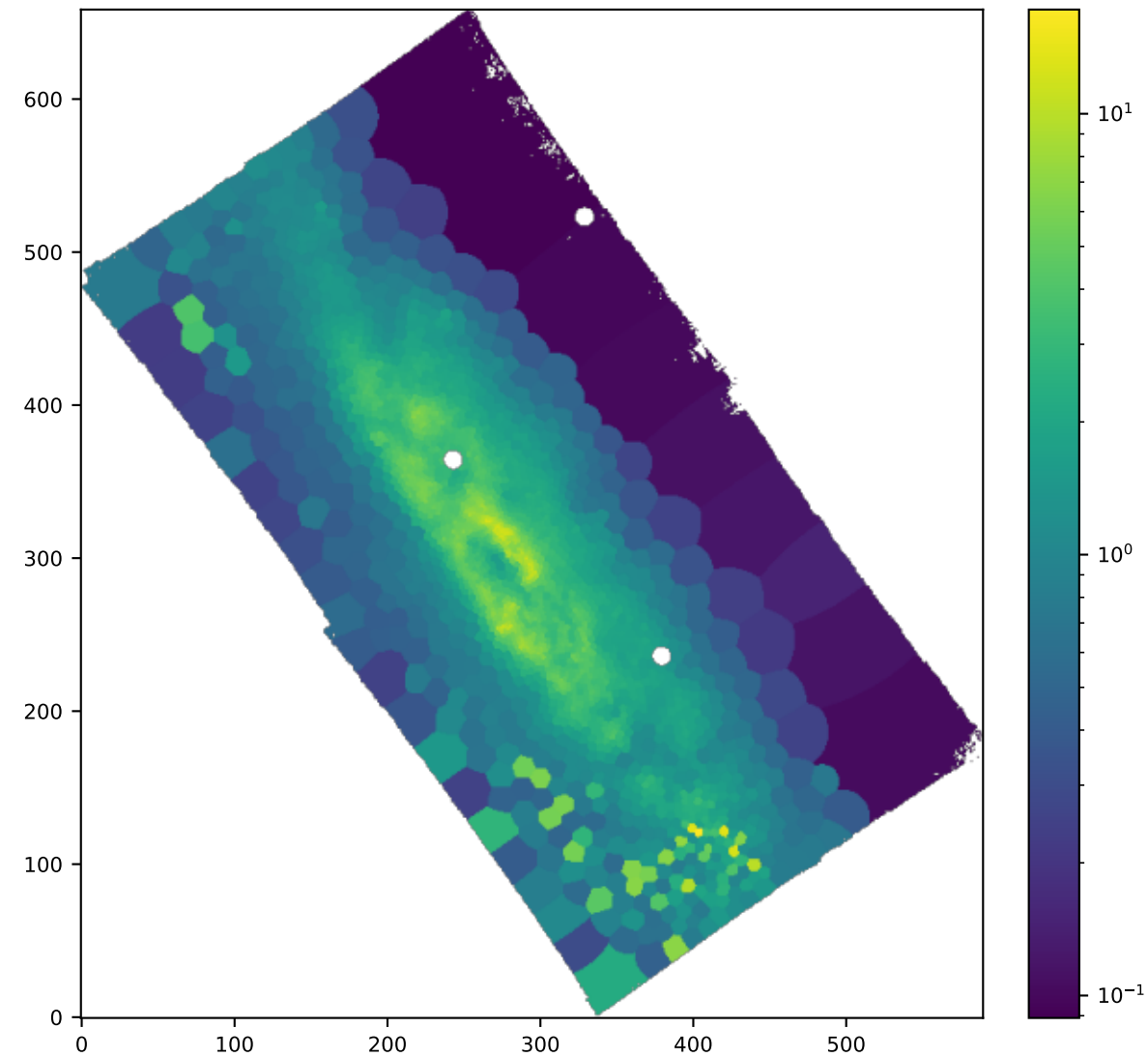
BIN SII6716_SIGMA_ERR
