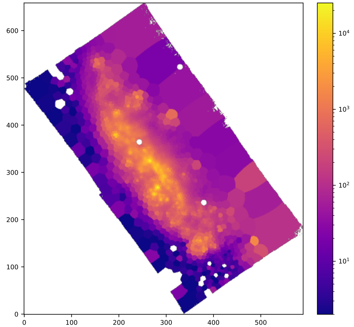
BIN HA6562_SIGMA
