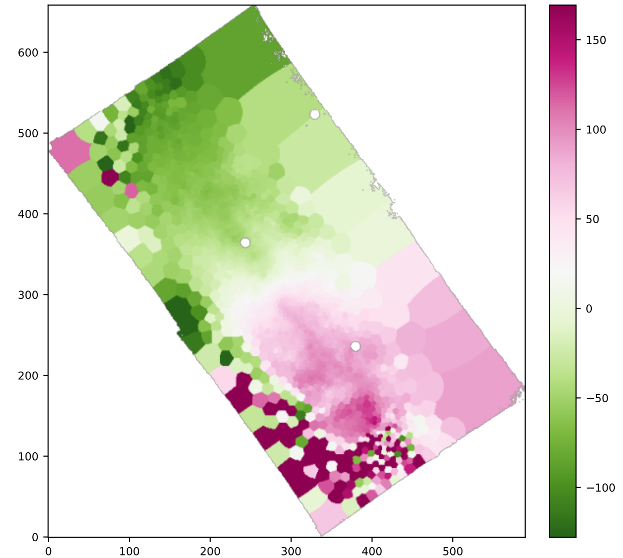
BIN SII6716_VEL
