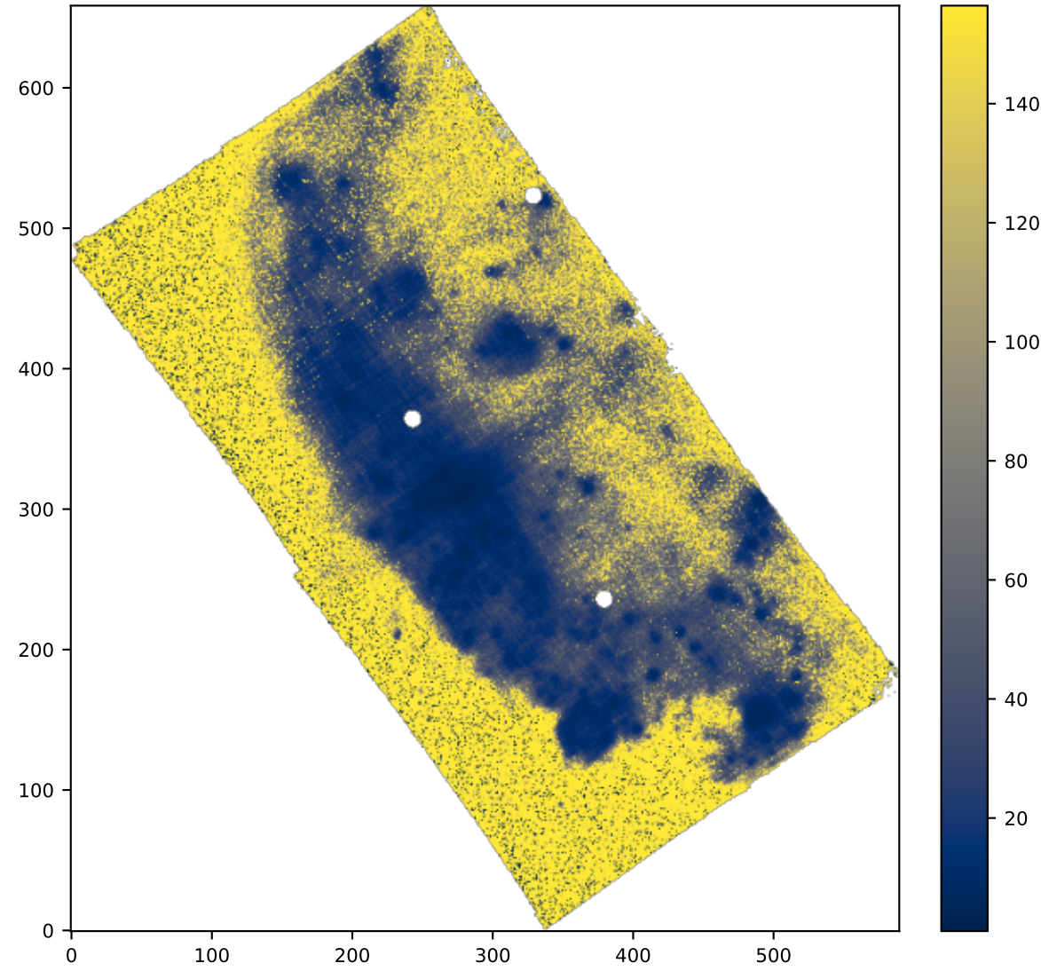
SPAXELS HA6562_SIGMA_ERR
