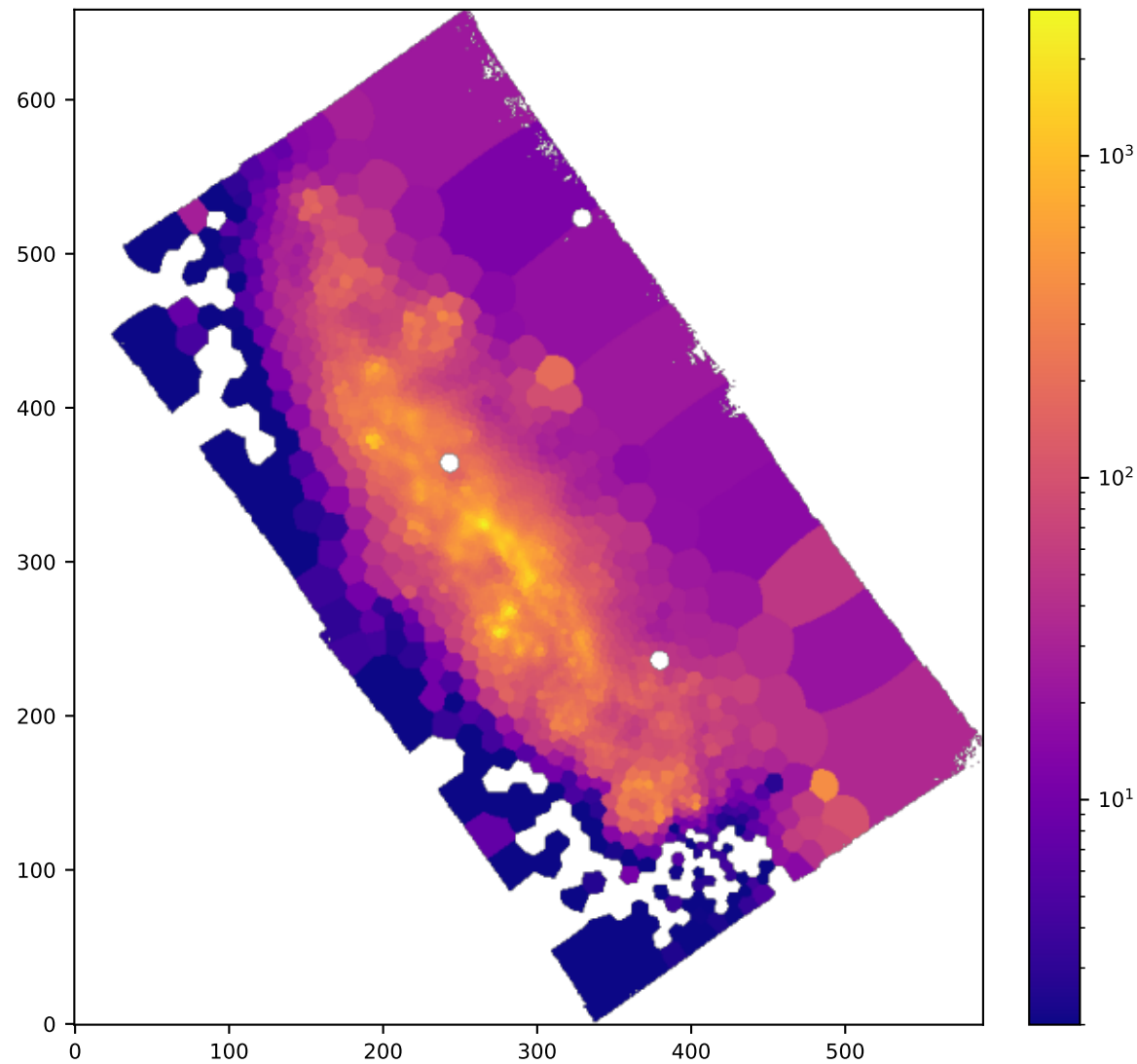
BIN SII6716_SIGMA
