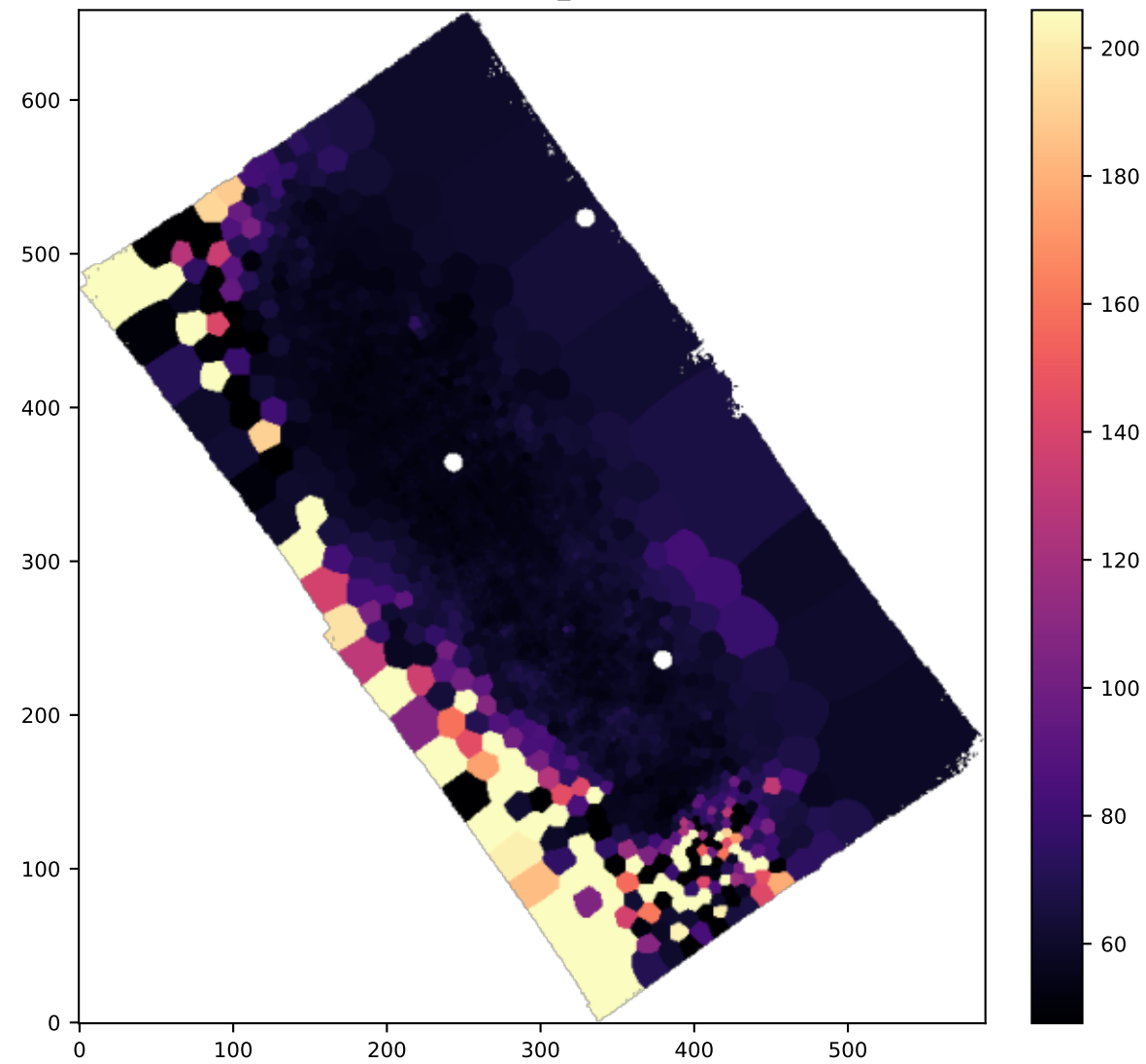
BIN SII6716_SIGMA
