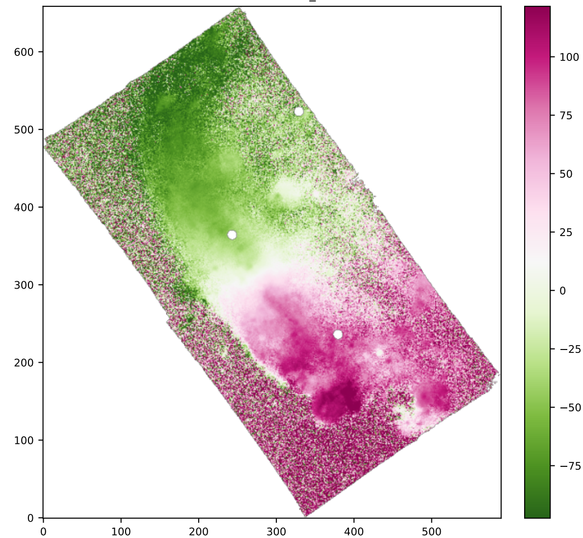
SPAXELS OI6363_VEL
