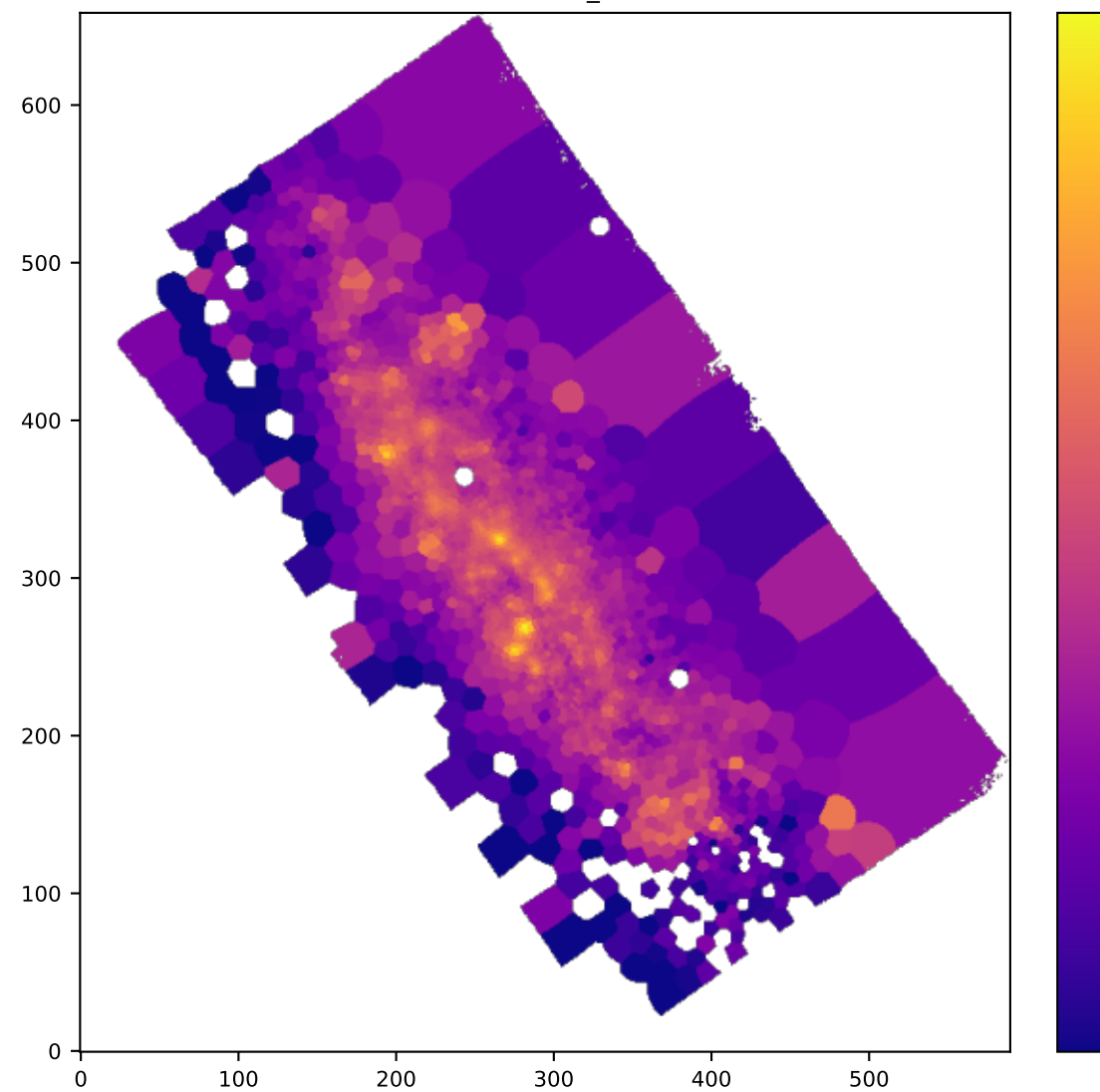
BIN OIII5006_SIGMA
