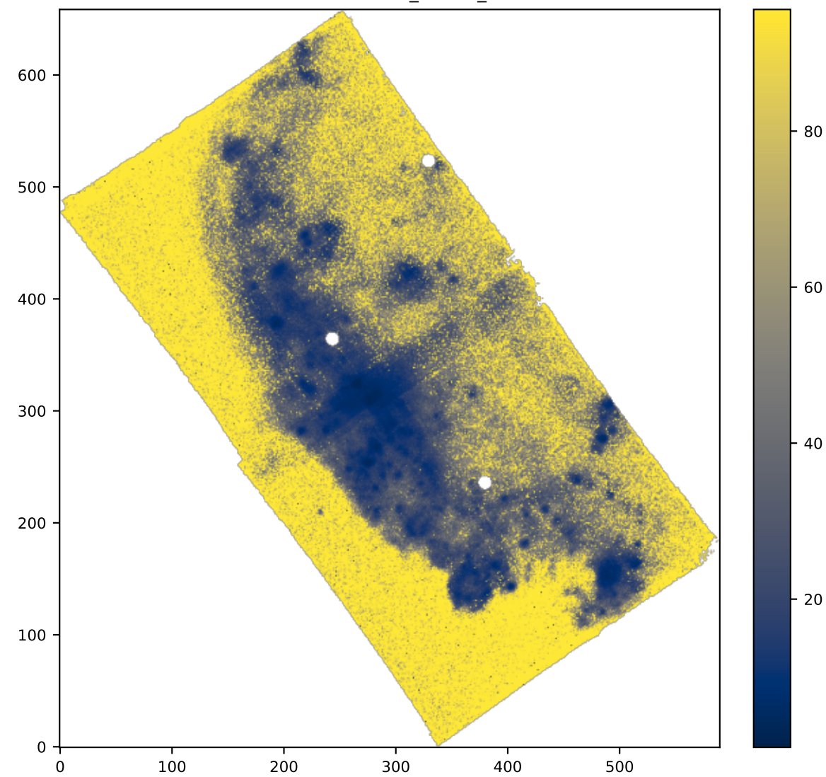
SPAXELS SII6716_SIGMA_ERR
