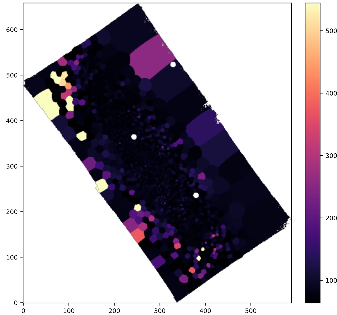
BIN OIII5006_SIGMA
