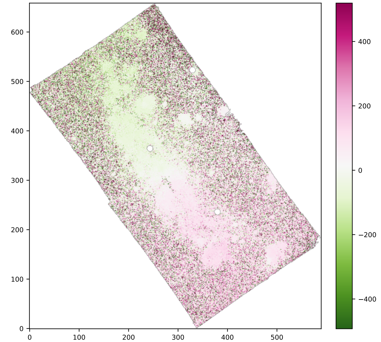
SPAXELS OIII5006_VEL
