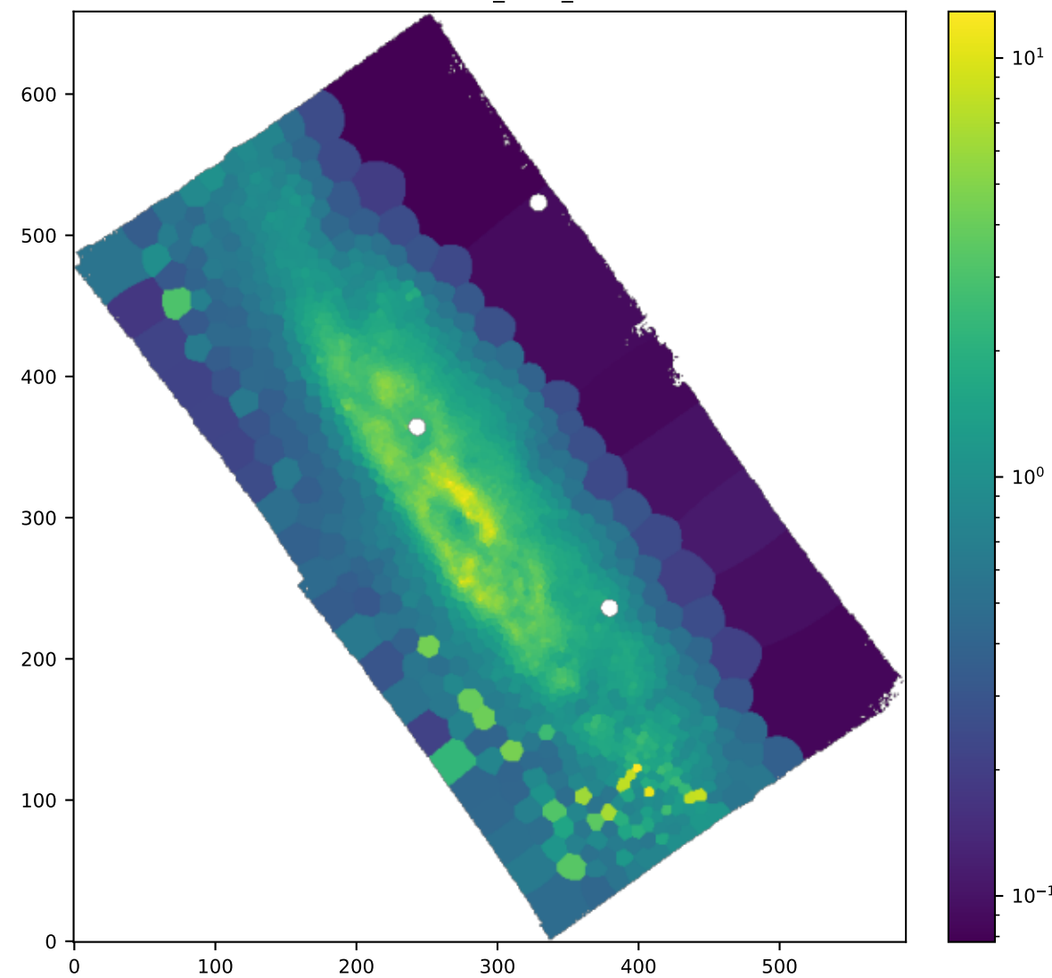
BIN SII6716_SIGMA_ERR
