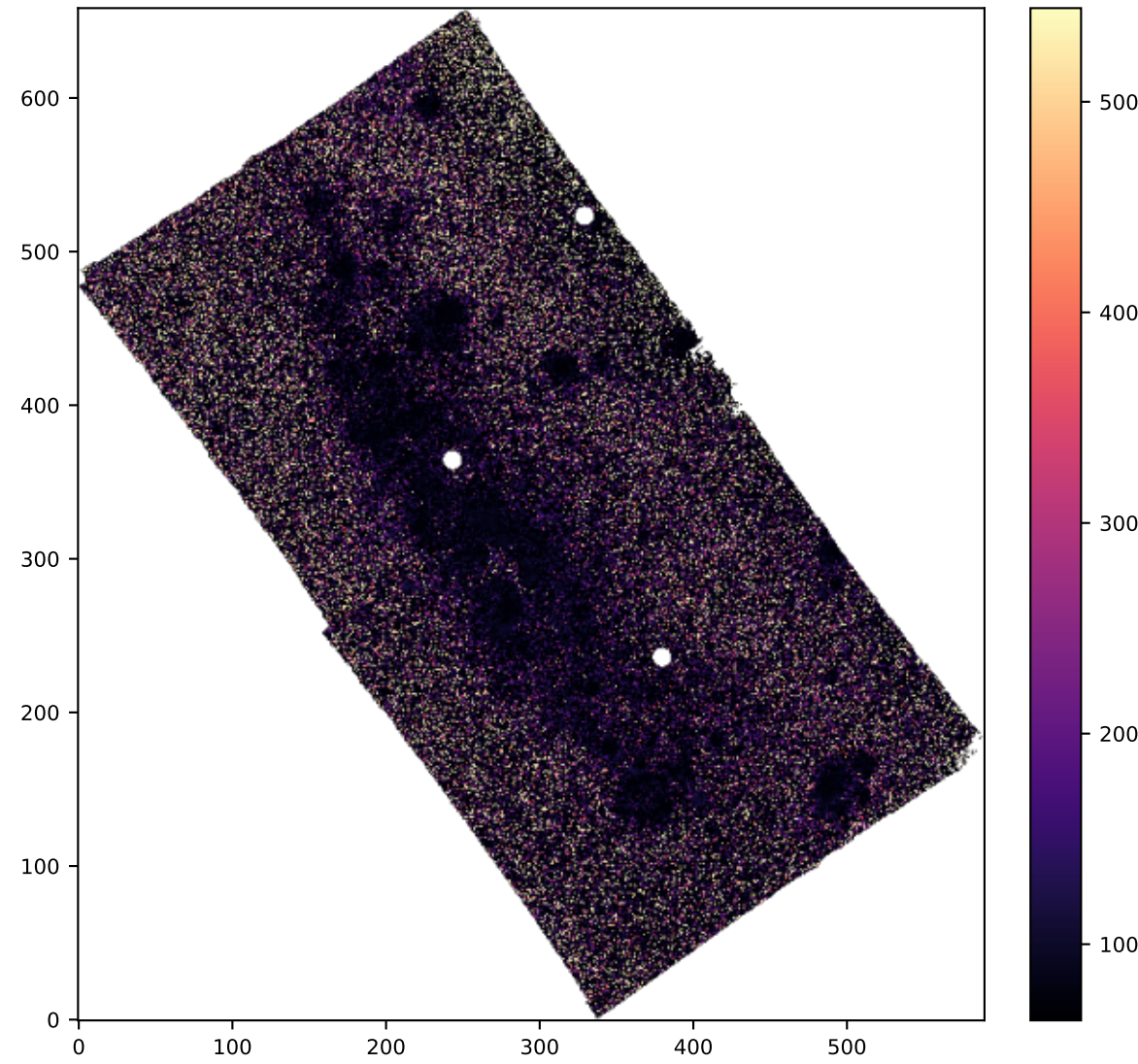
SPAXELS OIII5006_SIGMA
