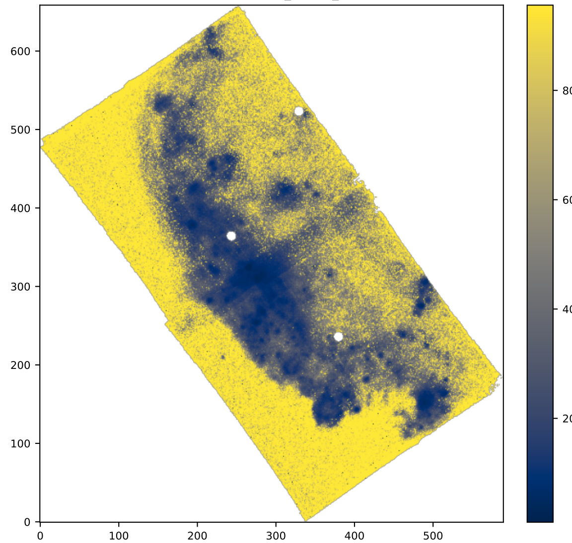
SPAXELS OI6363_SIGMA_ERR
