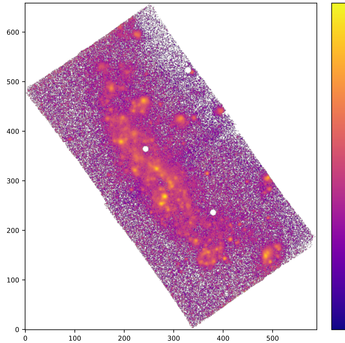
SPAXELS OIII5006_SIGMA
