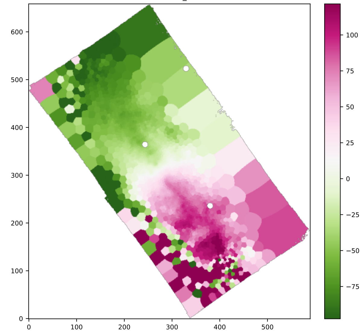
BIN SII6716_VEL
