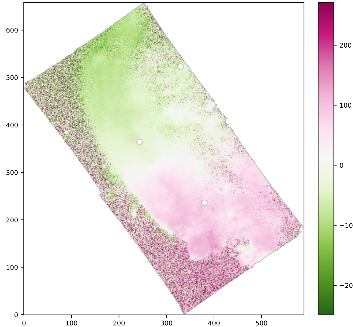
SPAXELS HB4861_VEL
