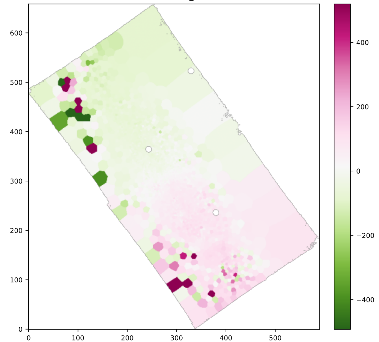
BIN OIII5006_VEL
