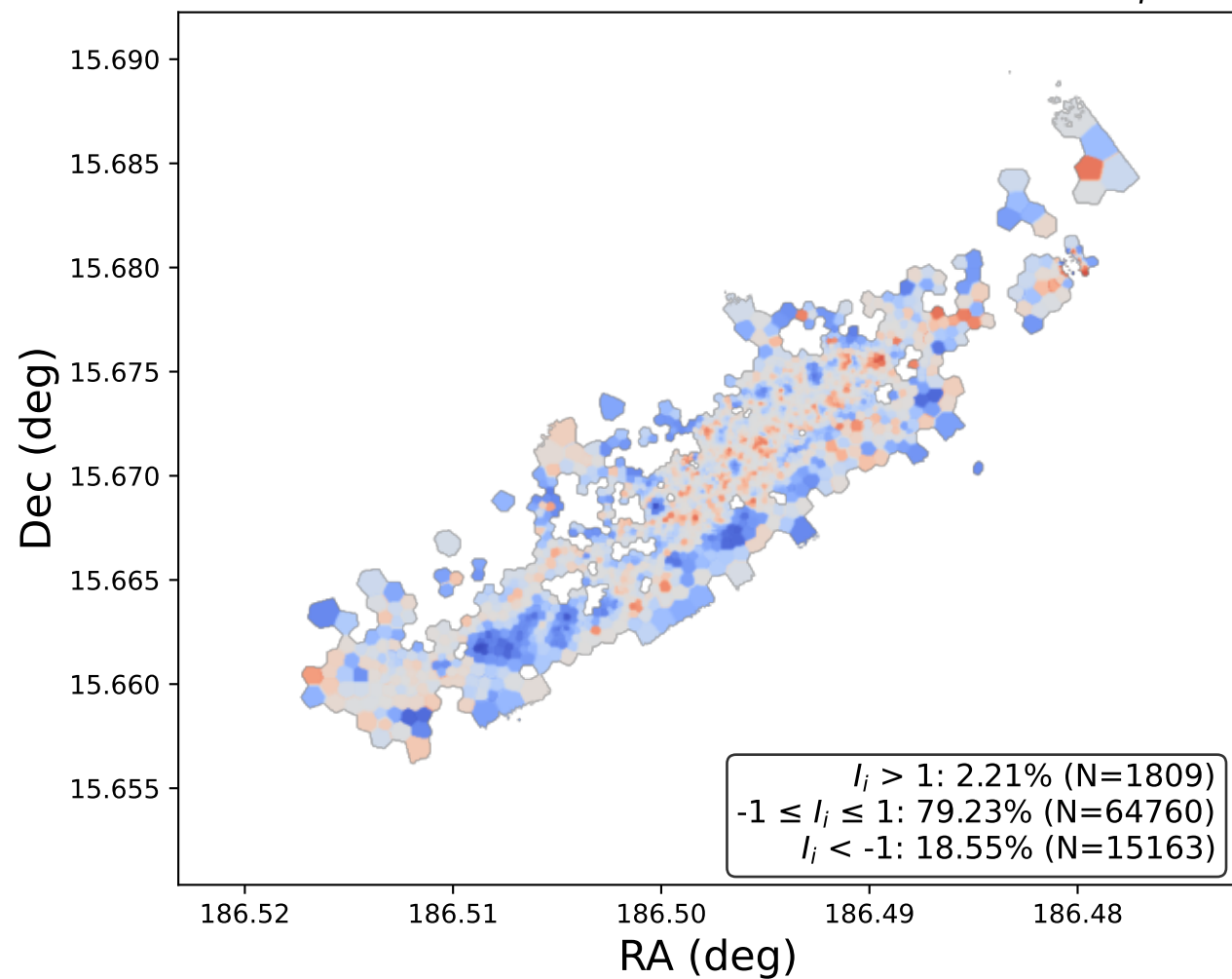
NGC4396: local bivariate Moran-like I_i
