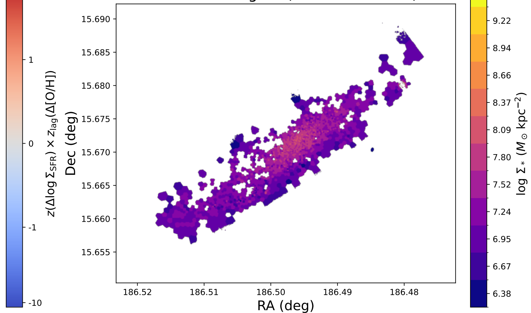
NGC4396: \log \Sigma_{*} (12 discrete bins)
