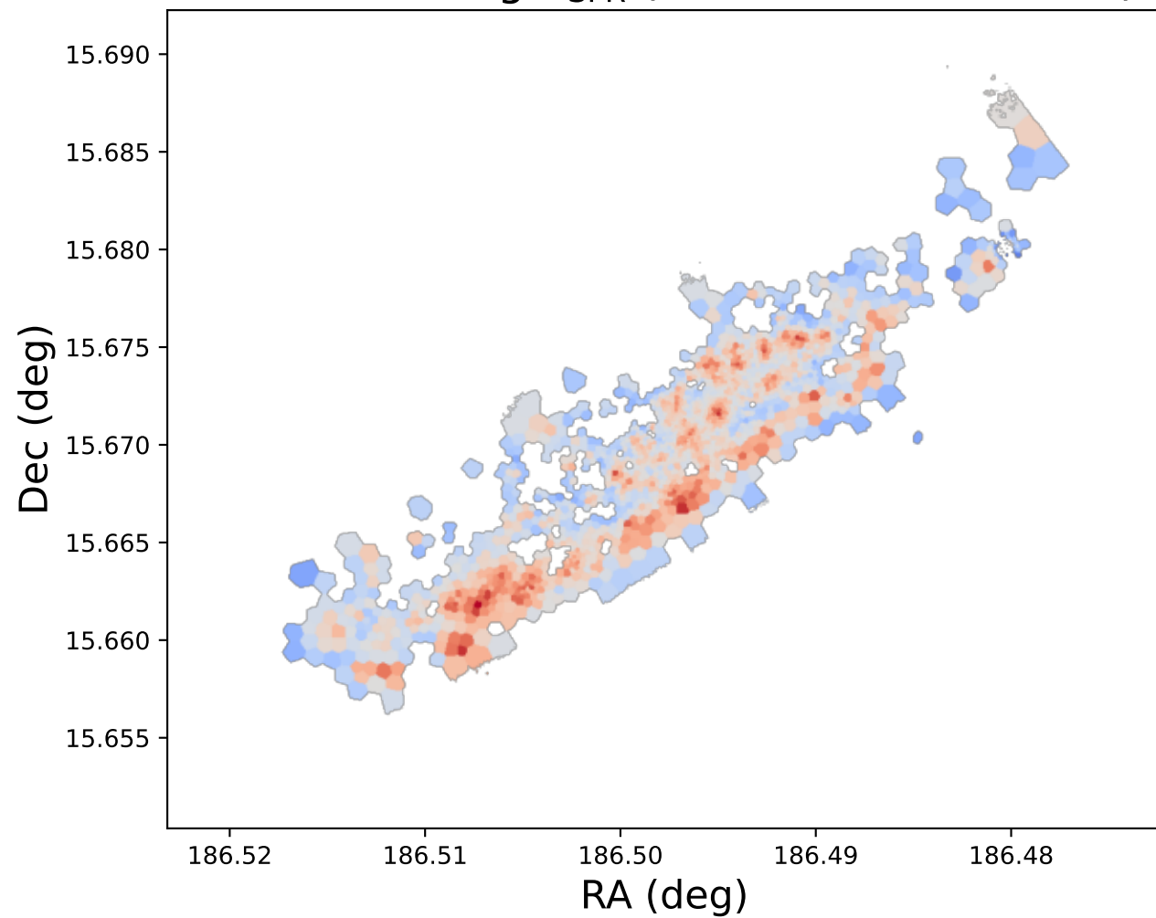
NGC4396: \Delta \log \Sigma_{\text{SFR}} (offset from bin mean)
