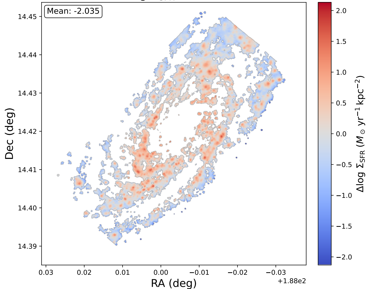
NGC4501: \Delta \log \Sigma_{\text{SFR}} (offset from mean)
