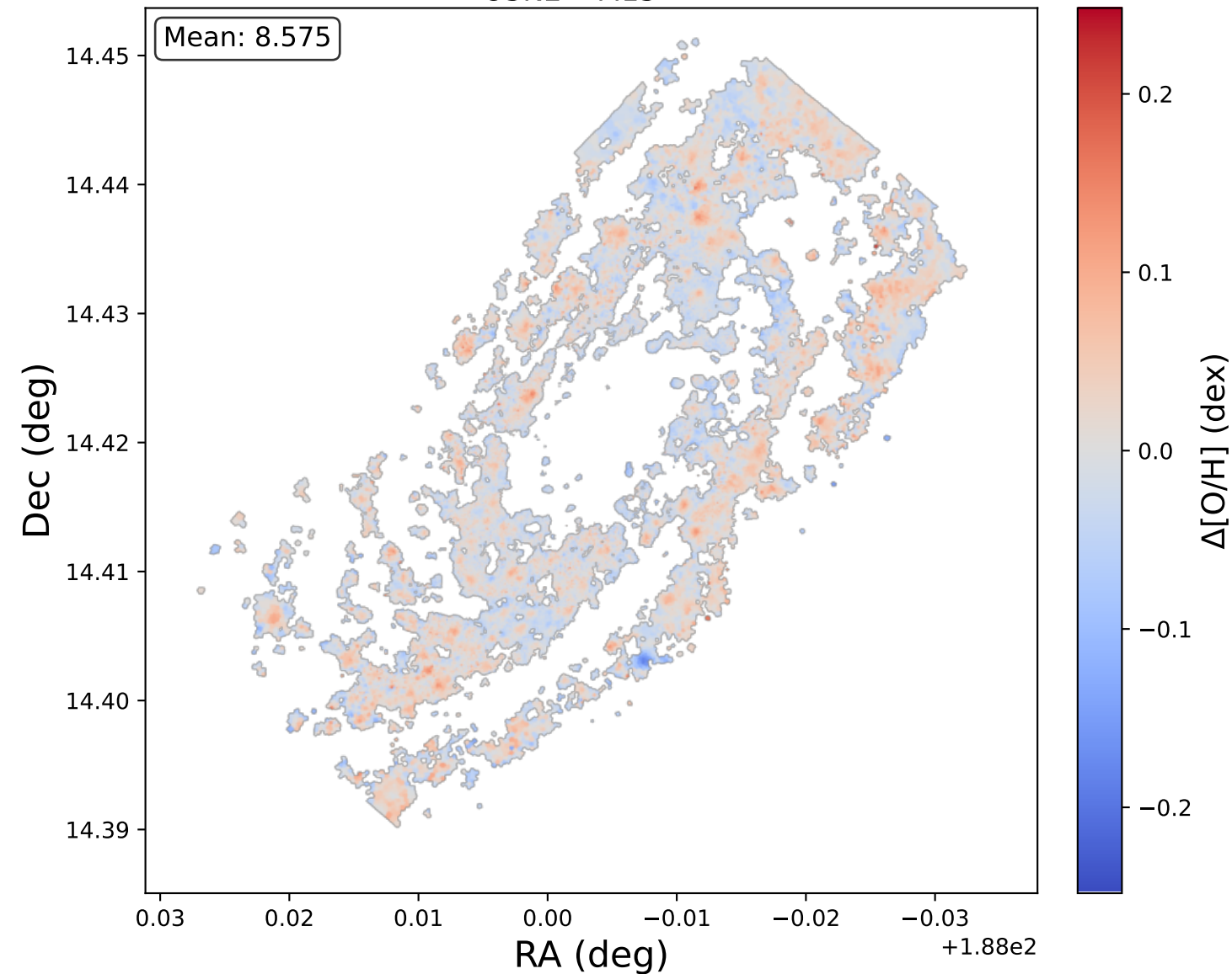
NGC4501: \Delta[\text{O}/\text{H}]_{\text{O3N2} - \text{M13}} (offset from mean)
