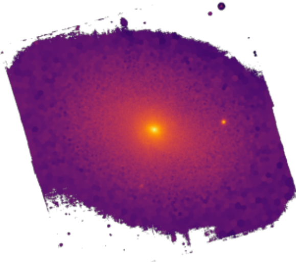
NGC4457
