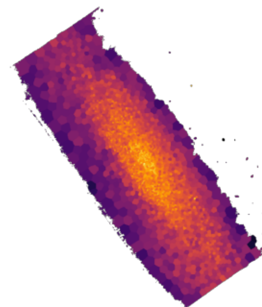
NGC4522
