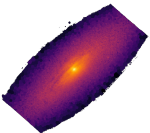
NGC4419
