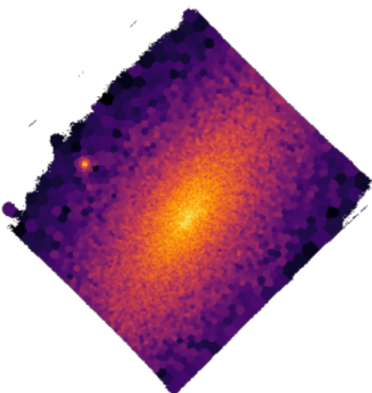
NGC4694
