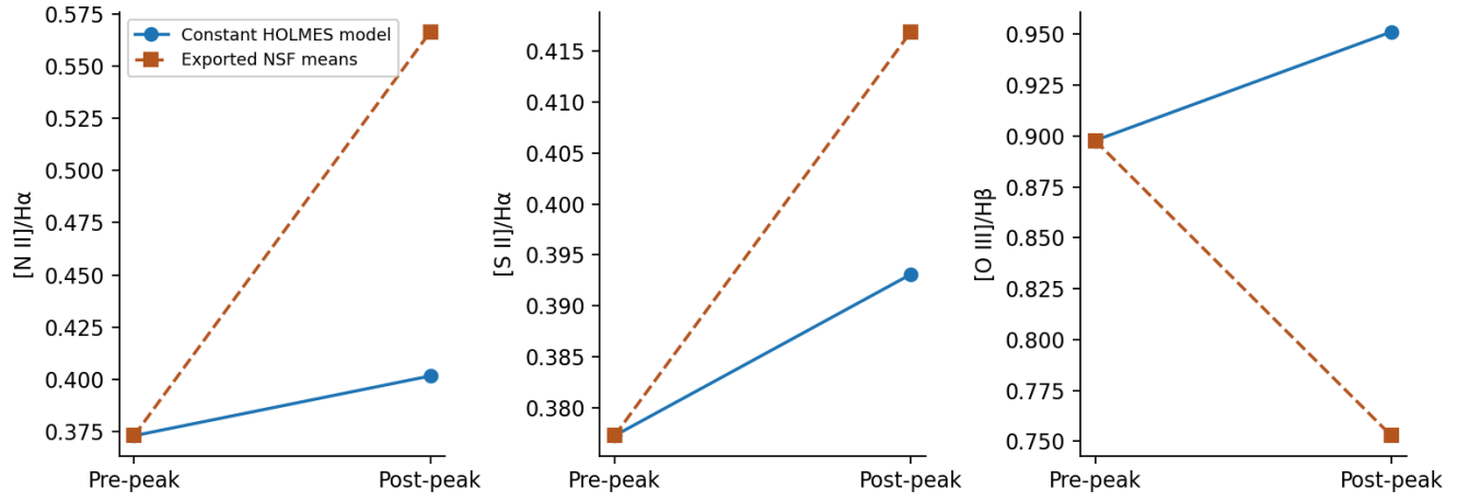
Figure 3. Conditional fixed-HOLMES predictions compared with the exported NSF mean ratios. The initial young ratio is calibrated to the pre-peak point. Post-peak Halpha luminosities are supplied from the data. The differences therefore test the constant-spectrum/photon-budget assumptions rather than the gas clock. Model 0 uses one common Halpha weight; the actual-Hbeta variant is in Appendix D. Lines connect different galaxy samples for comparison and do not imply observed temporal tracks.
