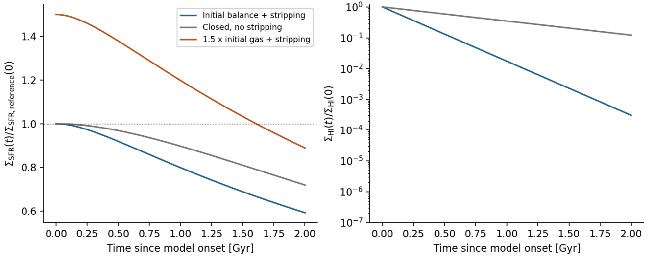
Figure 1. Model 0 at fixed conversion and depletion times. Left: SFR in units of the uncompressed initial reference; the orange curve begins with both gas columns multiplied by 1.5 and subsequently declines. Right: normalized atomic columns for the stripped and closed no-stripping cases. The orange atomic fraction coincides with the blue stripped fraction and is omitted. The elevated orange SFR is a spatial-level example, not a burst generated by switching on the HI sink.
