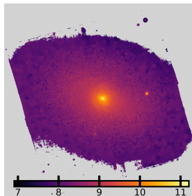
NGC4501: \log \Sigma_*
