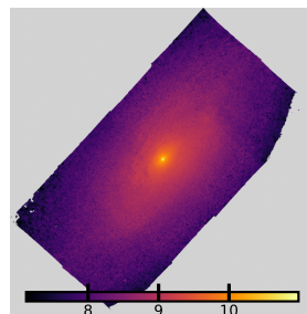
NGC4522: \log \Sigma_*
