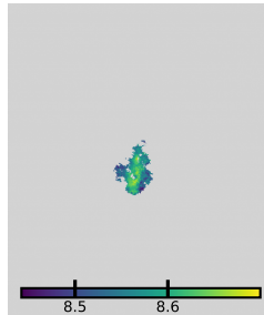
[O/H] (O3N2-M13, HII)
