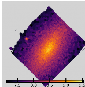
NGC4698: \log \Sigma_*
