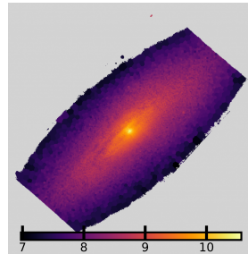
NGC4457: \log \Sigma_*
