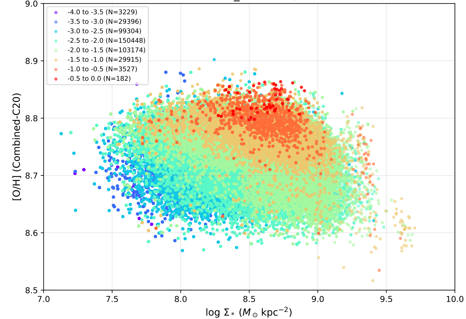
NGC4501 - rMZR in \Sigma_{\text{SFR}} bins (Combined-C20)
