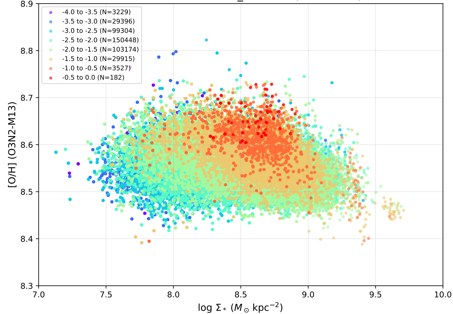
NGC4501 - rMZR in \Sigma_{\text{SFR}} bins (RS32-C20)
