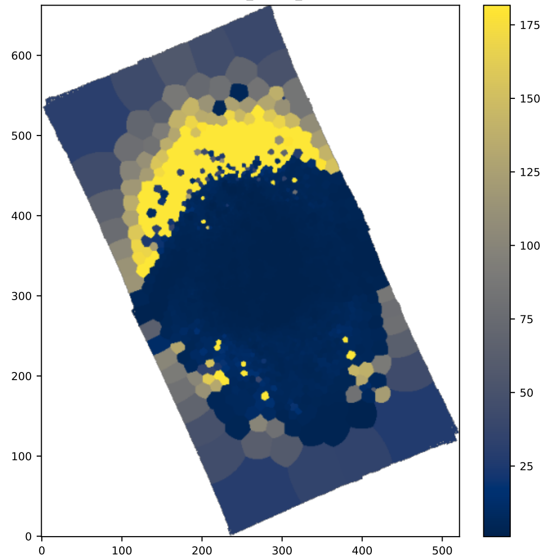
BIN OI6363_SIGMA_ERR
