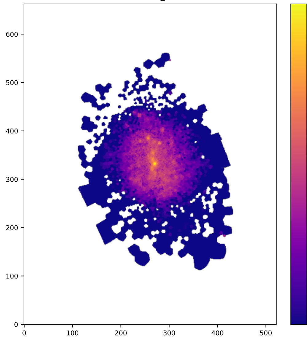
BIN OI6363_SIGMA
