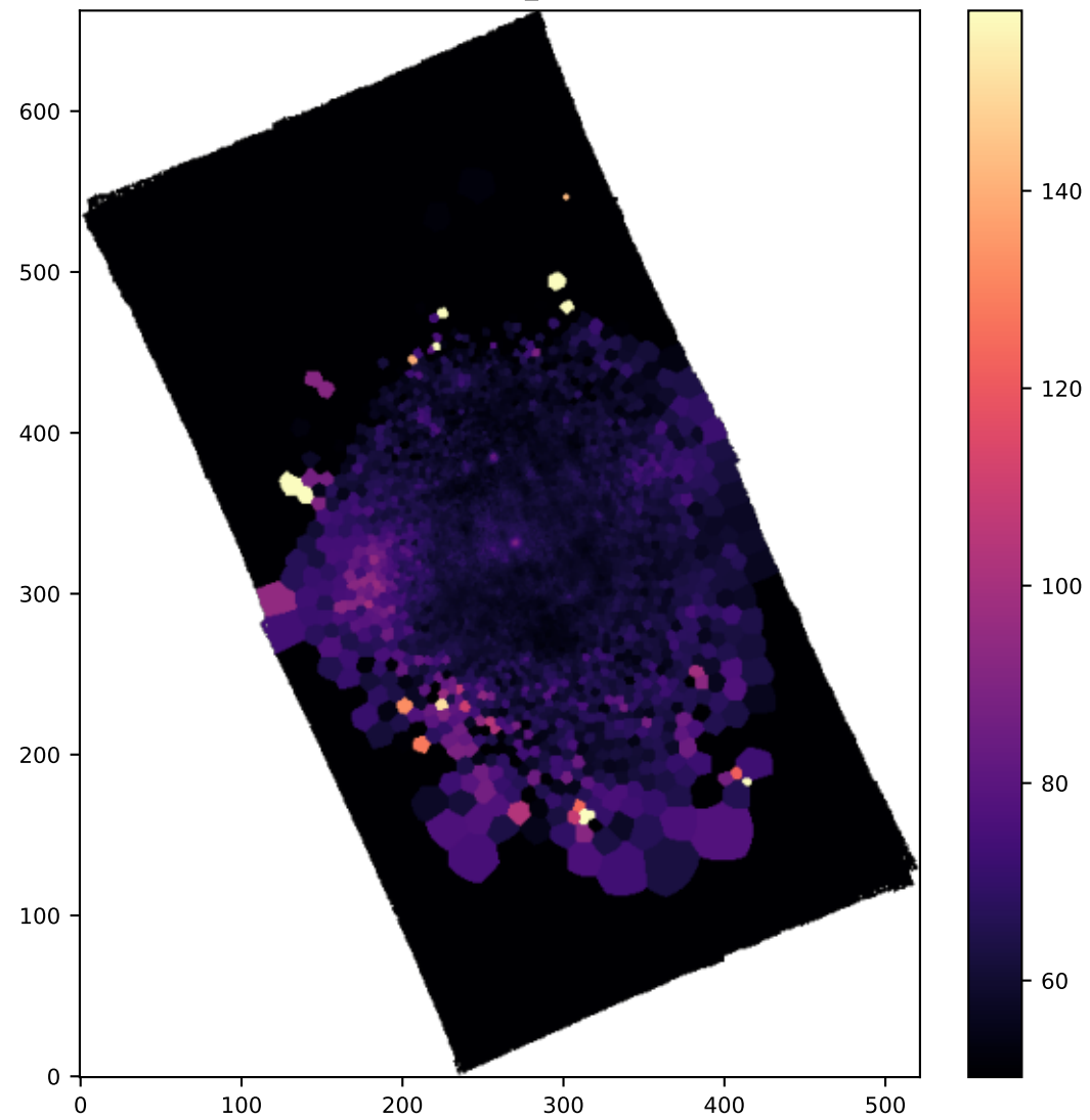
BIN OI6363_SIGMA
