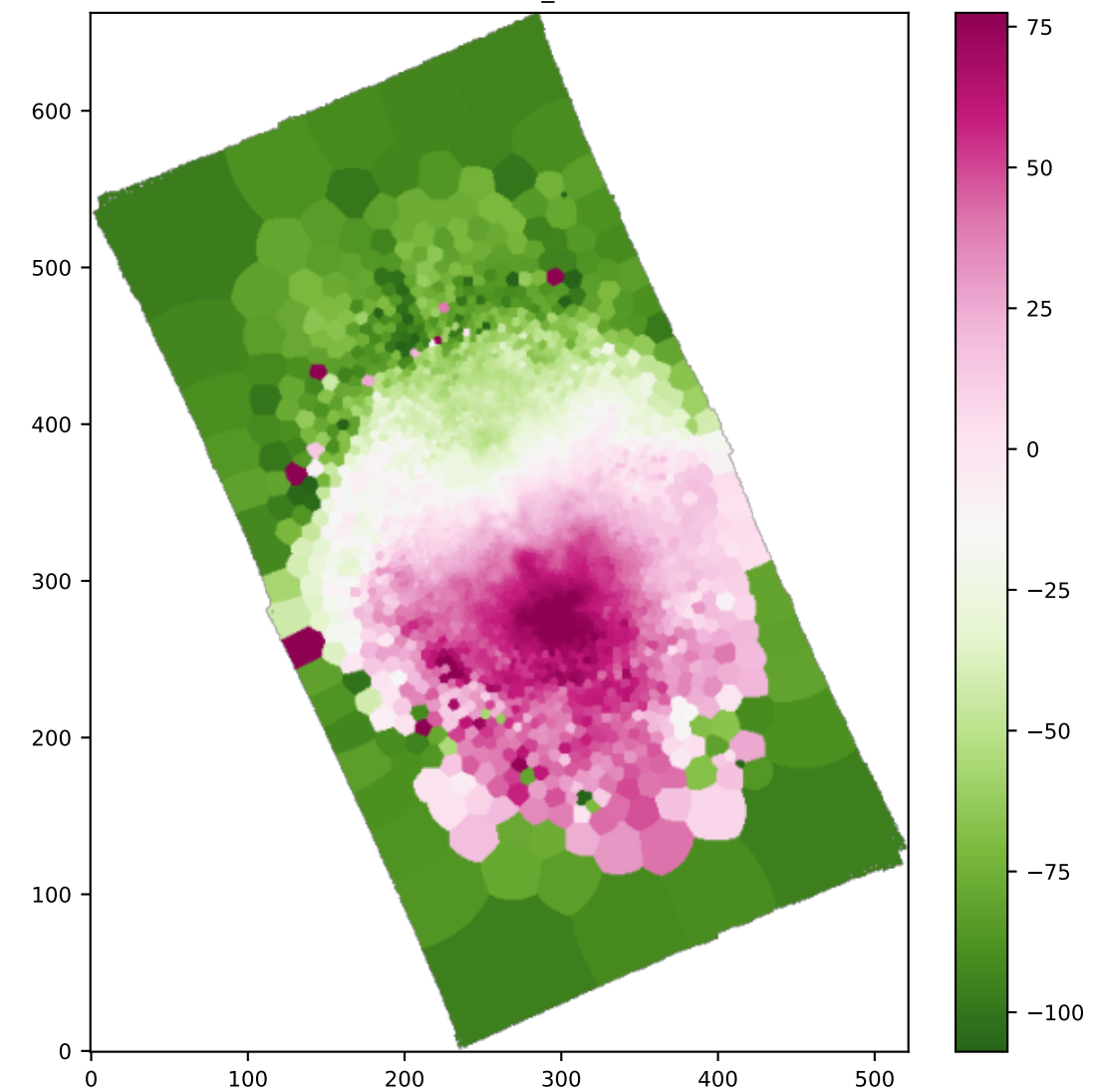
BIN OI6363_VEL
