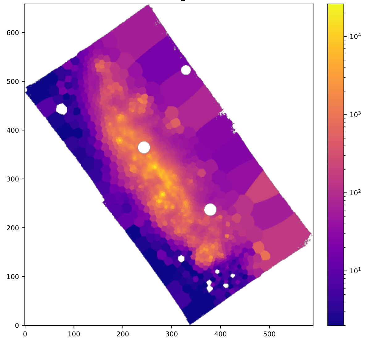
BIN HA6562_SIGMA
