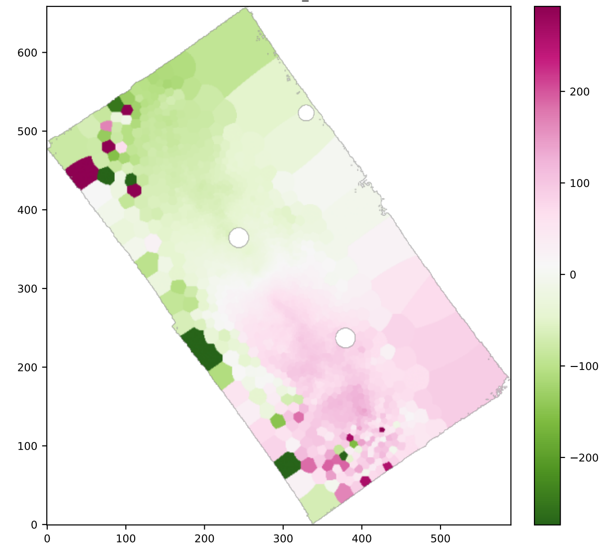
BIN HA6562_VEL
