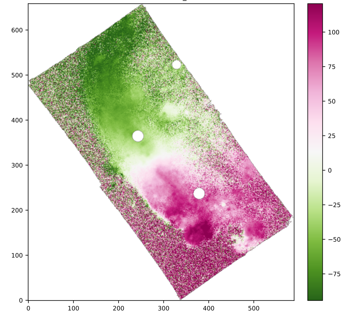
SPAXELS OI6300_VEL
