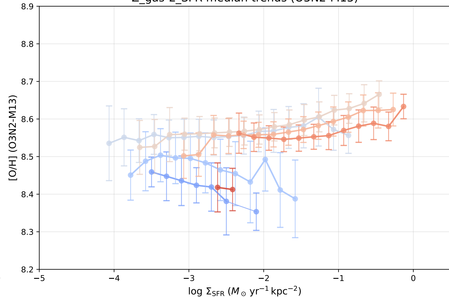
Z_gas- \Sigma_{\text{SFR}} median trends (O3N2-M13)
