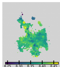
[O/H] (O3N2-M13, HII)
