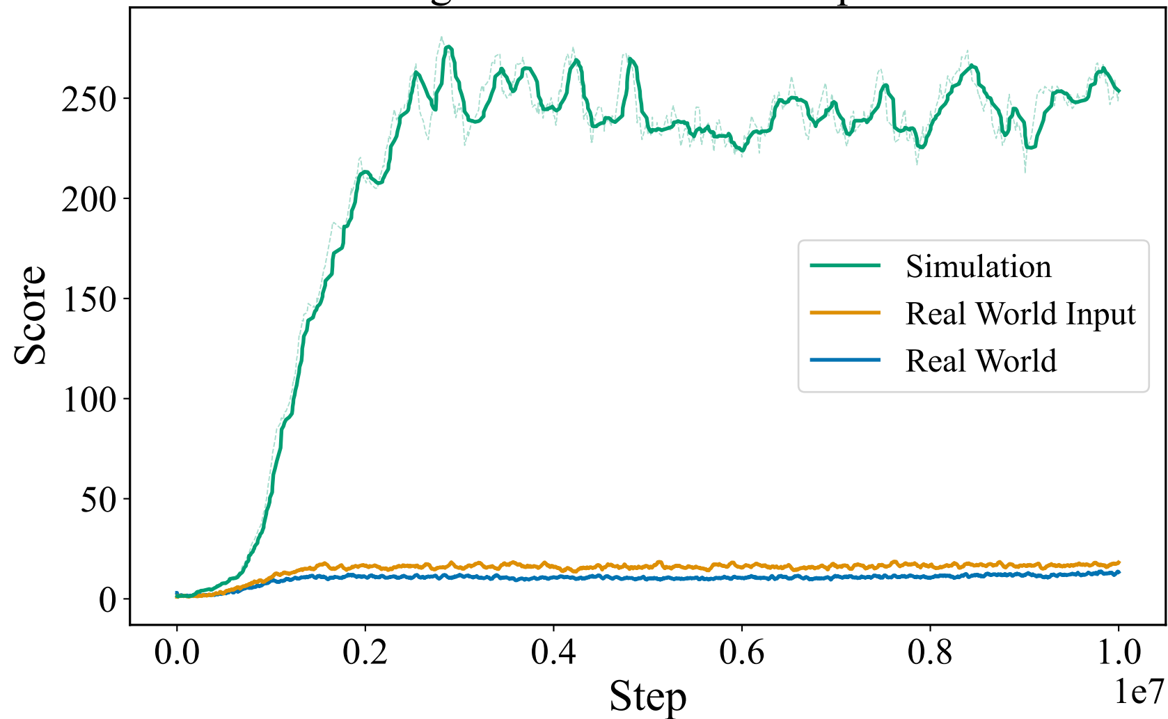
Average Score of Last 100 Episodes
