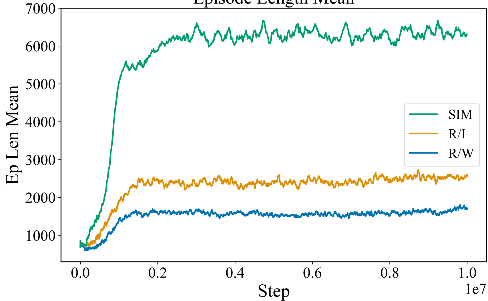
Episode Length Mean
