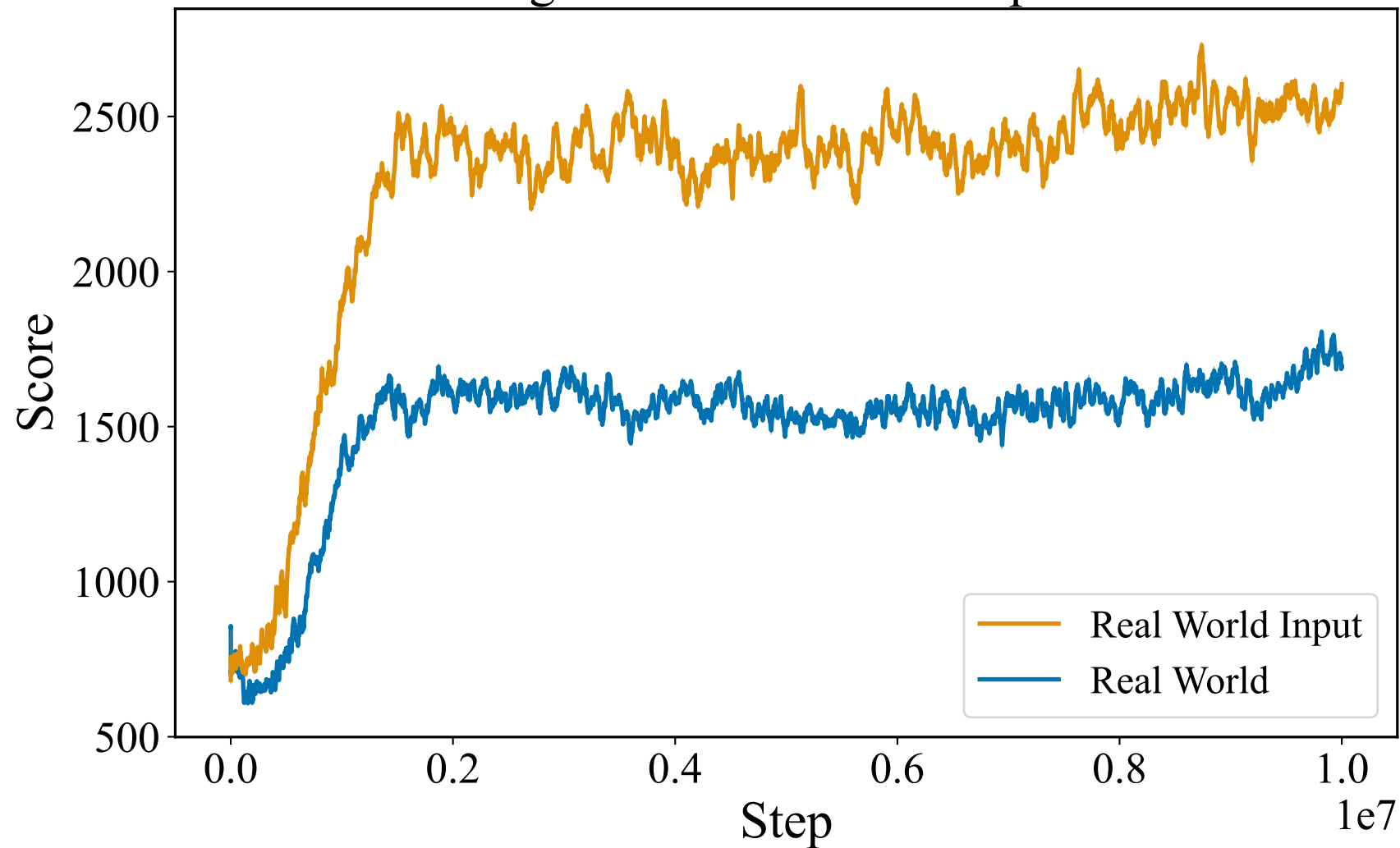
Average Score of Last 100 Episodes
