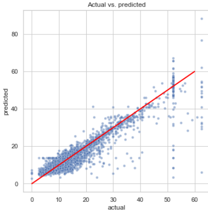
Fig. 3. Scatterplot of ‘predicted’ over ‘actual’
