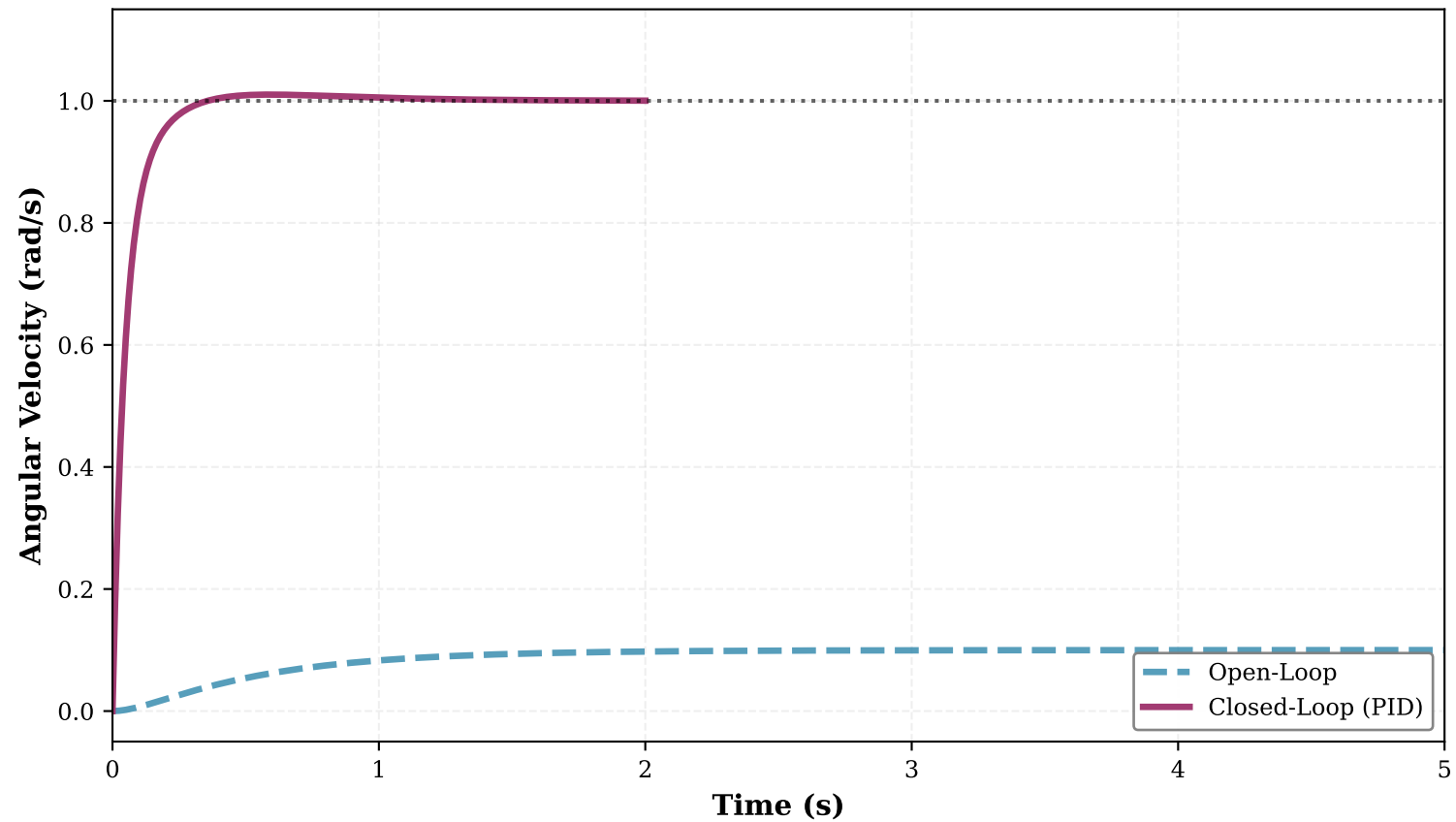
Step Response Comparison: Open-Loop vs Closed-Loop
